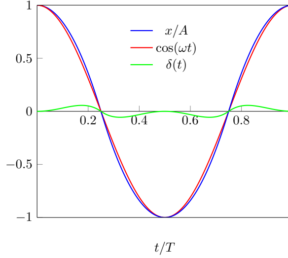
Figure 1. Graphs of the net displacement from Eq. (29), the unit-amplitude lowest-order Fourier component from Eq. (5), and the difference between them from Eq. (8).
