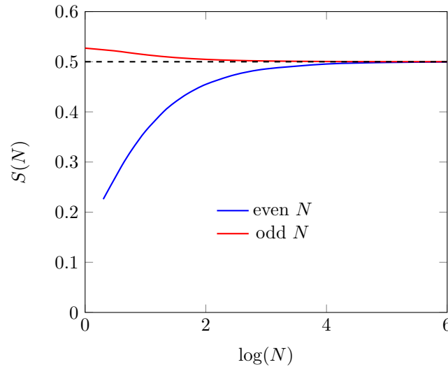
Figure 2. Graphs of the partial sums in Eq. (36), corresponding to k = 0 in Eq. (35), for values of N ranging from one to a million. The sums approach \frac{1}{2} from above for odd values of N and from below for even values of N . Similar behavior is observed for positive even values of k . For positive odd values of k , the partial sums for odd values of N approach \frac{1}{2} from below, while the sums for even values of N approach it from above. For negative integer values of k , the partial sums approach -\frac{1}{2} instead.
