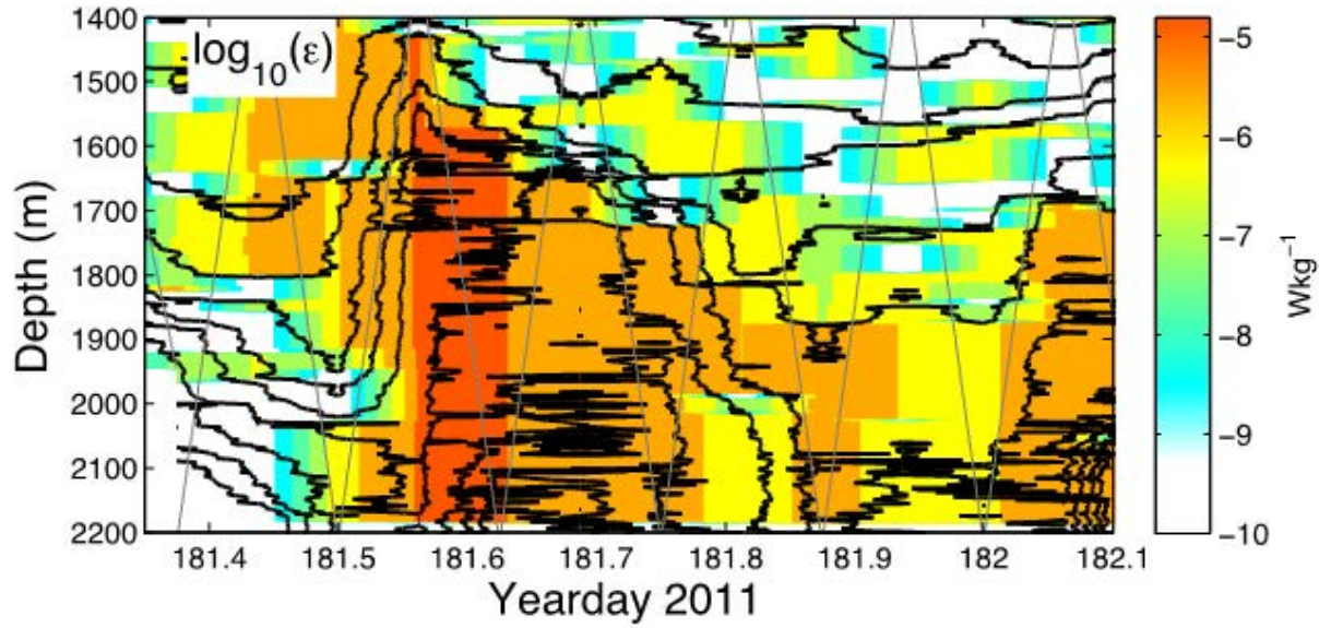
Figure 6: Turbulent dissipation rate (color) inferred from density overturns at mooring S9. Black lines are isopycnals. Gray lines show the sawtooth sampling pattern of the moored profiler.
