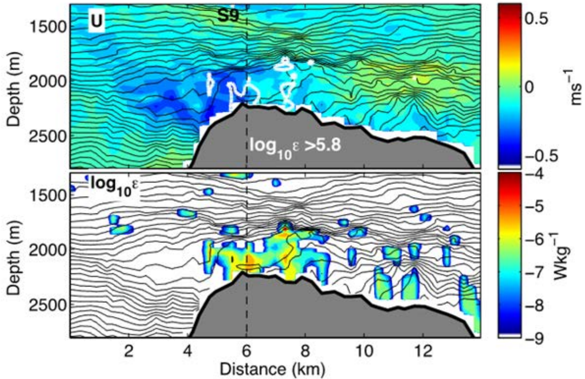
Figure 7: Snapshot from MITgcm model transect through mooring S9. (Top) zonal velocity and isotherms. Regions of high turbulent dissipation rate are contoured in white. (Lower) Turbulent dissipation rate (color) and isotherms.
