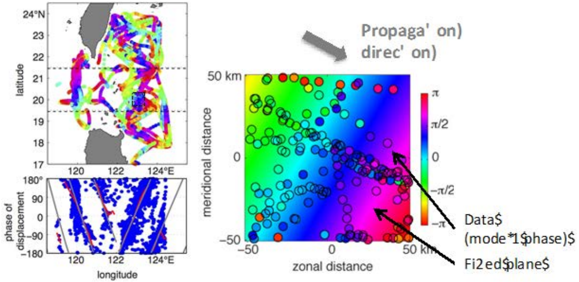
Figure 10: Top left: Phase of the semidiurnal internal tide at 500 m as a function of location. Estimates in Luzon Strait (between 19.5° and 21.5° are plotted as function of longitude in the bottom panel, showing progression equal to the mode-1 phase speed (gray lines). The direction of propagation can be estimated by looking at the spatial variations of the phase.
