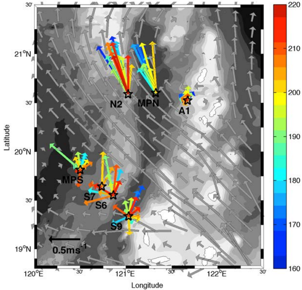
Figure 8: Low-passed velocity from moored ADCP's, averaged over the upper 150m. Vector colors indicate time (yearday 2011). Gray arrows are velocity at 150m from NRL EASNFS model provided by Dr.Ko, averaged over the duration of the mooring deployment. Note the strong and relatively constant northward flow over the western half of the northern line. Velocity scale is shown at lower left.
