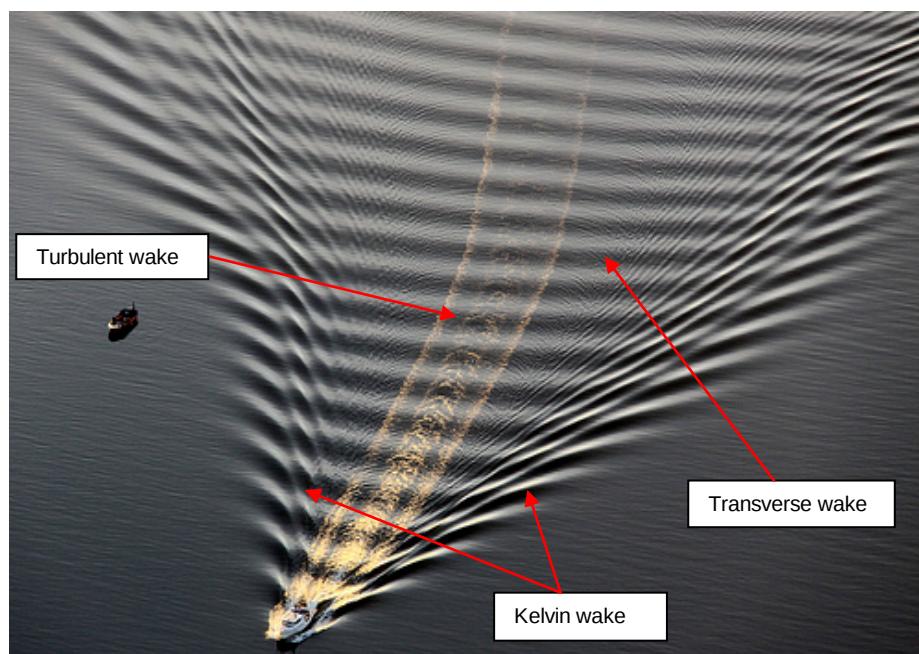
Figure 1: Optical image of a ship wake showing the different wave patterns produced by a ship. The bow wave is oriented at the Mach angle of 19^{\circ} 28' and the transverse wake are circular waves emanating from the ship's stern. © 2009 Chris Goldberg used by permission.
