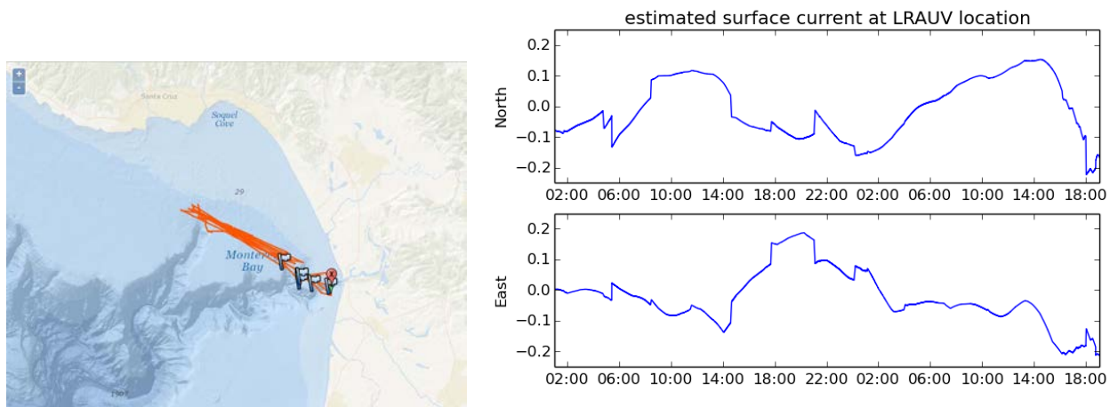
Figure 1: Field trial using onboard emulator to estimate surface current at LRAUV location. Left panel shows vehicle track and right panel shows estimated surface currents over time.
