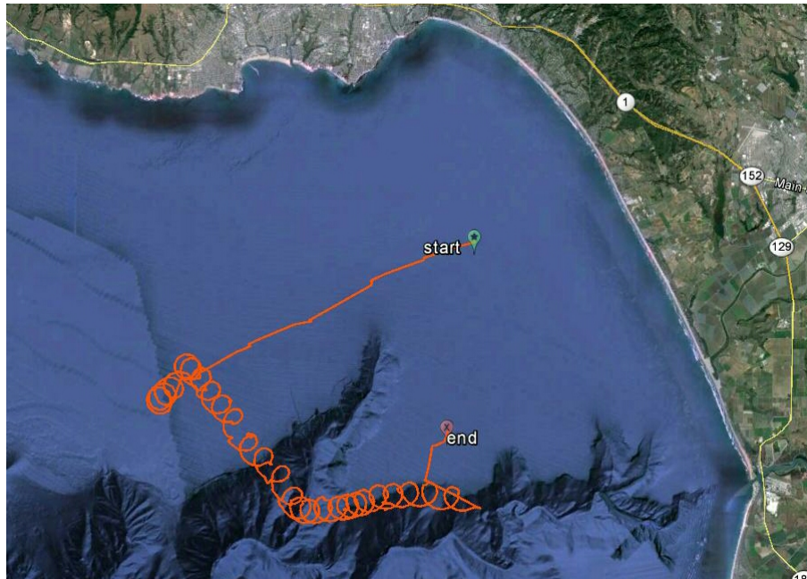
Figure 2: Path taken by LRAUV Daphne as she circled a virtual surface drifter in Monterey Bay. The drifter track was calculated from surface currents predicted hourly by the onboard compact model, interpolated in time and space using the method mentioned in work completed point 1.g.
