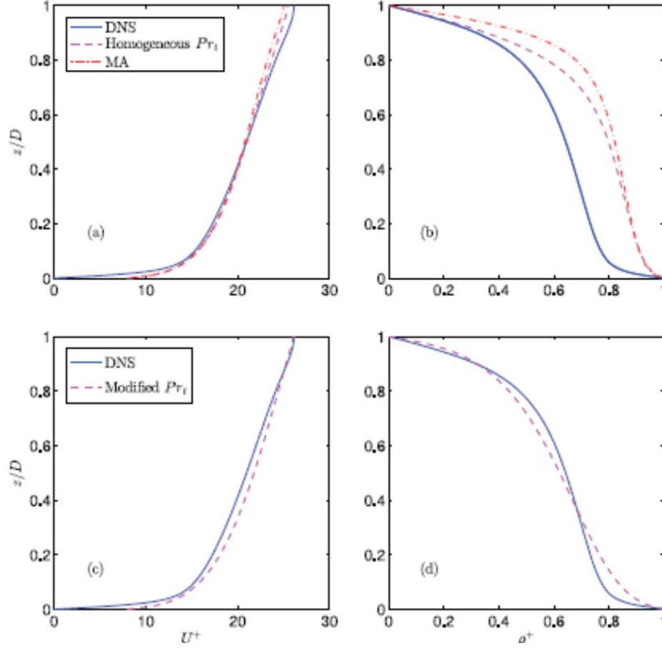
Figure 1: (left) Velocity profiles and (right) density profiles for Ri_\tau = 60 obtained from the zero-equation closure scheme using (a, b) the Prt formulations given by equation (2) and the formulation of Munk and Anderson (1948) and (c, d) the modified Prt formulation (equation (1)) compared with the channel flow DNS data of Garcia-Villalba and del Alamo (2011).
