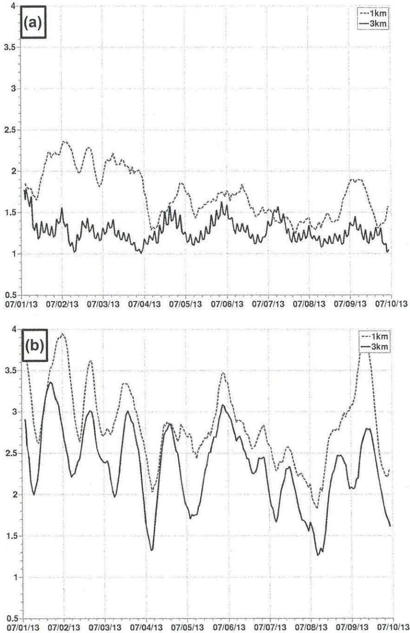
FIGURE 7 A comparison of the J_{FIT} values from the analyses (a) and the first guesses (b) from the 1-km (dashed) and 3-km (solid) model resolutions.
