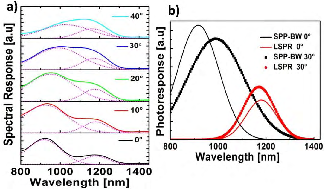
Figure 14: a) Measured angular photoresponse spectra of PENPD showing enhanced photocurrent due to both SPP-BW (0,1) and LSPR modes. P = 580 nm w = 160 nm h = 320 nm b) Fitting of the SPP-BW and LSPR before and after overlap at 0^\circ and 30^\circ
