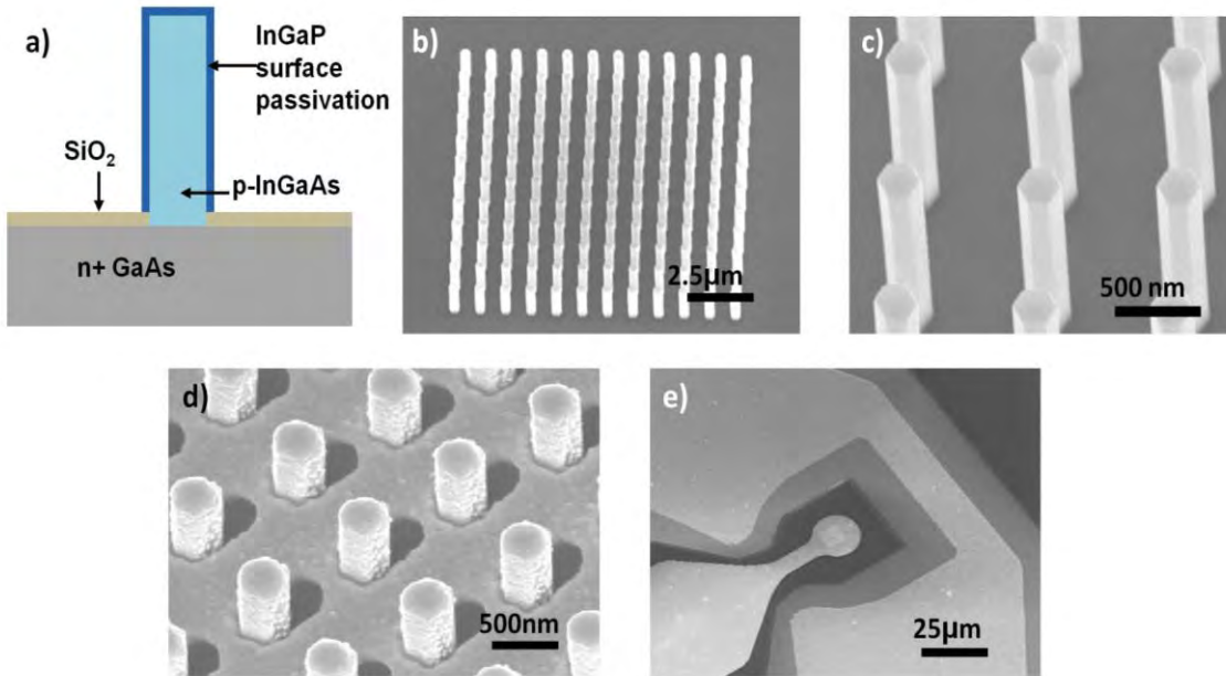
Figure 22: a) Schematic of nanopillar structure investigated for 1 micron nanopillar APD b) SEM of 10\ \mu\text{m} \times 10\ \mu\text{m} array c) Close up view of InGaAs nanopillar passivated with InGaP d) Close up SEM of final device showing plasmonic metal hole array antenna e) Nanopillar array integrated with GSG contact pads
