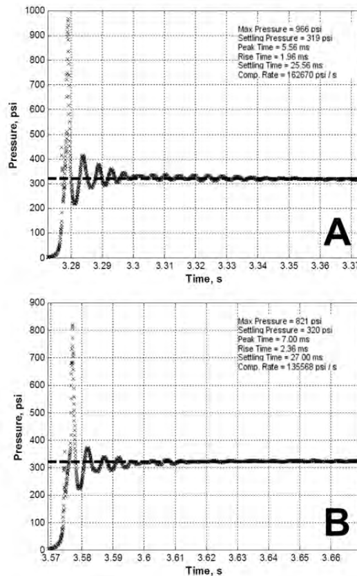
Figure 3. Representative pressure trace of a) water and b) AF-M315E at 300 psi and 25 °C.
