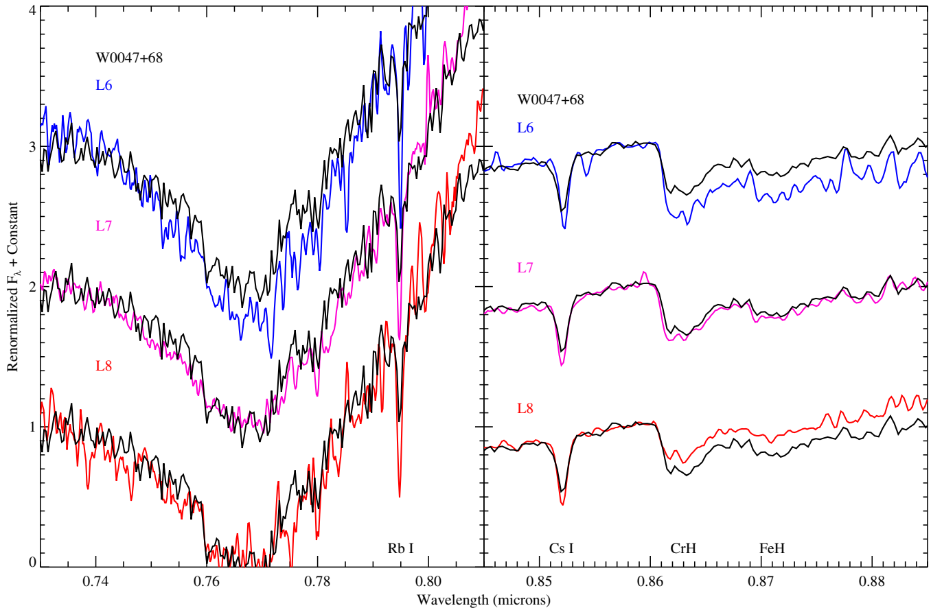
Figure 4. Optical MMT spectrum of W0047+68 (black) compared to the Kirkpatrick et al. (1999) spectra of L6, L7, and L8 standards in the K I doublet region and the CrH/FeH region; on the left, the spectra are normalized by the mean value in the range of 0.72–0.81 \mu\text{m} and on the right, 0.855–0.860 \mu\text{m} . W0047+68 best resembles the L7 standard, but the Rb I and Cs I lines are both weaker than expected. Note that the W0047+68 MMT spectrum shown here was taken with a different telescope and instrument, but we have smoothed the data to match resolutions.
