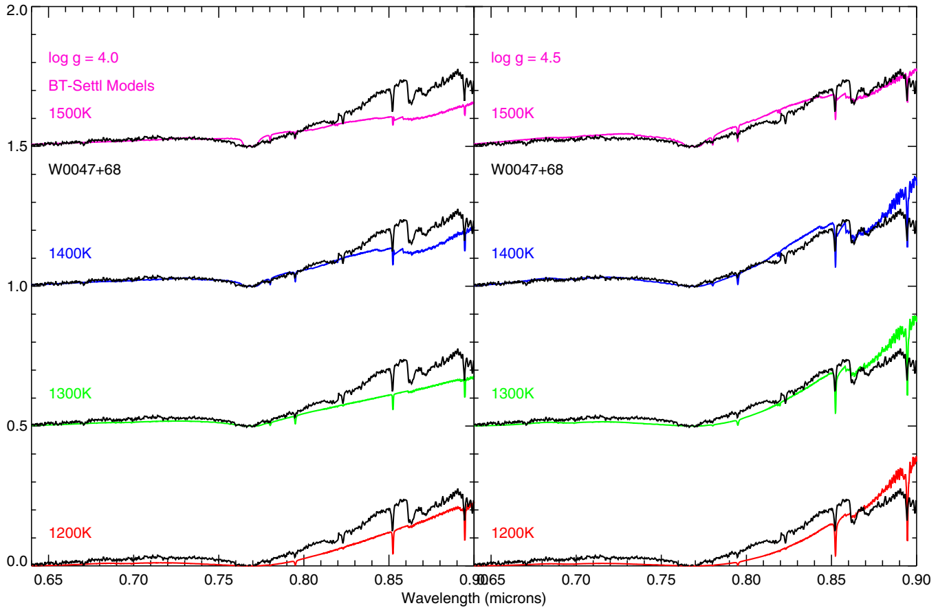
Figure 11. Comparison of observed W0047+68 spectrum to low-gravity ( \log g = 4.0, 4.5 ) BT-Settl models: each is normalized to agree in the 1.5–1.75 \mu\text{m} region. See the discussion in Section 3.4.
