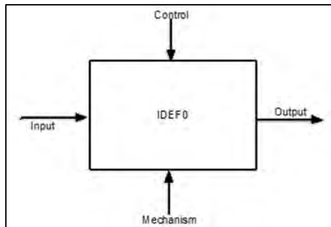
Figure 1. IDEF Methodology
