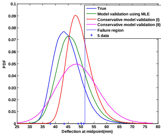
(a) Dataset 1 – Negatively Skewed Data (skewness: -0.6854)
