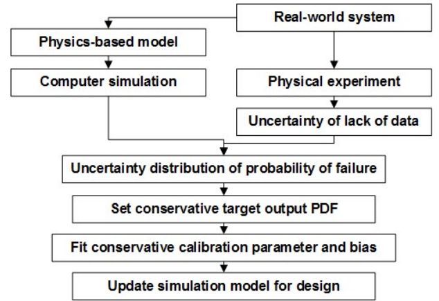
Figure 1. Flowchart of Proposed Model Validation Approach
