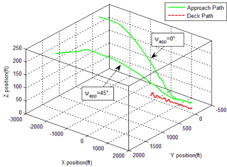
Figure 3 Approach trajectory from 0° and 45° azimuth
