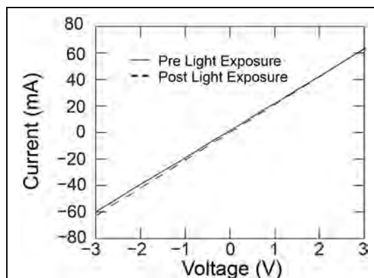
Figure 13. Current-voltage behavior of an ITO-PTMA-Au thin film before and after light exposure for 2 hours from an AM 1.5 solar simulator. The nearly identical behavior before and after light exposure indicate that short term light degradation does not inhibit charge transport within the PTMA film.
