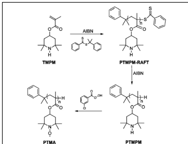
Figure 2. The synthetic route utilized to generate the radical polymer PTMA through a RAFT-mediated polymerization mechanism.
