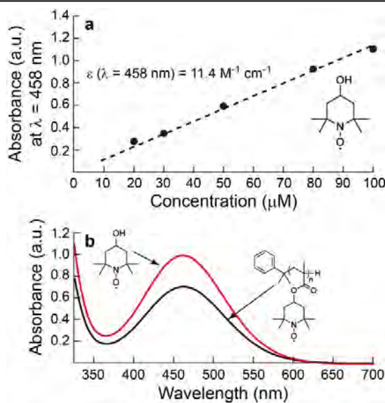
Figure 3. (a) Absorbance of the small molecule, TEMPO-OH (the chemical structure is inset in the figure), in chloroform, which is the small molecule analog to the pendant groups of PTMA. The measured molar absorptivity of this molecule was used to determine the concentration of pendant radicals in PTMA solutions. The dashed line is a linear regression fit to the data points. (b) UV-Vis absorbance spectra of PTMA (black curve) in chloroform at a concentration of 30 mg mL -1 . The red curve of (b) is the absorption spectrum of small molecule TEMPO-OH that would indicate 100% conversion of the protected pendant groups.
