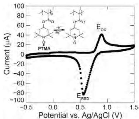
Figure 7. Cyclic voltammogram of a 25 mg of PTMA in 300 mL of dichloromethane (DCM) solution with 1 g of tetrabutylammonium tetrafluoroborate added to solution in order to serve as the supporting electrolyte. The scan was acquired at a rate of 100 \text{ mV s}^{-1} . The reversible oxidation-reduction reaction for the PTMA species (left side of reaction arrow) that is occurring is displayed in the inset.
