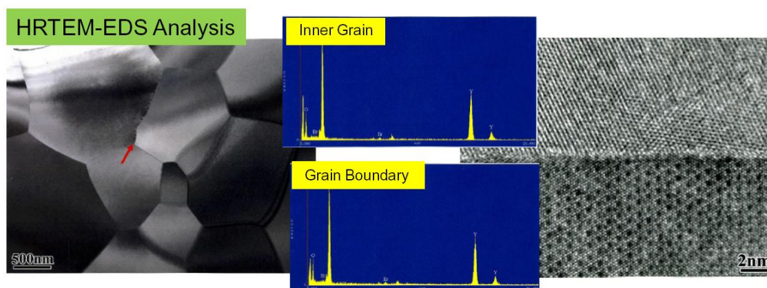
Figure 11(a) SEM-EDS and (b) HRTEM-EDS analysis results for 2%Er:Y 2 O 3 ceramics.
