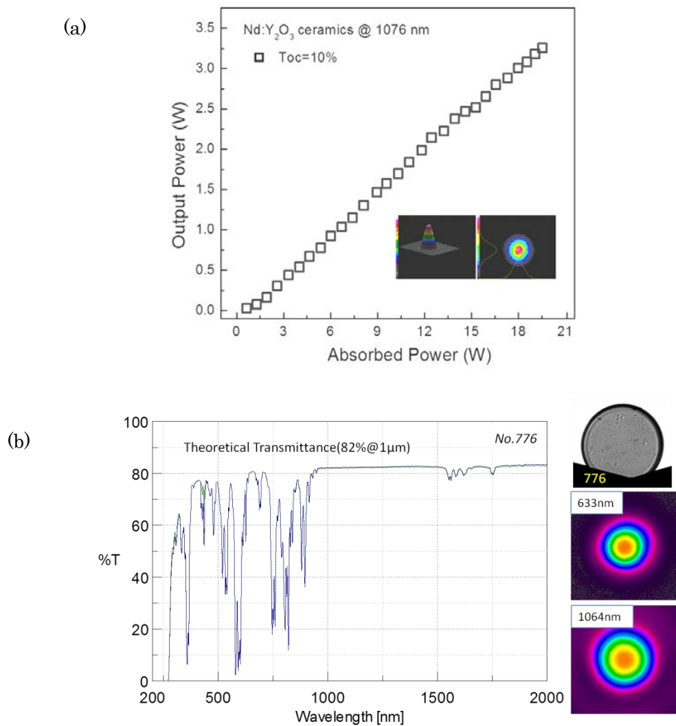
Figure 17(a) Laser oscillation performance for 1%Nd:Y 2 O 3 ceramics (Φ9xt10mm). (b) In-line transmittance, Schlieren image and inspection with beam profiler for the Nd:Y 2 O 3 ceramics.
