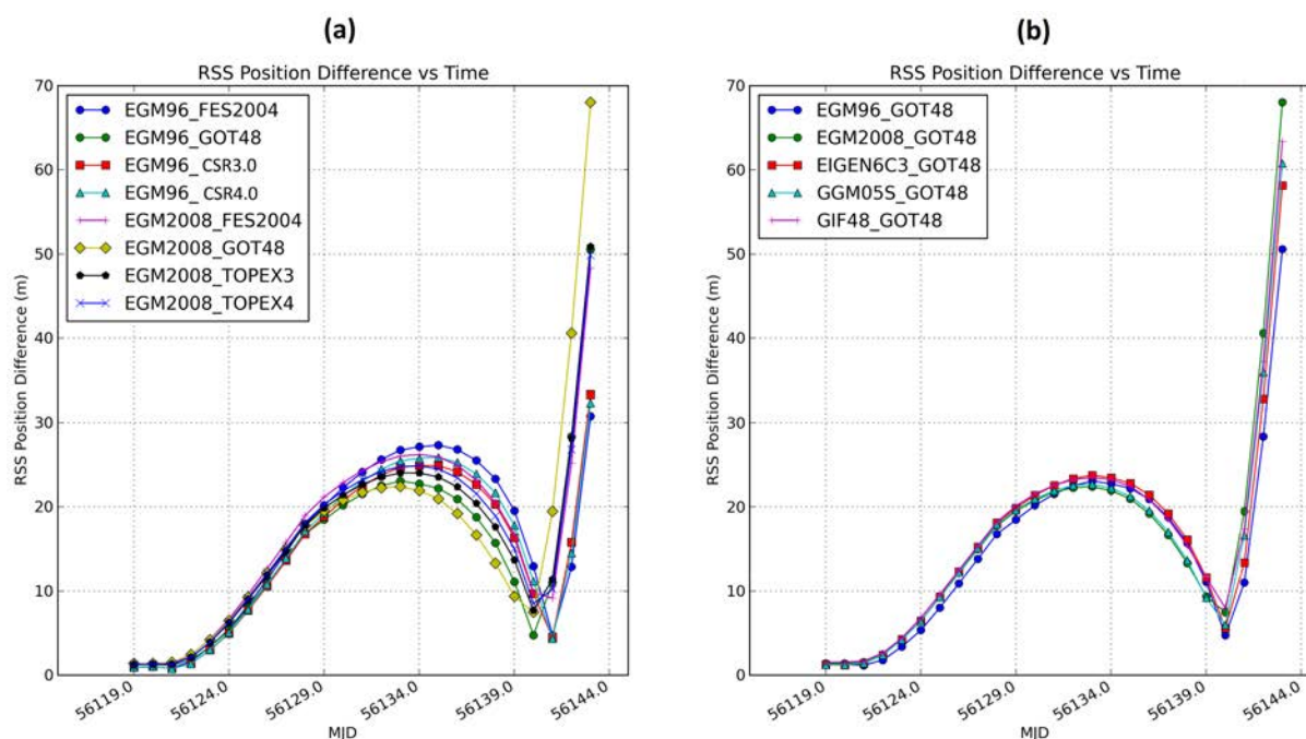
Figure 4: STARLETTE Average Daily RSS Orbit Difference Between Predicted Orbit and Fit Orbit (Left) and STARLETTE Average Daily RSS Orbit Difference Between Predicted Orbit and Fit Orbit for GOT4.8 Ocean Tide Model and Various Geopotential Models (Right)
