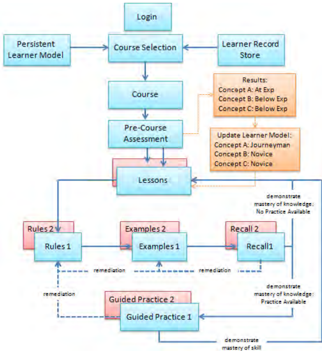
Fig. 3 GIFT's EMAP (Goldberg and Hoffman 2015)
