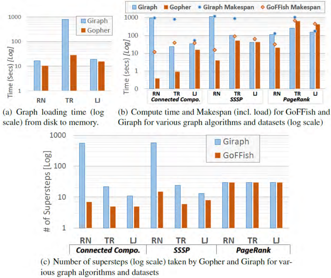
Figure 2. Comparison of GoFFish and Giraph for Connected Components, Single Shortest Path and Page Rank algorithms.
