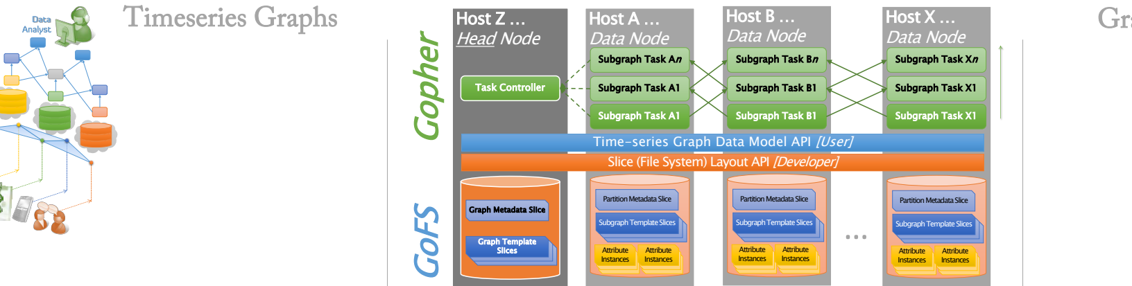
Figure 1: Sample scenario where temporal snapshots of sensor data forms timeseries graph and the GoFFish Architecture.
