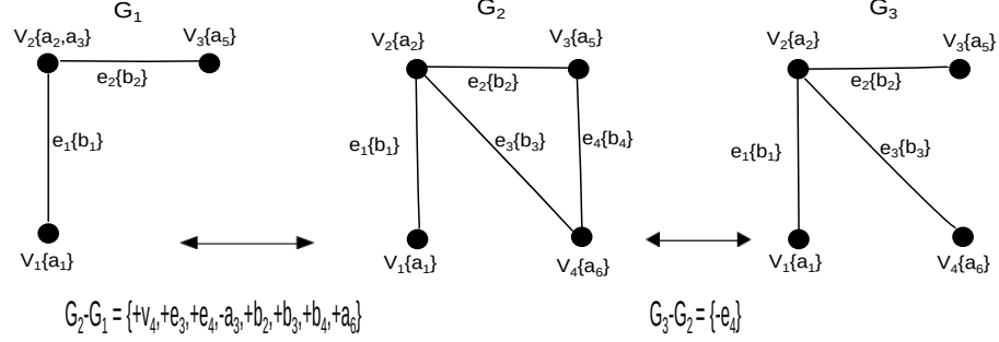
Figure 1. Example of three consecutive graph instances.
