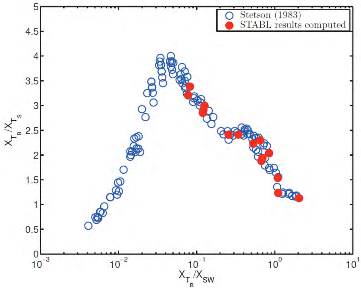
Figure 31 Effect of Nosetip Bluntness (Normalized by the Swallowing Length of Rotta 39 in Terms of the Transition Reynolds Number Ratio (Redrawn from Stetson 34 Figure 9(b).)
