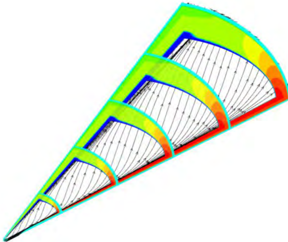
Figure 1 Rollup of Boundary-layer into Streamwise Vortex on 2:1 Sharp Elliptic Cone, Similar to HIFiRE-5 (from Ref. 9) (Contours are fluid density.)
