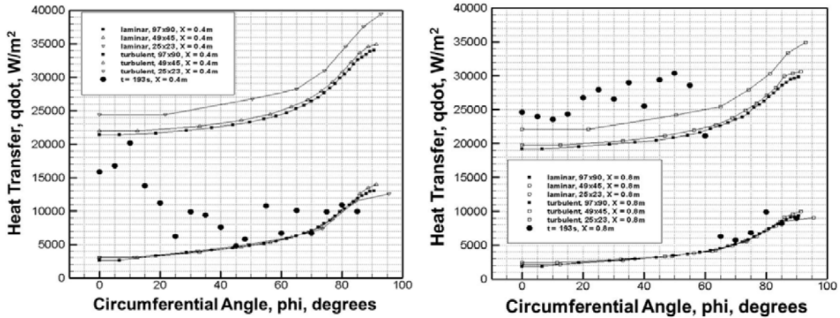
Figure 22 Heat Transfer at Mach 2.6 Conditions at x = 0.4 m and 0.8 m
