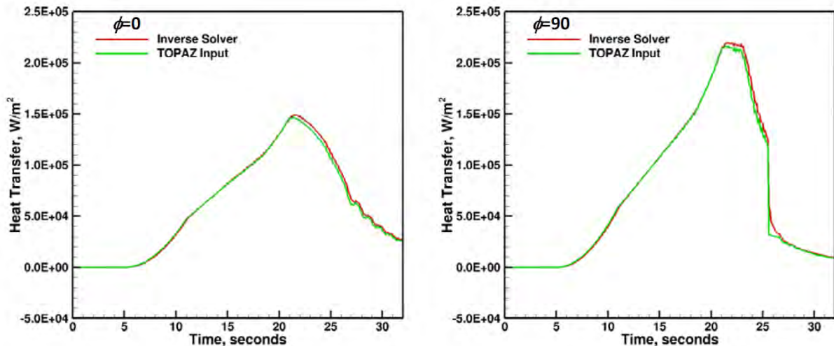
Figure 28 Input and Derived Heating Rates for the Circular Cone at x=400 mm
