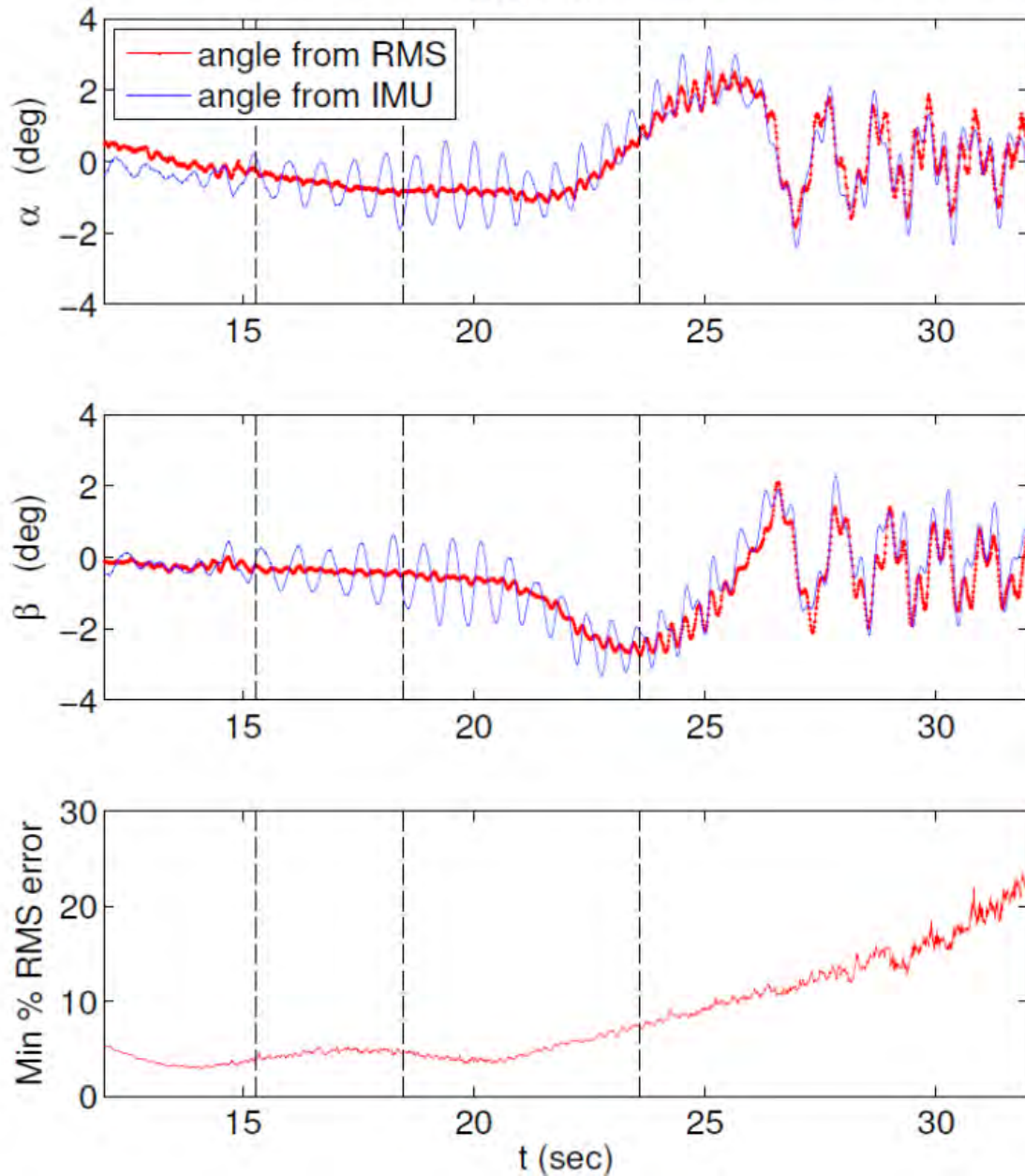
Figure 24 AoA and Yaw Results for the Ascent Portion of the Trajectory from the Interpolation/RMS Minimization Routine Compared with the IMU Values
