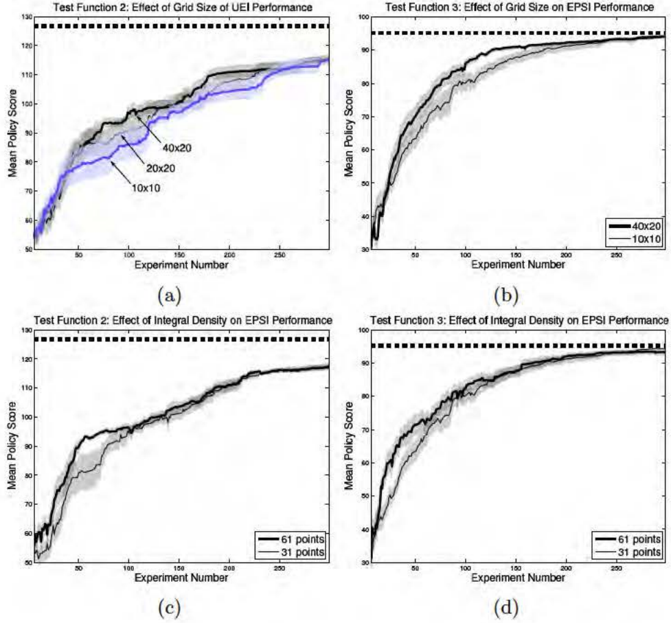
Figure 6.10: A comparison of the effect of grid resolution (top row) and numeric integral density (bottom row) on algorithm performance. In general, higher density candidate point grids and numeric integrals resulted in improvements in the quality of results. All EPSI results shown use \pm 3 standard deviations of p(y) as the limits to the numeric integral. Each line represents the mean of 20 trials, and the shaded regions indicate \pm 1 standard error.
