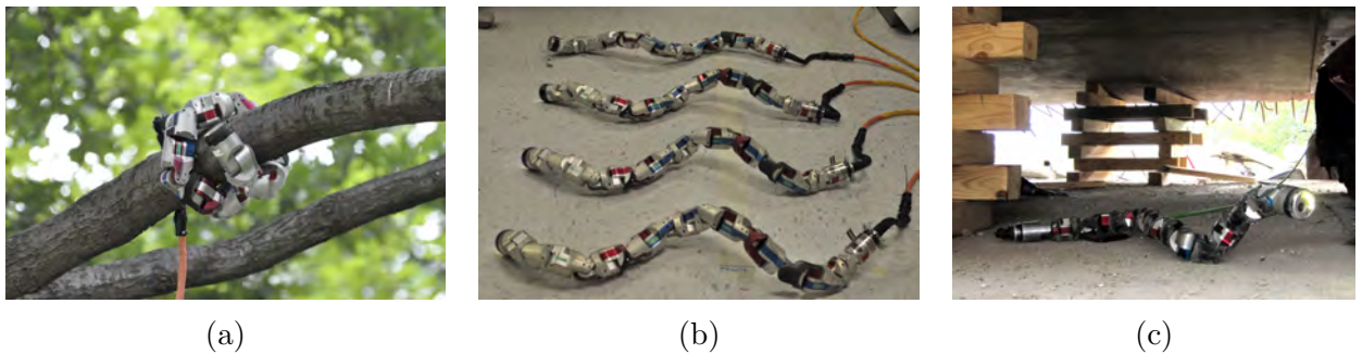
Figure 2.9: (a) Snake robot locomoting along a tree branch. (b) Time-lapse snapshots of the sidewinding gait. (c) Robot deployed in a mock building collapse.
