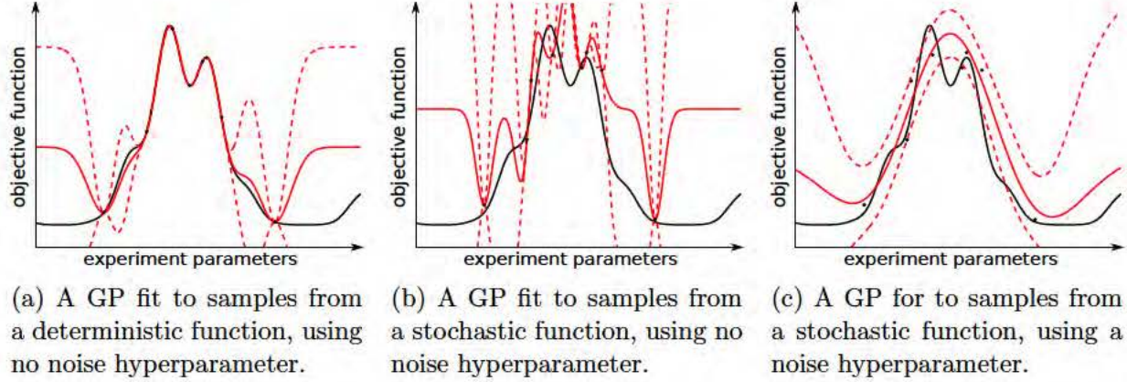
Figure 2.8: Effects of stochasticity in the objective and noise covariance function hyperparameters on GP regression. The black solid line is the function, the red line is the GP posterior mean, and the red dotted lines are one standard deviation uncertainty bounds of the GP predictive distribution. Fitting stochastic data without an explicit noise hyperparameter leads to overfitting (see (b)), as the GP attempts to interpolate the observations exactly. (c) Using a noise hyperparameter eliminates this overfitting.
