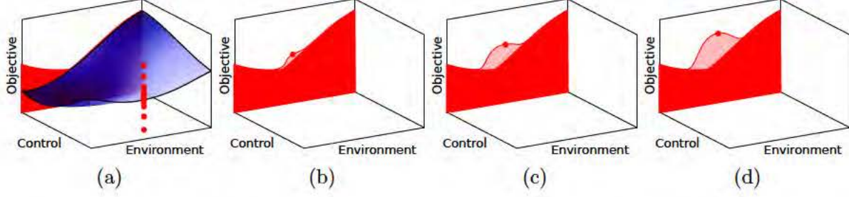
Figure 6.6: EPSI provides a measure of the potential improvement to the score of the estimated optimal policy \hat{\gamma}^* resulting from sampling at some x^i . (a) Sampled values from the distribution at \hat{f}(x^i) are shown; this is a sampling of the GP posterior at this point. The policy score given \hat{f} is the shaded region on the objective/environment plane. (b) - (d) New estimates of the policy score are generated by updating \hat{f} with these samples. The lightly shaded regions show the predicted improvement over \mathcal{S}(\hat{\gamma}^*) , the estimated optimal policy score. The EPSI is the weighted combination of these policy score improvement contributions.
