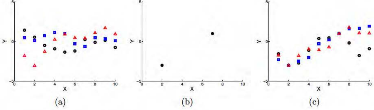
Figure 2.5: (a) A GP with a squared exponential covariance function and zero mean is used to generate a multivariate Gaussian over random variables associated with points \{1, 2, \dots, 10\} \subset X . Three samples are drawn from this distribution, and plotted as the black circles, red triangles, and blue squares. (b) Two points are chosen in X \times Y (perhaps evaluations of some unknown function). (c) The GP from (a) is conditioned on these points, and three new samples are drawn from the posterior. Notice that the samples all interpolate these points; the posterior distribution's variance has collapsed to zero in these dimensions.
