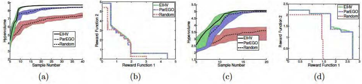
Figure 5.6: Results of two different expensive MOO methods – optimization of the expected improvement in hypervolume (EIHV) and ParEGO – and a random experiment selection baseline on the 1-D (a) and 2-D (c) test functions shown in Figure 5.5. The line indicates the median hypervolume of the 20 trials, while the shaded regions represent the middle 50% of the trials. Also shown are the resulting Pareto frontiers from each method on each test function ((b) and (d)). On both functions EIHV outperforms ParEGO, and both methods are significantly better than random, demonstrating the importance of careful experiment selection in expensive optimization.
