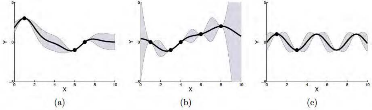
Figure 2.6: A useful, albeit incomplete, visualization of a GP is obtained by plotting the mean function along with a shaded confidence region of the pointwise standard deviations. (a) Posterior from a GP with a squared exponential covariance and hyperparameters \ell = 1 and \sigma_f^2 = 1 . (b) Squared exponential covariance with \ell = 1.4 and \sigma_f^2 = 4 . (c) Periodic covariance with \ell = 2 , \lambda = 5 , and \sigma_f^2 = 2 .
