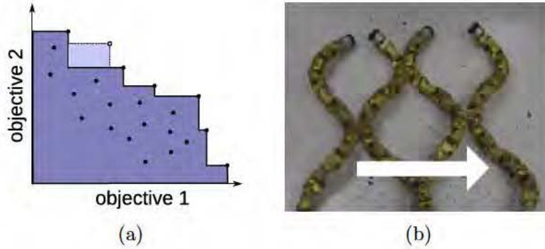
Figure 5.1: (a) The set of Pareto optimal solutions are those that are not Pareto dominated by any other points in the full set of solutions. The Pareto optimal points in this figure are those which are on the stair-stepped line. The hypervolume of such a set is the volume which is dominated by the Pareto set, shown as the dark shaded region; this is a popular measure of the quality of a multi-objective solution set. The light shaded region is the potential improvement to the hypervolume if the point indicated by the circle were added to the set. (b) One problem when teleoperating our snake robots is that the large movement of the head, which houses the camera, can cause operators to become disorientated. We demonstrate multi-objective optimization methods in this chapter to help solve this problem, simultaneously optimizing for the conflicting objectives of head stability and speed.
