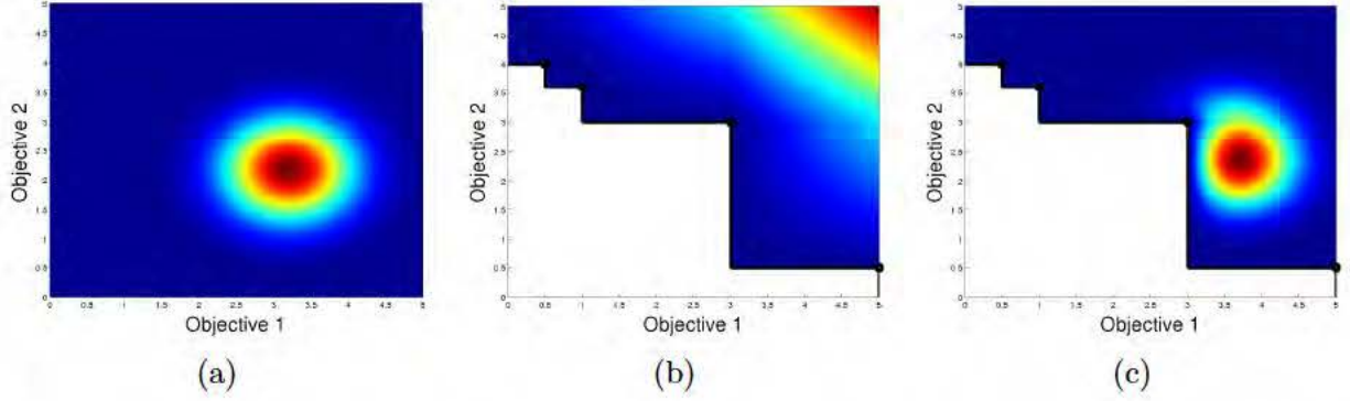
Figure 5.3: These objective space plots are computed using the example samples and function fits from Fig. 5.2. The expected improvement in hypervolume (EIHV) for a given parameter x = 8 is the expectation over the improvement in hypervolume for potential objective values \hat{\mathbf{f}}^x . Therefore, the integrand (c) is the (a) probability density of \hat{\mathbf{f}}^x times the (b) improvement for each potential y in the objective space Y_1 \times Y_2 \dots Y_n . The resulting quantity is integrated over the objective space to obtain the final \text{EIHV}(x) value.
