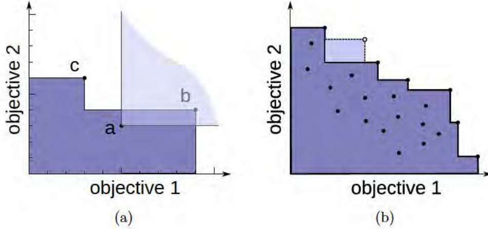
Figure 2.11: Objective-space illustrations of a multi-objective optimization problem. Sampled points are solid circles, and the Pareto front (or frontier) is created by connecting Pareto optimal samples; it is illustrated by the bold jagged line. (a): A simple example of Pareto dominance. The dark shaded region shows the area that is Pareto dominated by the Pareto optimal set \{b, c\} . The light shaded region indicates areas of the space that Pareto dominate a . (b): The dark shaded area represents the hypervolume of the currently known Pareto front; the lightly shaded area is the hypervolume increase resulting from a sample at the location of the circle.
