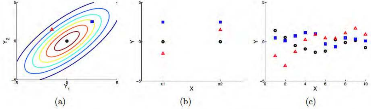
Figure 2.4: (a) A bivariate Gaussian PDF with three points selected. (b) Each of the random variables from (a) is associated with a point in X . The three points shown in (a) are shown as sets of points here, including the circles which represent the mean, or most likely values. (c) As more points are added, and the multivariate Gaussian becomes harder to visualize, each sample from that Gaussian approximates a function from X to Y ; this is shown here with 10 points.
