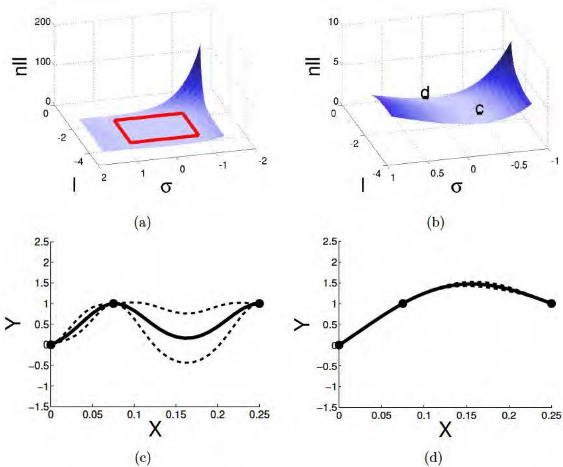
Figure 4.2: (a) When conditioning on sparse data, large regions of the likelihood surface can be relatively uniform, causing it to be difficult to reason between different hyperparameter values. (b) A zoomed in view of the red boxed region of (a); the central valley also extends much further as \ell decreases with no significant change in the negative log likelihood value. The different markers correspond to the different GP fits in (c) and (d), which have approximately the same likelihood but represent significantly different hypotheses.
