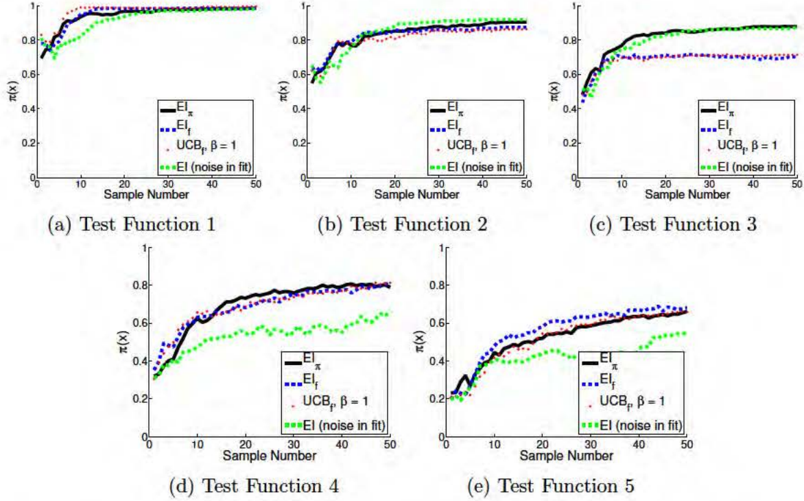
Figure 8.4: As in Fig. 8.3, the average expected probability of success for each algorithm’s recommendation at each step is shown above. These results, averaged over 100 runs of each algorithm, compare the proposed EI_\pi algorithm with use of EI and upper confidence bounds on the latent function obtained while fitting a GP to binary data, and EI on a GP fit directly to the 0/1 data with a tuned noise parameter.
