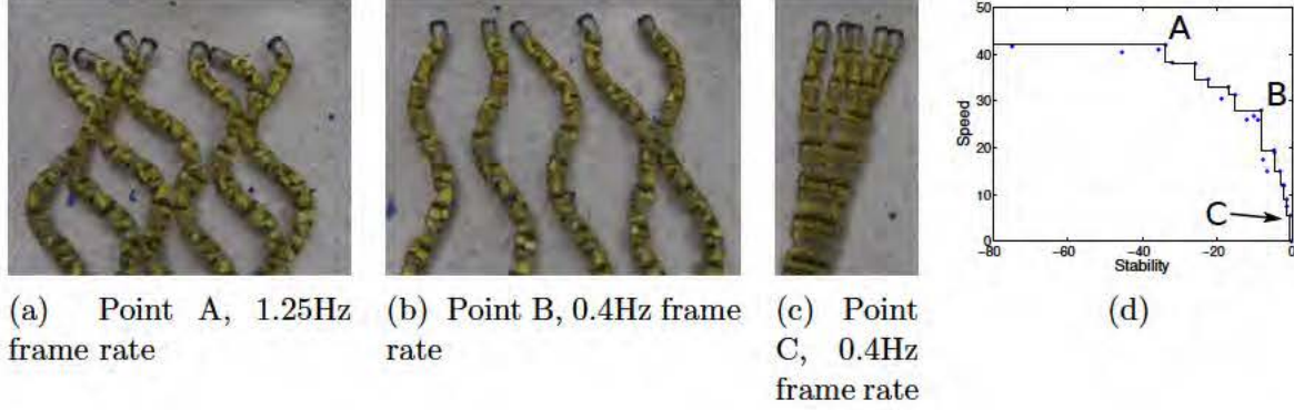
Figure 5.8: (a)-(c) Time lapse images showing the head and snake motion of three different points in the head stability/speed Pareto set. The snake in (a) moves quickly, but the head rotates back and forth. The snake in (b) moves at a slower rate, but with noticeably less head sway. Finally, (c) is a very slow but very head-stable motion. As can be seen in (d), these points span the Pareto front, and none dominate the others. Shown as blue dots are the results of all experimental evaluations during the optimization.
