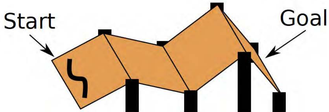
Figure 6.12: Diagram of test course. The robot was placed at the start location to begin, with the task of reaching the goal location in the minimum amount of time. The slope of each segment can be set independently, and is estimated in real time as the robot moves along the segment.
