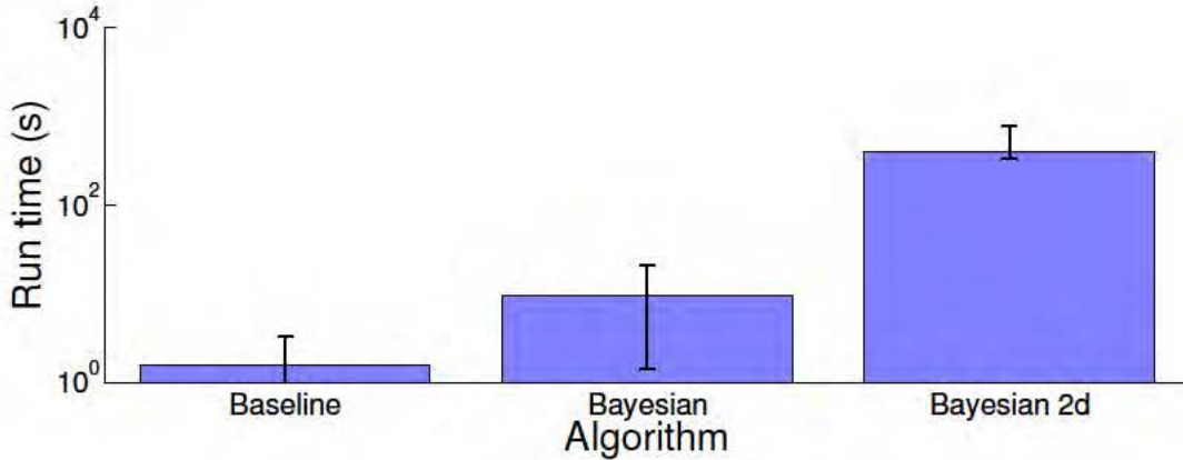
Figure 4.10: A comparison of the computational time required for the different algorithms (during optimization of test function 2). In each category of methods (baseline, Bayesian, and 2-D Bayesian) the results were comparable, so only one example of each is shown. The height of the bar represents the average computation on steps 11-20, and the error bars give the 25th and 75th quantile. Note that the data is on a semilog plot; the computation required for more complex methods is several orders of magnitude more than the simpler methods. These tests were run on a 2.6 GHz Intel Core 2 processor.
