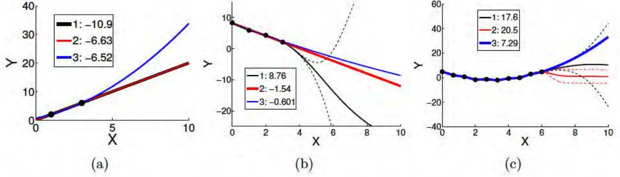
Figure 4.4: Automatic model selection can be accomplished by choosing a mean and covariance function whose MLE hyperparameters result in the highest likelihood over all of the models. Each figure above is shown with GP posteriors using the MLE hyperparameters for three models of varying complexity (each used an isometric squared exponential covariance, and the mean functions were mx , mx + b , and ax^2 + bx + c ), with the most likely drawn as a thicker line. The legend also displays the negative log likelihood of each. For a small number of data points, simple models are chosen; as the complexity of the data increases, more complex models are naturally chosen. This automatic model selection serves to help reduce overfitting.
