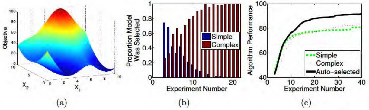
Figure 4.6: The result of model selection on optimization with EI on a simple noisy test function. Each algorithm was run 50 times. (a) The latent deterministic test function; Gaussian noise with a standard deviation of 4 was added. (b) For the auto-selection approach, the proportion of experiments in which each model was chosen after a certain number of data points. (c) The average optimization performance in terms of best sampled point for each single covariance function as well as the automatic model selection process.
