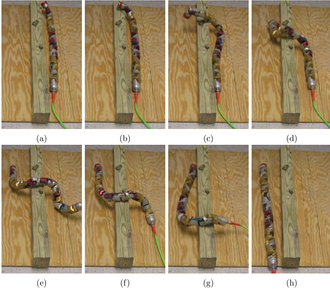
Figure 8.5: After completion of the optimization, the predicted best parameters result in a robust motion which successfully moves the snake robot over the obstacle.
