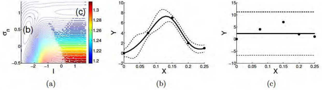
Figure 4.5: (a) A slice from the 3 dimensional negative log likelihood surface for a squared exponential covariance function with a diagonal noise term (the signal parameter \sigma_f varies from 3.6 to 2.5 with the change in \ell in order to capture both minima in this surface). For visualization purposes (to avoid washing out the minima due to the scale of the remainder of the surface), a tan scaling has been applied. (b) The GP fit corresponding to the maximum that explains the data as relatively low noise. (c) The GP fit corresponding to the maximum that explains the data as pure noise.
