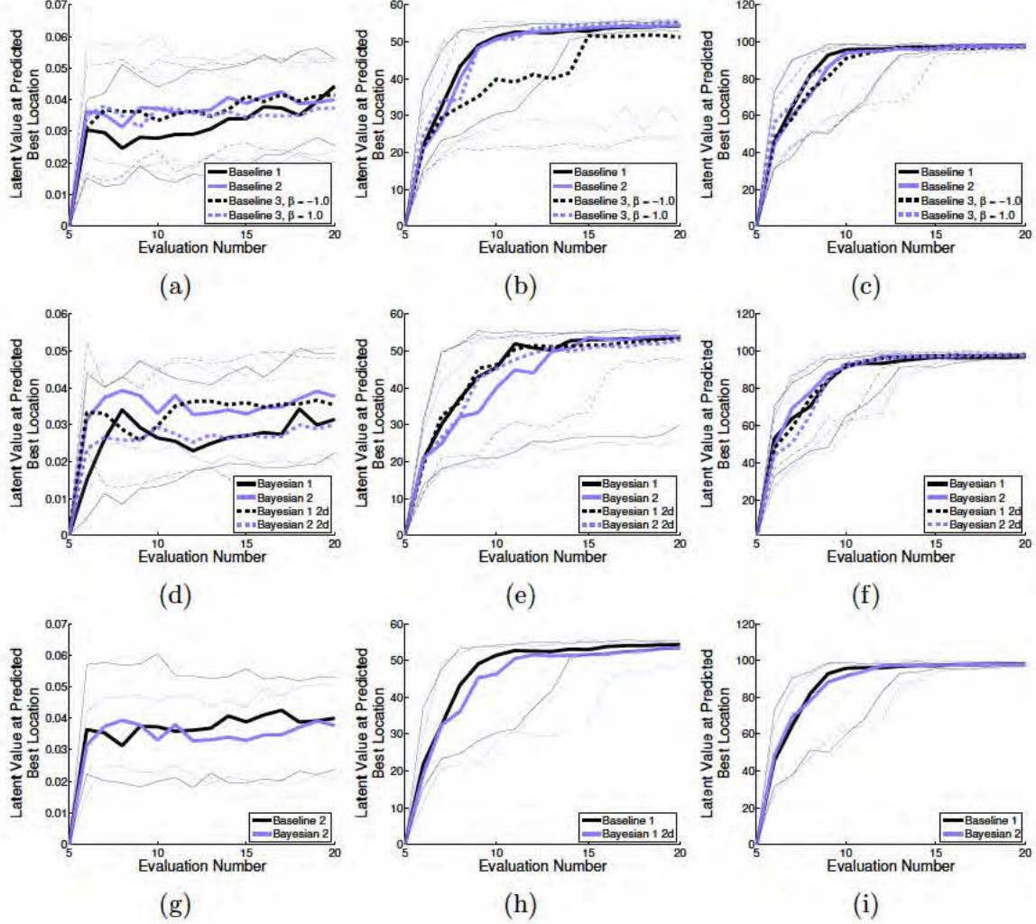
Figure 4.9: For each test function, 50 tests were run for each approach described in the text. Each column shows results from the test function in the corresponding column of Fig. 4.8. The first row compares the baseline approaches, the second row the described Bayesian approaches (using both 1-D and 2-D integrals), and the third row compares the best baseline to the best Bayesian approach. The thick lines are the median algorithm performance, defined as the quality of the recommendation, and the thin lines are 25% and 75% quantiles. Note that for each test functions, the baselines perform on par with or better than the best Bayesian approach.
