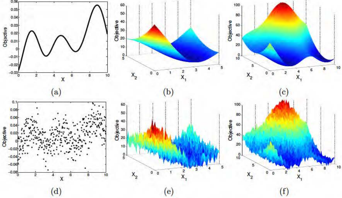
Figure 4.8: Test functions considered for an empirical comparison of various adaptations of the EI metric to stochastic functions. The top row shows the deterministic latent f_{\text{lat}} , and the bottom row a dense sampling of the stochastic f_{\text{noisy}} . From left to right, a 1-D function with a high level of noise, a 2-D function with a medium level of noise, and a second 2-D function.
