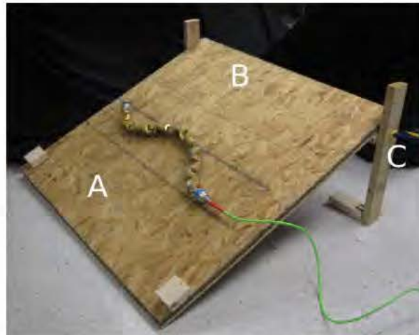
Figure 6.13: The training setup consisted of a 4 foot by 4 foot plywood sheet. The robot began at a small circle at point A for uphill trials, and one at point B for downhill slopes. The height of the test setup was changed when requested by the optimization algorithm by adjusting one quick clamp on each side of the plywood sheet, and clamping on to small blocks of wood attached to the underside of the sheet. The distance travelled was measured by comparison of the snake's position at the end of ten seconds to ruled markings drawn on the wood.
