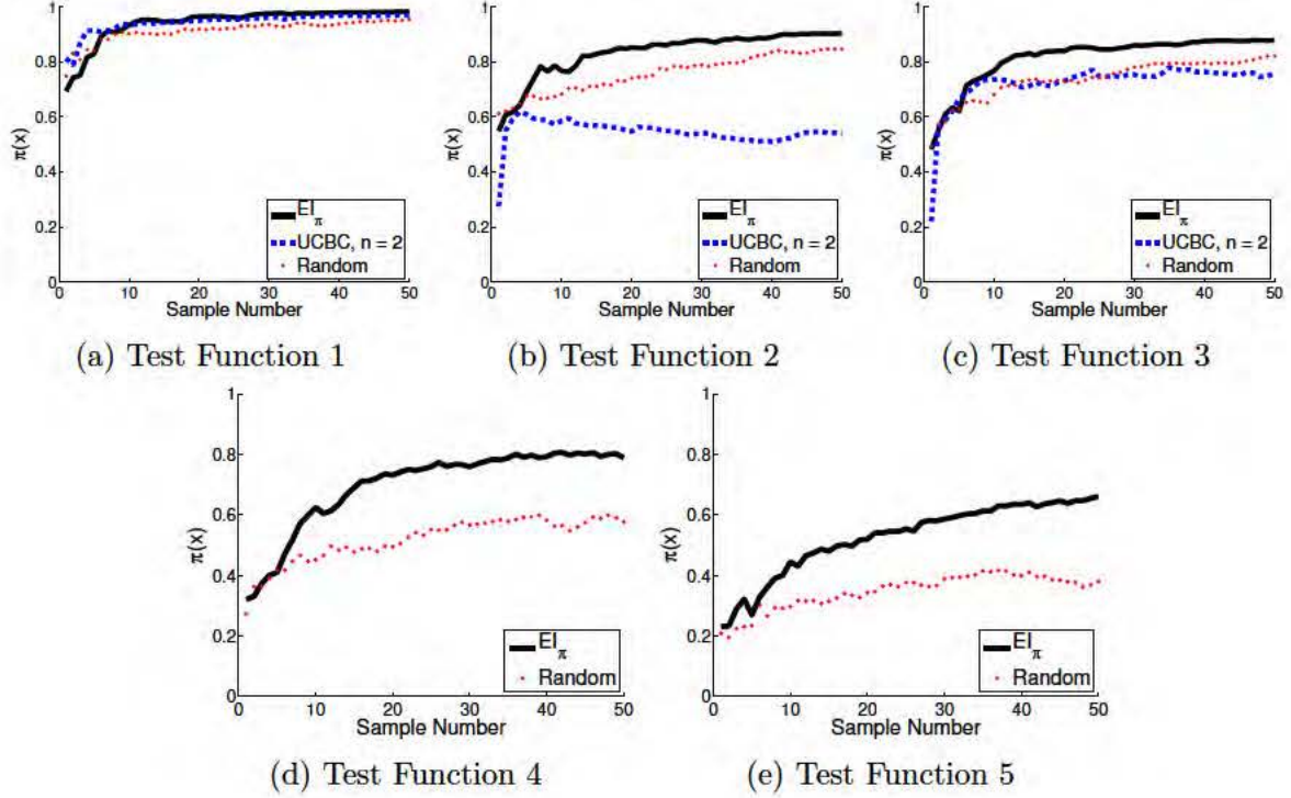
Figure 8.3: After each sample, each algorithm was queried as to its recommendation for a point x that would have a maximum expectation of success \pi(x) ; these results show the underlying probability value of that point averaged over 100 runs of each algorithm. Here I compare the stochastic binary EI ( EI_\pi ) to the continuous-armed bandit algorithm UCBC suggested in [4] as well as uniform random selection. The cause of the unusual drop in performance of UCBC with more samples on test function 2 has not been determined.
