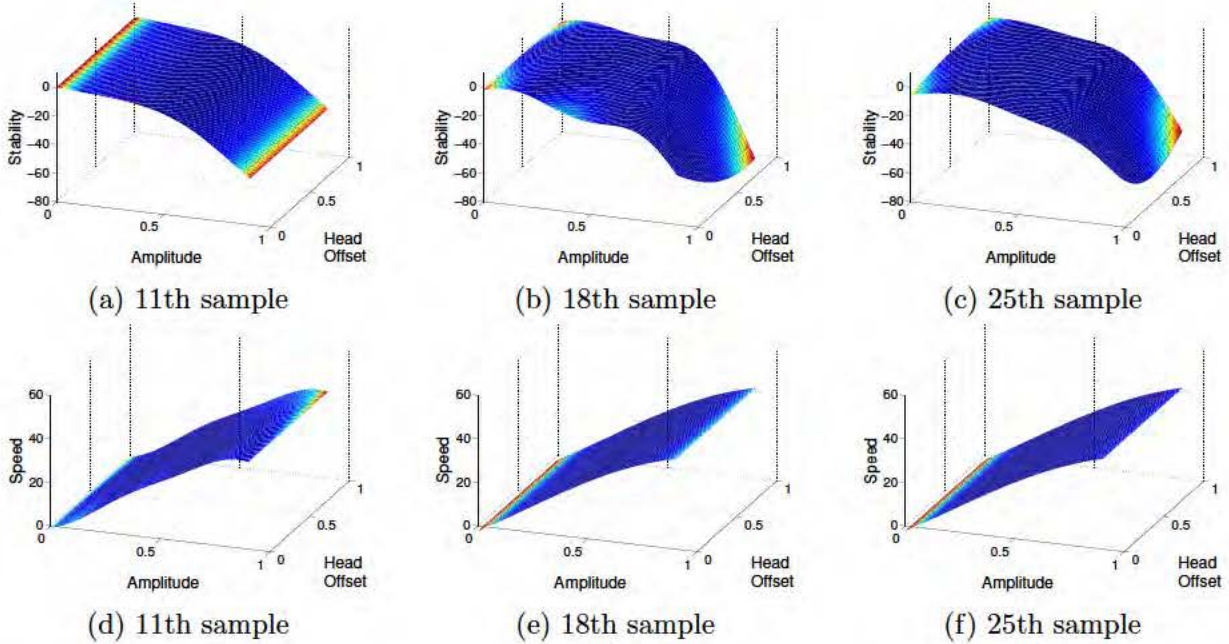
Figure 5.7: After the initial random experiments, the GP function regression method generates an estimate of the function after each subsequent sample. These surfaces are shown here for three selected iterations, where the top row is regression of the stability objective and the bottom is the regression of the speed objective. The color of the surface is the uncertainty in the estimate (blue regions in the center have low uncertainty, red regions near the edge have high uncertainty).
