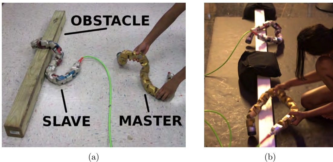
Figure 7.1: (a) In the kinesthetic control approach, a user moves a compliant input snake (often termed the “master” or a “dolly”), and the controlled “slave” robot mirrors the commanded shape. This can be an effective way to locomote the snake in challenging situations. (b) This demonstration process was used for large scale data collection at Chicago’s Museum of Science and Industry; over the course of three days at the museum, nearly 10% of the 276 attempts that were made by visitors succeeded.
