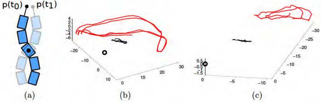
Figure 5.9: (a) The focal point p(t) is a distance l from the head camera, normal to the image plane; it is shown here for two different timesteps. The motion of this point provides a measure of head stability. (b) The head stability objective used for the snake robot trials was the estimated swept area of the head camera’s focal point. The data above from one of the trials shows the center of mass of the robot (black circle), the trace of the head (black line) and the trace of this focal point (red line) through multiple cycles of the commanded gait. The wide sweeps of the head result in a poor objective score of -68.6 ( V = 11.5 and H = 59.6 ). (c) The same plot for a trial resulting in a more stable head trajectory; the resulting head stability objective is -2.70 ( V = 2.75 and H = 9.81 ).
