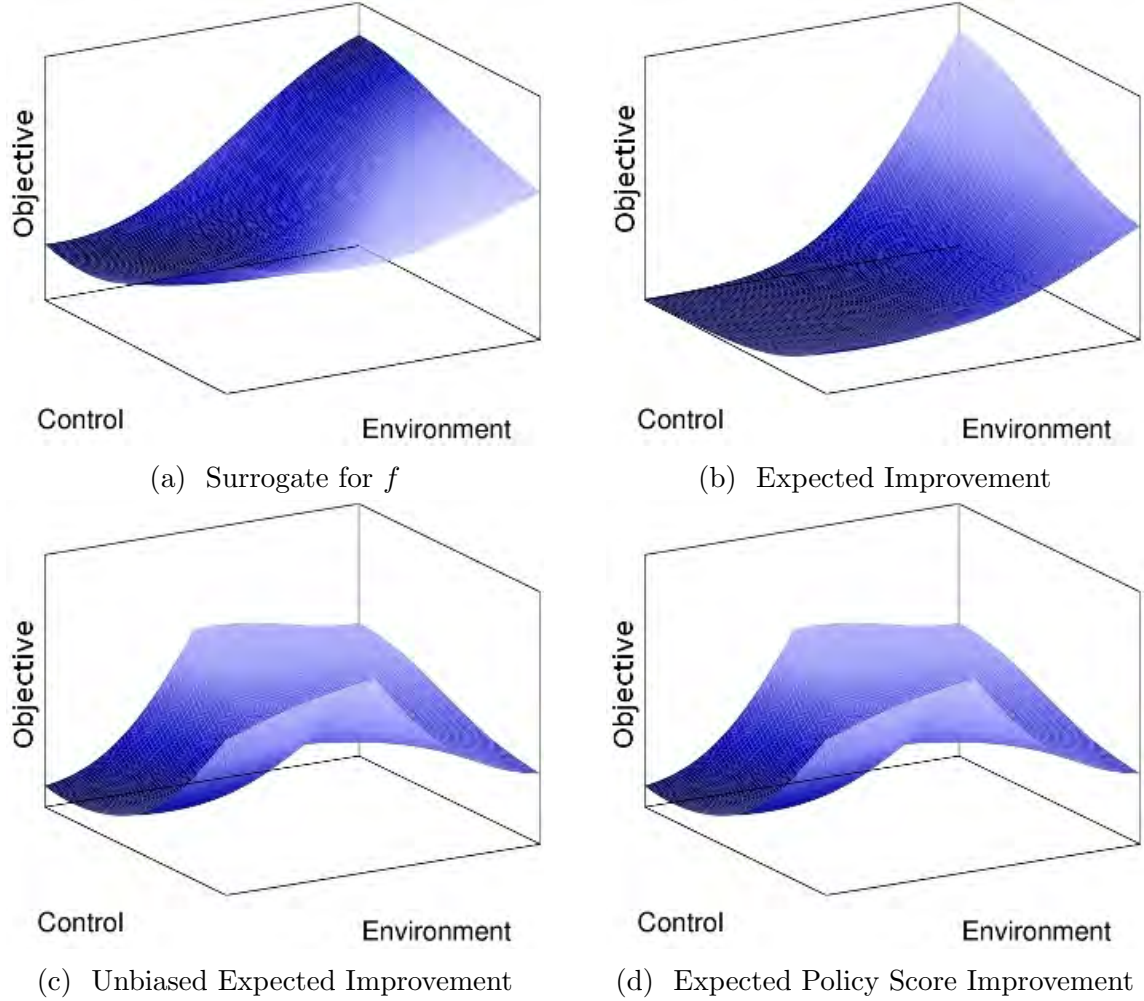
Figure 6.4: (a) A surrogate for the objective f ; the intensity represents the confidence (dark = high, light = low). (b) The value of a potential experiment using EI. The EI metric biases point selection towards environments with high objective values. (c) The value of a potential experiment using EI over the best predicted objective value for that environment. This reduces this bias toward easy environments and more directly optimizes the policy score. (d) The estimated policy score improvement as a result of sampling each point. This selection criterion is computationally intensive, but results in better performance than (c).
