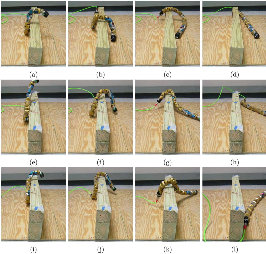
Figure 8.7: Successful trials from optimizations for 5.5 (top), 7 (center), and 9 (bottom) inch obstacles. The robot started at the left side of the obstacle, and moved over the obstacle to the right.
