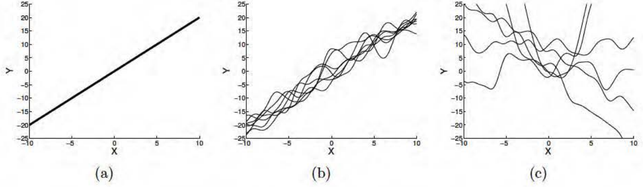
Figure 2.1: The mean function describes the average expected function value. If the mean function is a simple linear function such as (a), then functions such as (b) have higher likelihoods than those given in (c), because they are closer to the expected value.
