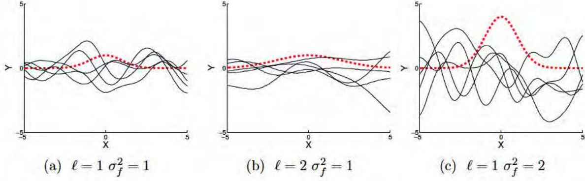
Figure 2.3: The black solid lines are samples drawn from GP priors with a squared exponential covariance function and three different hyperparameter values. The red dashed line is the covariance function k(x, x') with x' = 0 . (a) The length scale parameter is set to 1, as is the signal variance. (b) When the length scale increases, typical function samples are smoother and vary less quickly – values are more correlated across the spatial dimension. (c) When the signal variance increases, the amplitude of typical function samples increases.
