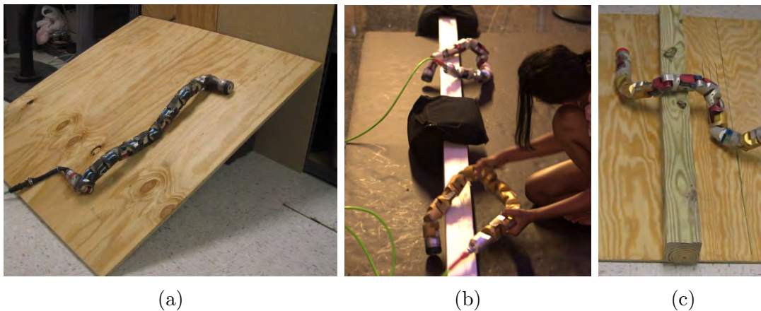
Figure 1.1: This thesis develops learning algorithms for robotics applications; this includes (a) optimization of motion in steady-state settings, (b) learning from demonstration, and (c) overcoming obstacles with limited feedback.
