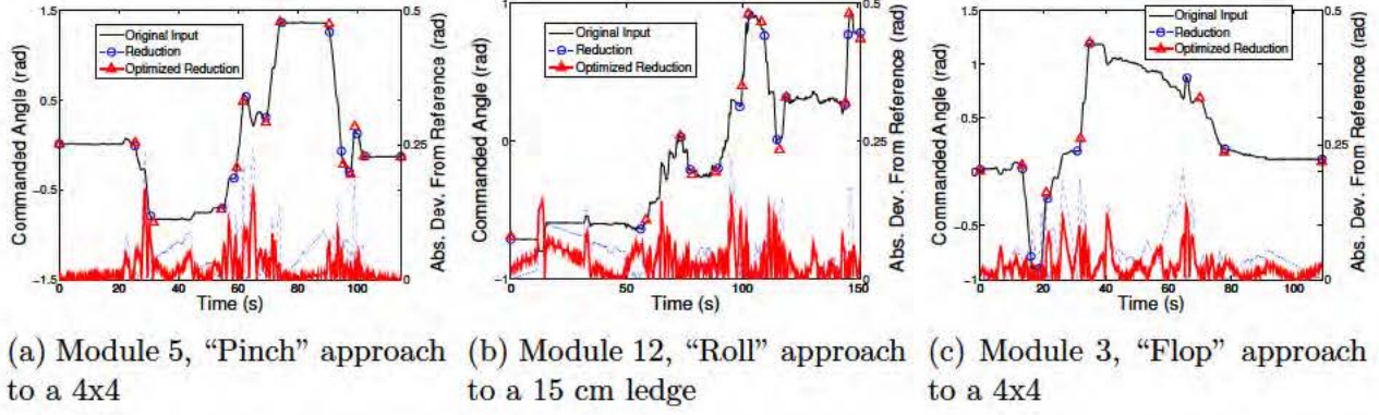
Figure 7.5: These plots show the fidelity of a piecewise linear approximation to the original kinesthetic input for three randomly selected joint angle trajectories. The original trajectory is shown by the solid black line. Simply reducing from a dense interpolation of the input (here, the mean-squared error threshold was 0.004 \text{ rad}^2 ) gives a fair approximation to the input; the circular markers indicate the linear segment endpoints and the dotted blue line indicates the deviation of this approximation from the original (right axis scale). The secondary gradient descent optimization over the linear segment endpoints provides a noticeable improvement (triangular segment endpoints and red solid line for deviation). Note that by moving to a piecewise linear parameterization, the amount of information that needs to be stored for these trajectories reduce from 2774, 3652, and 2636 points in \mathbb{R}^2 to 14, 13, and 10, respectively.
