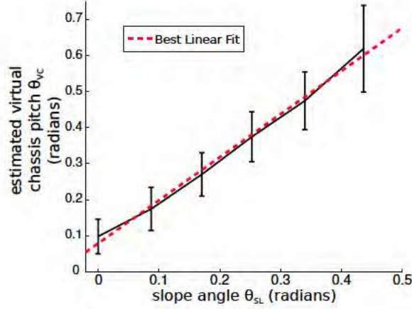
Figure 6.16: The bars in the figure denote the variance of estimated virtual chassis pitch \theta_{VC} with different gait parameters and on different slopes. A linear relation between the slope angle \theta_{SL} and virtual chassis pitch \theta_{VC} is revealed.
