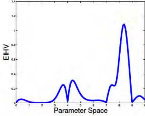
Figure 5.4: The expected improvement in hypervolume for each point in the parameter space (corresponding to the GP fits in Fig. 5.2).
