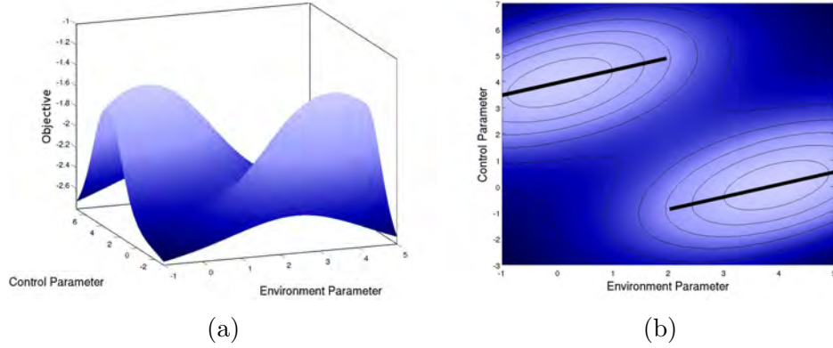
Figure 6.2: (a) I am interested in problems for which the optimal control parameter changes significantly with changes in the environmental conditions. Ideally similar environment/control combinations lead to similar system output; I therefore assume this function is continuous, although these methods can still operate with some discontinuities. (b) The optimal policy (dark lines that indicate mapping from environment to control) tends to be piecewise continuous; similar environments usually result in similar controllers, but there are likely to be some discontinuities. A good policy can be estimated from a low-cost model of the true expensive system output, requiring only a handful of carefully chosen points.
