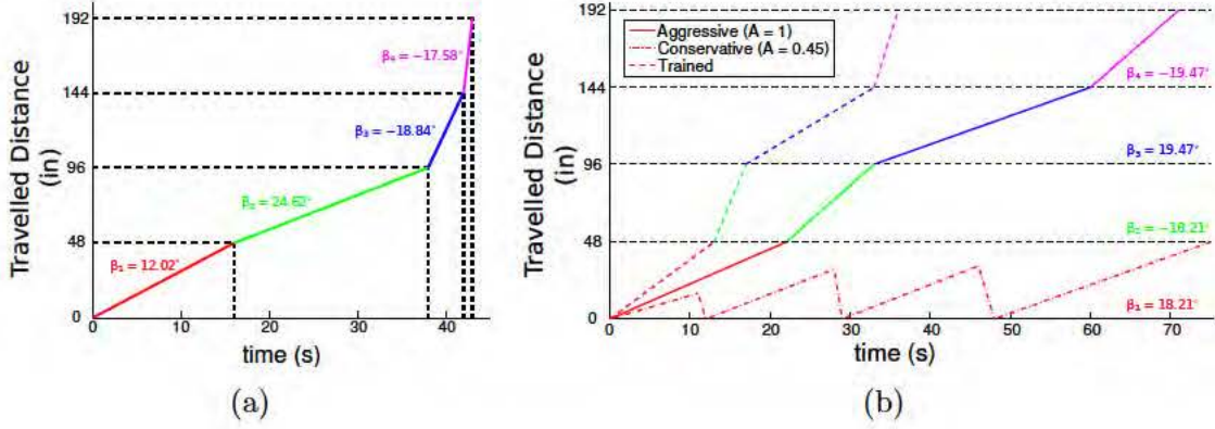
Figure 6.18: (a) Performance of adaptive sidewinding on a simple test course. The slope of each line denotes the travelling speed, and different colors represent panels at different slopes. (b) A comparison among three strategies (shown in different line types). Sidewinding with a small amplitude failed to finish the task, and the conservative approach of sidewinding with a large amplitude leads to slow completion. The adaptive strategy outperforms both static policies.
