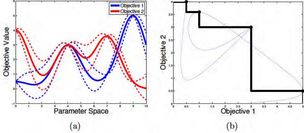
Figure 5.2: Two objectives were sampled at \tilde{x} = \{0, 4, 7, 9\} . (a) The resulting GP fits. (b) The objective space projection of the GP fits is shown as the thin line, while the thick line indicates the current Pareto front of the sampled points.
