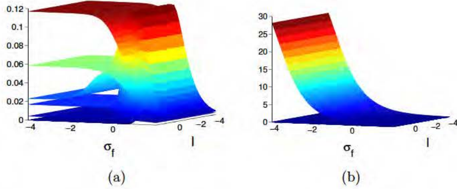
Figure 4.3: (a) Sections of the likelihood surface for a three-hyperparameter model (isometric squared exponential covariance plus a diagonal noise term). The 2-D l and \sigma_f surfaces are shown for various values of \sigma_n . (b) When the simpler two-hyperparameter model (zero mean, isometric squared exponential covariance) is used, the likelihoods are much larger – the sloping surface is the likelihood for the two parameter model, whereas the slices from the three parameter model is shown at the very bottom – note the differing scales between these figures.
