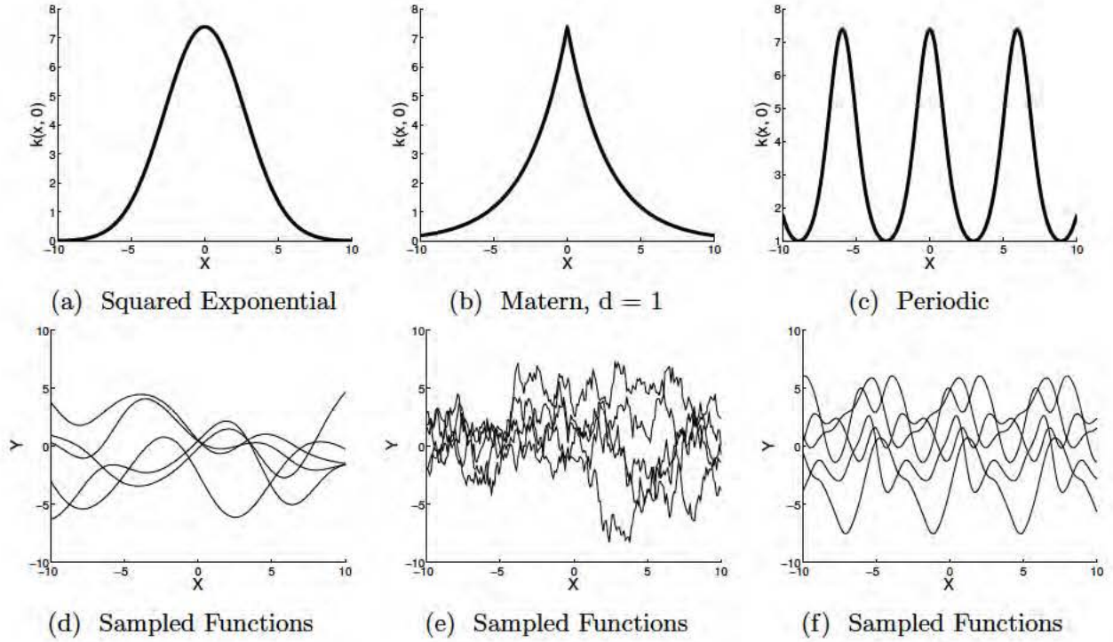
Figure 2.2: The covariance function describes how points in the space are correlated. Each figure in the top row shows the covariance function output k(x, x') , where x' is set to zero and x is allowed to vary. Higher values indicate higher correlation between function values at these points. Each bottom row figure shows samples from a GP prior with a zero mean function and the covariance function pictured above it.
