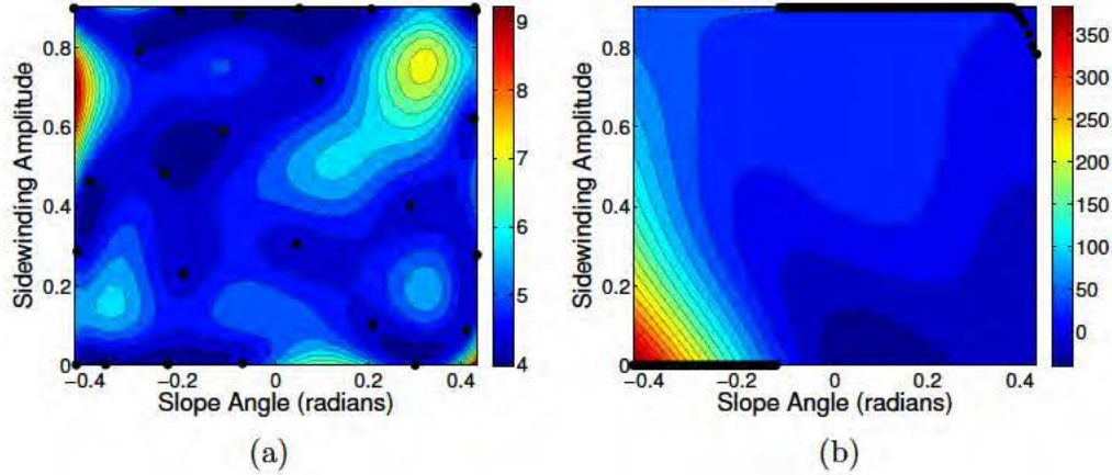
Figure 6.15: GP posterior pointwise variance and mean after sampling budget has been exhausted. (a) Uncertainty in the final objective function estimate. The black dots in the figure are the 25 sampled points. The uncertainty is highest furthest from the sampled points. (b) The mean predicted objective. The optimal policy is shown by the large black dots; at steep downhill slopes, the optimization determines that a zero-amplitude sidewinding gait is most effective (this gait rolls down the hill very quickly). At a critical slope, the optimal control switches to a high amplitude sidewinding gait. At very steep slopes the optimal control parameter decreases slightly; perhaps this decreased amplitude increases the stability or repeatability of the motion.
