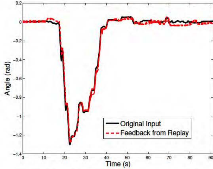
(a) Module 7, “Head to Tail” approach to a 4x4
