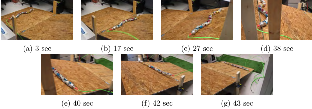
Figure 6.17: For this setup of our test course, the optimal control policy chose a sidewinding parameterization with a wide base for the uphill segments, and quickly transitioned to a zero-amplitude roll for the downhill segments. Note the time each frame was taken, and the difference in speed when moving uphill versus downhill.
