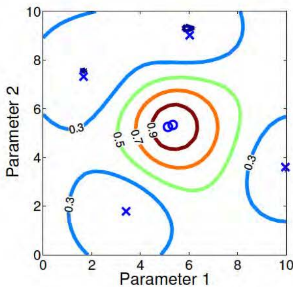
(a) Experiment selection using EI_\pi
