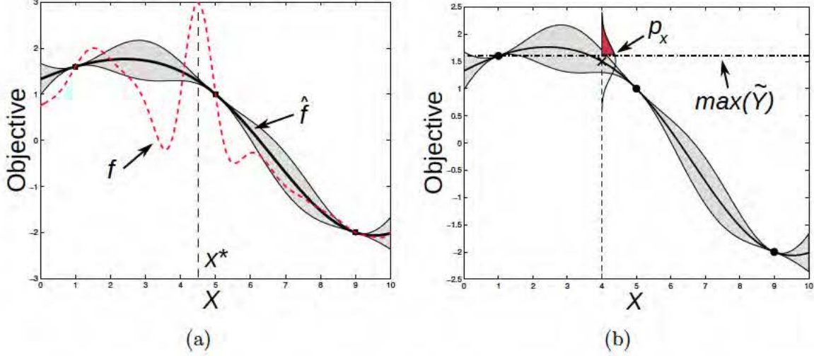
Figure 4.1: (a) The objective function f , surrogate \hat{f} , and maximizer x^* . (b) The best sampled point, \max(\tilde{Y}) , and the predictive distribution for a potential sample location. The red shaded area of this distribution indicates the portion of this distribution considered improvement in this context.
