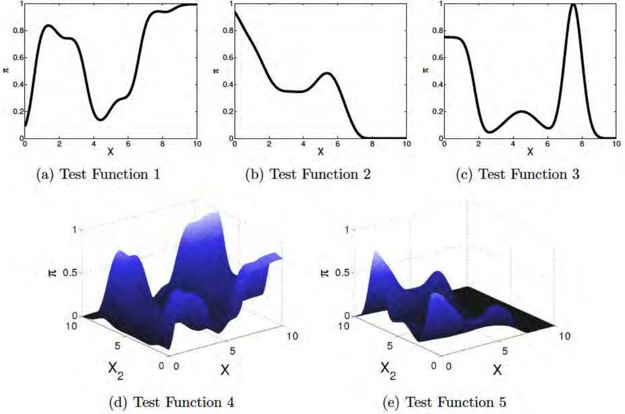
Figure 8.2: A number of synthetic test functions were created for algorithm comparison and validation. The equations for the functions used as benchmark tests in this chapter are given in Appendix A.
