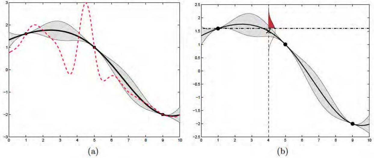
Figure 2.10: (a) A surrogate function (dark line) interpolates sampled points of an unknown underlying function (dotted red line). The surrogate quantifies uncertainty in its prediction, as shown by the shaded region. (b) Experiment selection metrics such as probability of improvement and expected improvement consider the predictive distribution at a potential sample point x (vertical line), compared to the best previous sample (horizontal line).
