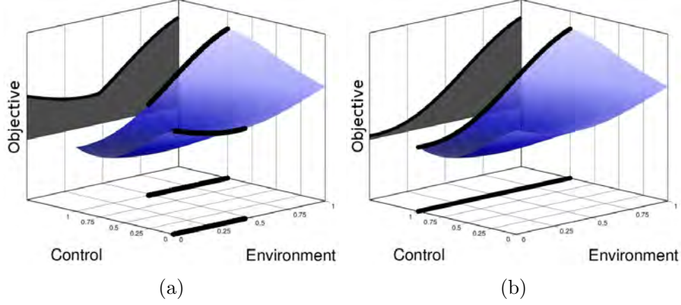
Figure 6.3: An example objective for one dimensional environment and control spaces. The policy \gamma is shown below the function and its performance is projected on the objective/environment plane. The policy score is the integral of this gray shaded region. An optimal policy is illustrated in (a) , presenting the best control parameter for every environment parameter. Note that the policy shown in (b) , which also maps to a control parameter that maximizes the objective at x_e = 1 , results in a significantly lower overall score because of its poorer choices in other regions of the environment space.
