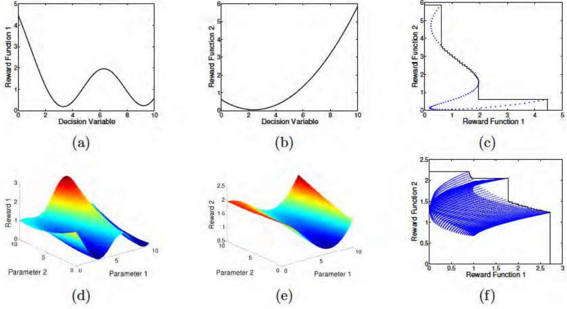
Figure 5.5: Competing test functions created from one dimensional slices ((a) and (b)) and scaled two dimensional regions ((d) and (e)) of the Branin test functions. The plots in (c) and (f) show the resulting objective space projection (blue dots) and Pareto frontiers (black lines).
