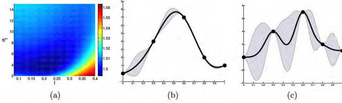
Figure 2.7: (a) A region of the likelihood surface for the two hyperparameters of a squared exponential covariance, \ell and \sigma_f^2 , which contains the maximum likelihood estimate. For numerical optimization reasons, the negative log likelihood is usually considered; this figure is also shown with arctan scaling to make the contours more apparent. (b) The GP posterior using the maximum likelihood hyperparameters, \ell = 0.21 and \sigma_f^2 = 3.6 . (c) The GP posterior using a set of non-maximum likelihood hyperparameters, \ell = 0.082 and \sigma_f^2 = 2.1 .
