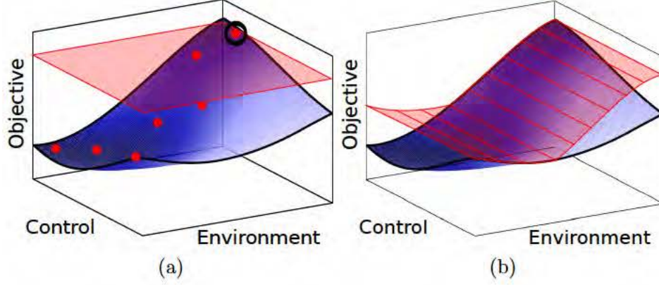
Figure 6.5: (a) Standard EI measures improvement over the best sampled experiment, the value of which is represented by the horizontal red plane. This biases against sampling in difficult environments, such as those towards the left of the environment axis. (b) Unbiased expected improvement reduces this bias by measuring improvement over the maximum of the estimated objective for each environment ; the objective is shown below in blue, and the maximum is shown above in red.
