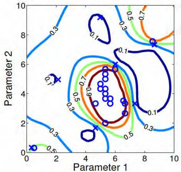
(b) Experiment selection using EI_\pi and ignoring areas of high certainty
