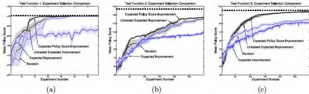
Figure 6.9: Comparison of algorithms on the three analytic test functions shown in Fig. 6.7. Each algorithm was run 10 times, and the scores averaged. The dotted black line represents the best possible policy for that function. EPSI performed best, followed by UEI. Expected improvement selected initial experiments intelligently, but its inherent bias lead to poor overall performance. Random point selection suffered from no such bias, and resulted in steady policy score improvement with increasing experiments. Each line represents the mean of 20 trials, and the shaded regions indicate \pm 1 standard error.
