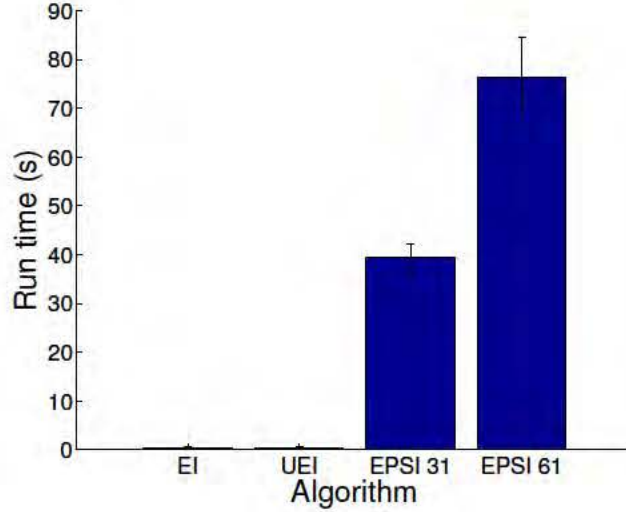
Figure 6.8: The average run time for iterations 31-40 of three separate runs of standard EI, UEI, and EPSI (with numerical integral resolutions of 31 and 61), using the MATLAB code provided with this thesis run on a 2.8 GHz Core i7-2640M processor. For the simple implementations used, the run time of UEI is inconsequential compared with EPSI, and doubling the numerical integral resolution of EPSI doubles the computational time (as would be expected). The error bars provide a 95% confidence interval for each algorithm.
