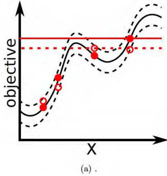
Figure 4.7: (a) If function evaluations (circles; underlying function values are dots) are taken from a noisy function (solid curve with 1-\sigma variance as dashed lines), the maximal sample (dashed horizontal line) does not necessarily correspond to the value or location of the underlying function's maximum at the sampled locations (solid horizontal line).
