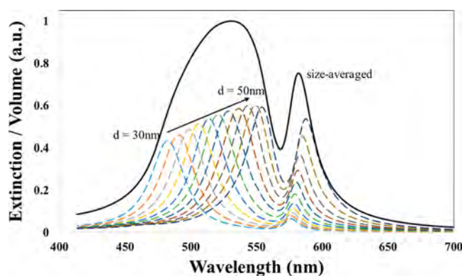
Figure 5. Average extinction cross-section per unit volume of a distribution of PIC-coated silver platelets, computed using the boundary element method. The distribution of experimental sizes was modeled by fixing the thickness of the platelets at 10 nm and varying the diameter d from 30 to 50 nm. A thickness of 8 nm was assumed for the PIC coating. The PIC permittivity is modeled by the complex frequency-dependent dielectric function described in the text with an oscillator strength of f = 0.02 and a line width \hbar\gamma = 21 meV. The single-particle data (dashed lines, scaled up by a factor of 3) shows significant transparency dips when the exciton and plasmon resonances are close. In the average extinction over an equal distribution of the sizes (solid line), the transparency dip persists due to the relatively small variation in the transparency energy.
