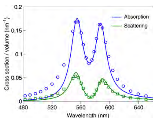
Figure 6. Comparison between temporal coupled-mode theory and BEM. Symbols are calculated using BEM for a platelet with core thickness of 10 nm, core diameter of 50 nm, and a 8 nm thick layer of PIC coating. Lines are modeled by temporal coupled-mode theory using \omega_1 = 2.24 eV, \gamma_1 = 10 meV, \xi_1 = 31 meV for the plasmonic resonance and \omega_2 = 2.11 eV, \gamma_2 = 6.3 meV, \xi_2 = 27 meV for the exciton resonance.
