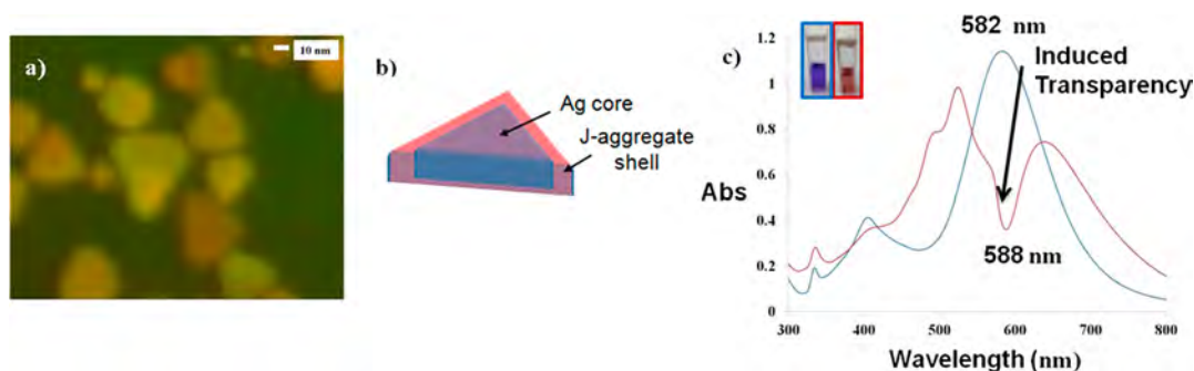
Figure 2. (a) TEM image of silver nanoplatelets (scale bar = 10 nm). (b) Schematic of a bilayered nanoplatelet, consisting of a silver nanoplatelet core and a PIC J-aggregate shell. (c) Absorption spectra of a solution containing 0.1 mg/mL silver nanoplatelets in water (blue curve) and a solution containing 2 mL of 0.1 mg/mL silver nanoplatelet solution mixed with 100 \mu L of 0.02 mM PIC (red curve). An induced transparency is observed. The inset (upper left) provides images of the silver nanoplatelet and silver nanoplatelet/PIC solutions. The optical path length for all spectral measurements was 10 mm.
