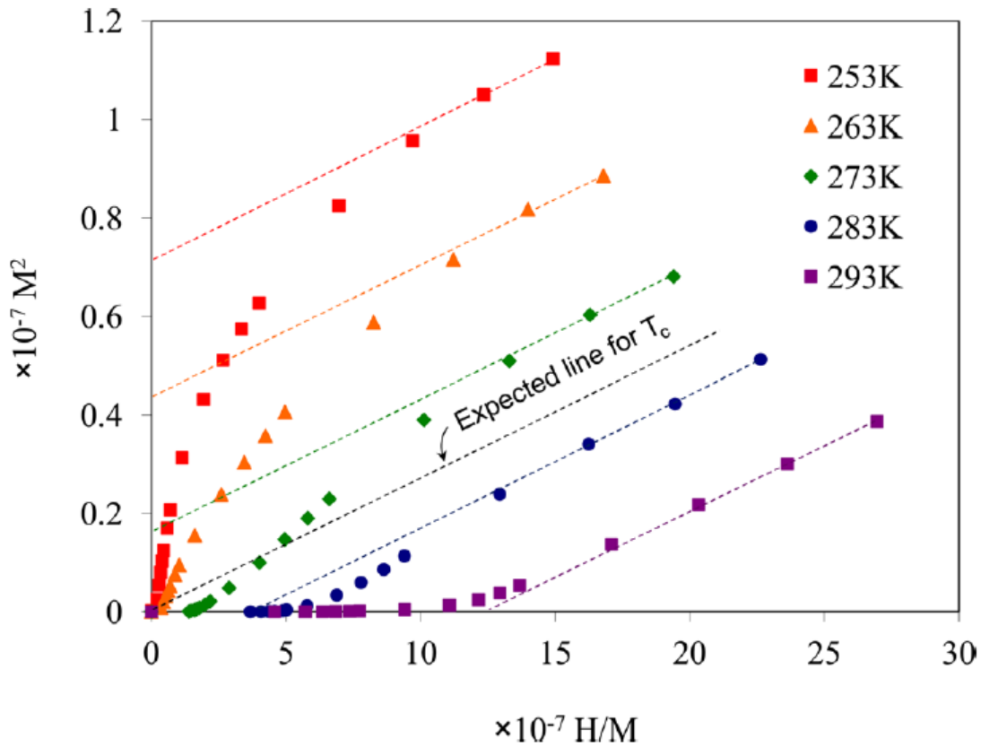
Figure 6: Arrott plot for 25 nm sputtered Gd thin film
