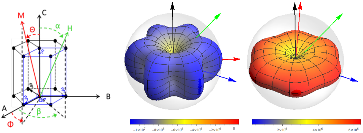
Figure 13: Left - Crystal orientation showing the applied field vector (H) in green and its corresponding polar ( \alpha ) and azimuthal ( \beta ) angle as well as the red magnetization vector (M) and its polar ( \theta ) and azimuthal ( \phi ) angles. In addition the black and blue arrows indicate the C and B axes respectively. Middle – The energy surface of a NdCo 5 sphere at T=255K with a 100 Oe field applied at \alpha = 45^\circ and \beta = 45^\circ . Right – The energy surface of NdCo 5 at 286K with the same applied field parameters.
