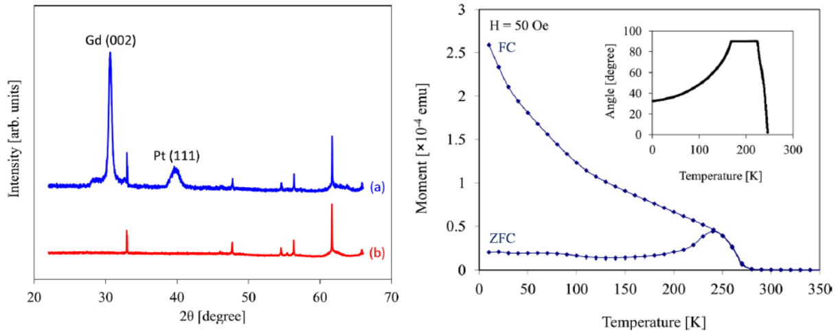
Figure 5: Left – XRD results for 20 nm sputtered Gd thin-film (a) and the Silicon substrate (b). Right – ZFC-FC results for a temperature range of 10 to 350 K.
