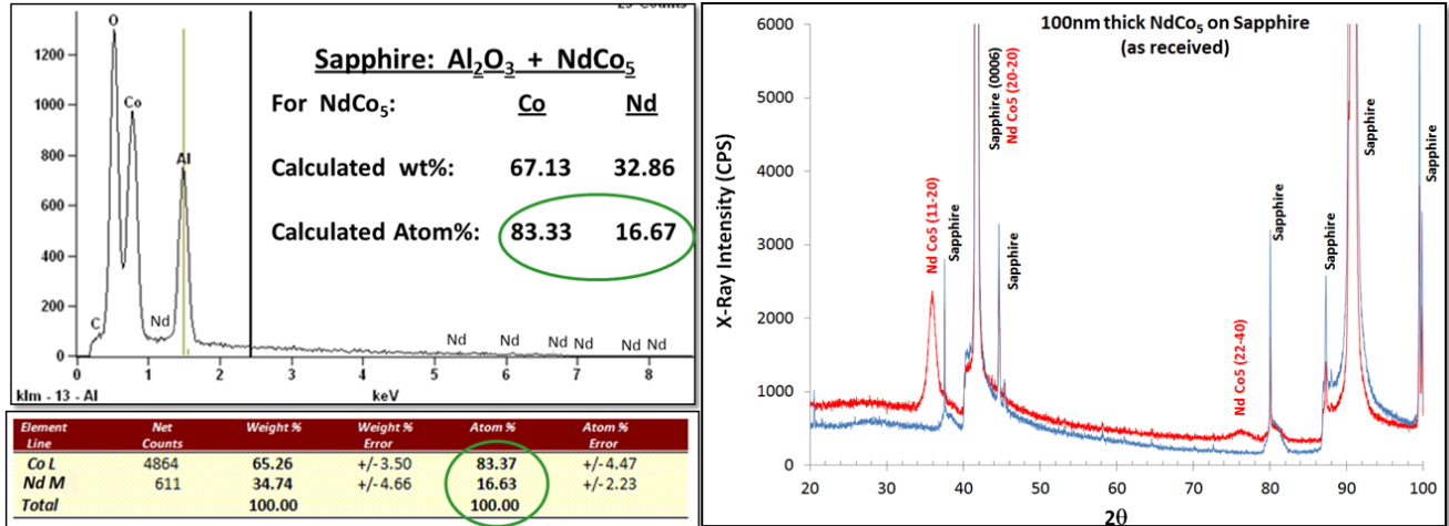
Figure 18: Left – EDS of 100 nm of NdCo 5 film on sapphire. Right – XRD of 100 nm NdCo 5 film on sapphire.
