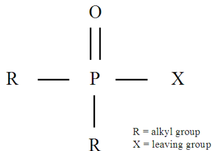
Figure 3. Basic Structure of Nerve Agent (Canard, 2006:87)
