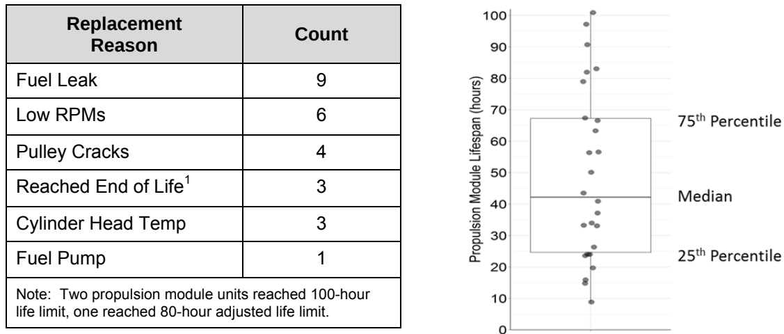
Figure 4-3. Reasons for Propulsion Module Replacement and Distribution of Lifespans
