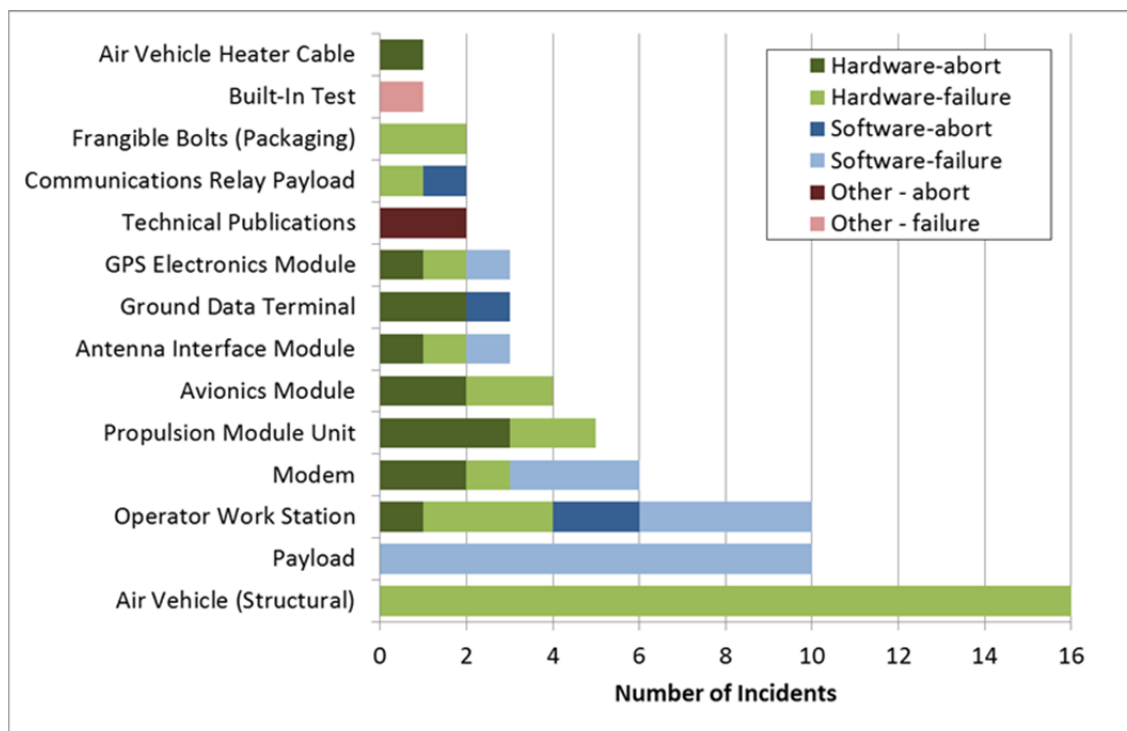
Figure 4-2. Failure chargeability
