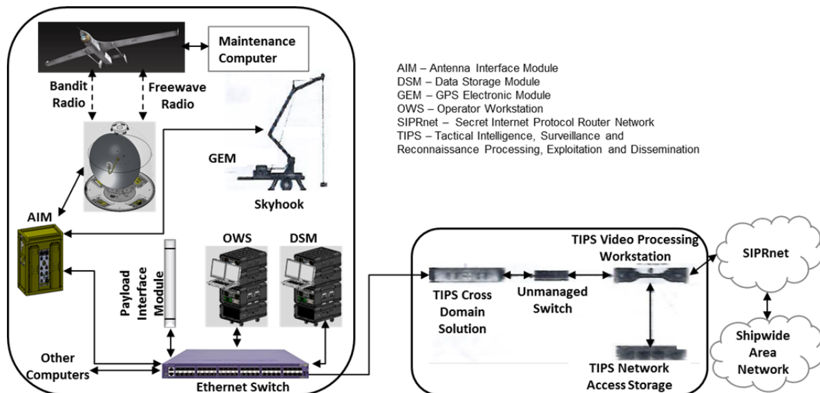
Figure 2-1. RQ-21A Architecture
