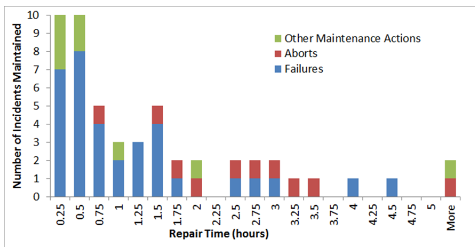
Figure 4-8. Distribution Twentynine Palms Repair Times
