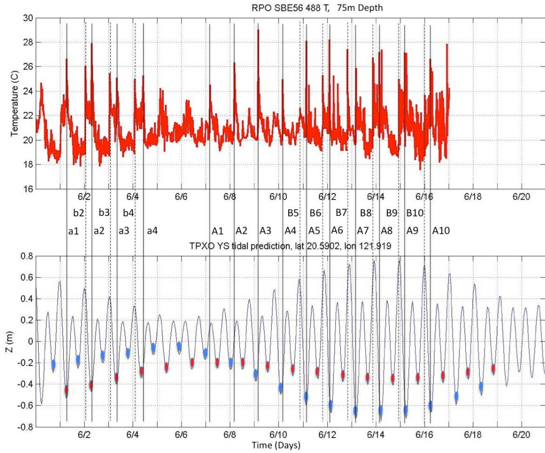
Figure 2. Temperature from 75 m depth on mooring RPO (water depth 266 m) plotted over the tidal heights in the Luzon Strait as generated from the TPXO global tidal model. The temperature time series has been lagged back 48.5 hours to allow for the propagation time from the strait to the mooring. The blue and red dots illustrate how the stronger beat during the first fortnight became the weaker beat during the second fortnight. Vertical solid lined indicate a-waves, and dotted lines indicate b-waves. For details see text.
