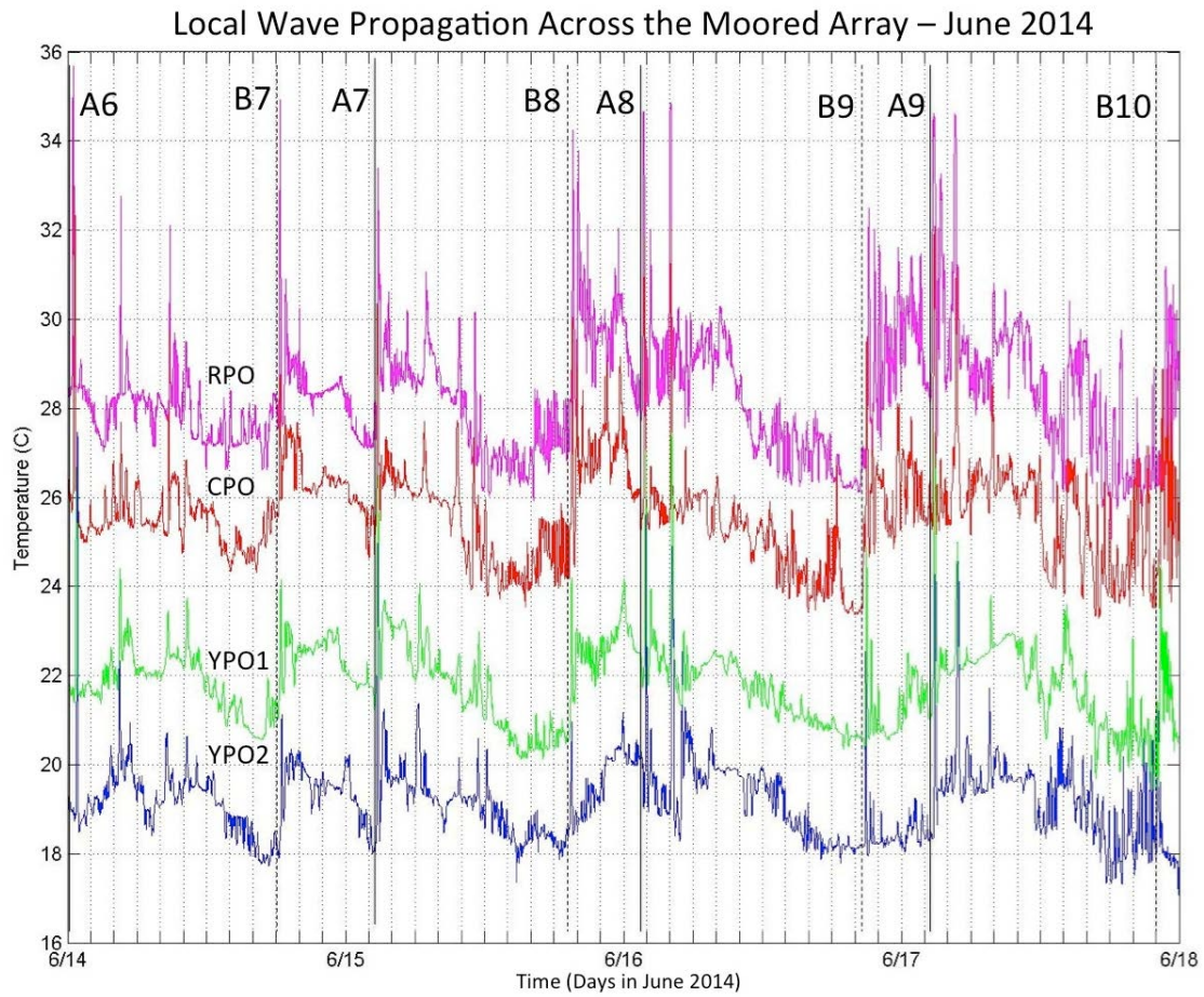
Figure 3. Temperature time series near 75 m depth from each of the four moorings spanning the June 2014 moored array. Each time series has been lagged to allow for the propagation time between moorings, and offset by 2°C for clarity. The (a, b) waves are indicated by a (solid, dashed) vertical line. This figure represents a time of strong generating tides in the spring/neap cycle.
