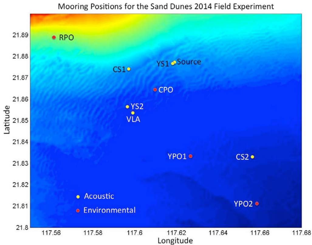
Figure 1. Mooring positions on bottom topography for the ONR Sand Dunes June 2014 moored array in the northeastern South China Sea. Maximum relief in the region of the highest dunes was 16 m near CPO. YPO2 lies ahead of the dune field as the wave travels, YPO1 and CPO are in the dune field, and CPO is just past the dune field.
