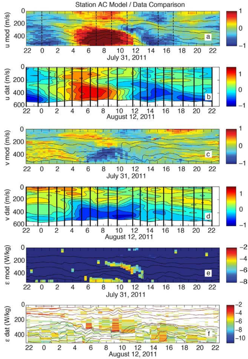
Figure 3. Model (MITgcm) / data comparisons over the northern Heng-Chun Ridge. July 31 and August 12 are from the same position in the tidal cycle. The u -component (a, b), v -component (c, d), and turbulent dissipation (e, f) are compared.
