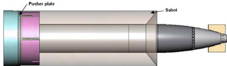
Fig. A-1 Projectile in obturator-pusher plate-sabot assembly
