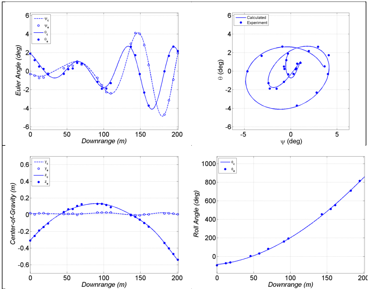
Fig. C-7 Measured and calculated motion for TRN39361
