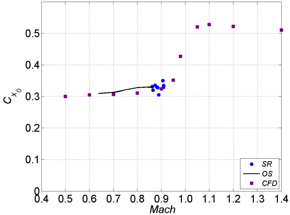
Fig. 17 Zero-yaw axial force coefficient
