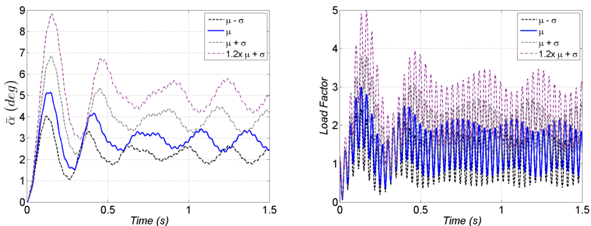
Fig. 23 Effects of uncertainty on maneuverability of baseline and enhanced canard configurations
