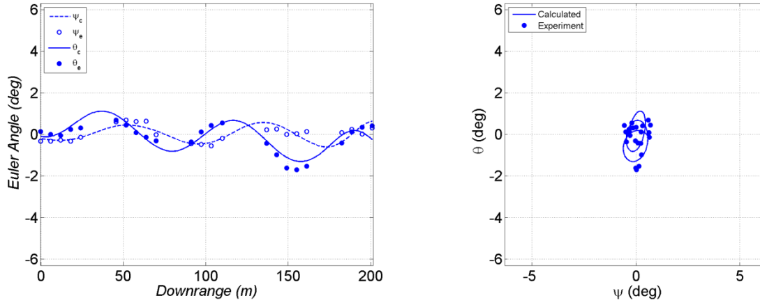
Fig. 10 Angular motion for TRN39363
