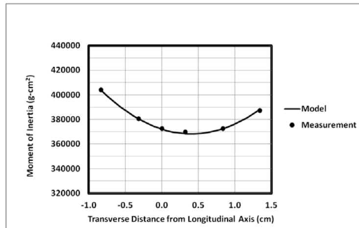
Fig. B-1 Axial moment of inertia about longitudinal axis and lateral center-of-gravity data
