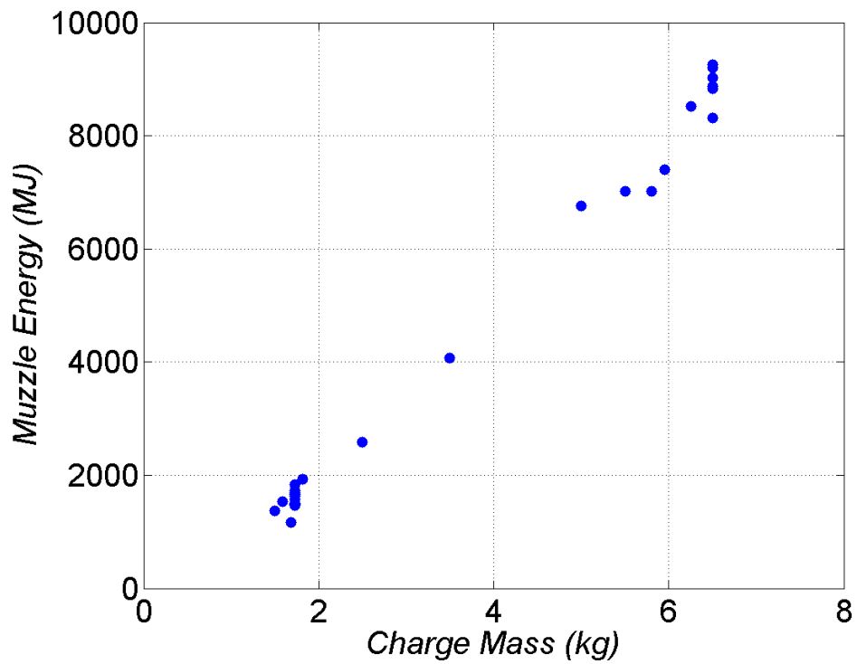
Fig. A-3 Relationship between charge mass and muzzle energy
