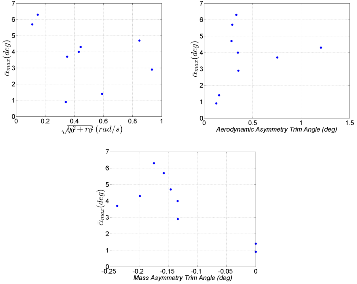
Fig. 16 Correlations between maximum total angle of attack and tip-off, aerodynamic trim, and mass trim
