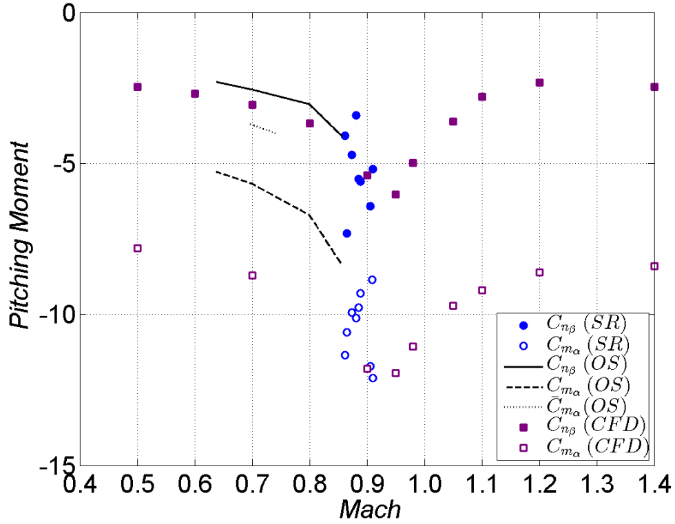
Fig. 18 Pitching moment coefficient
