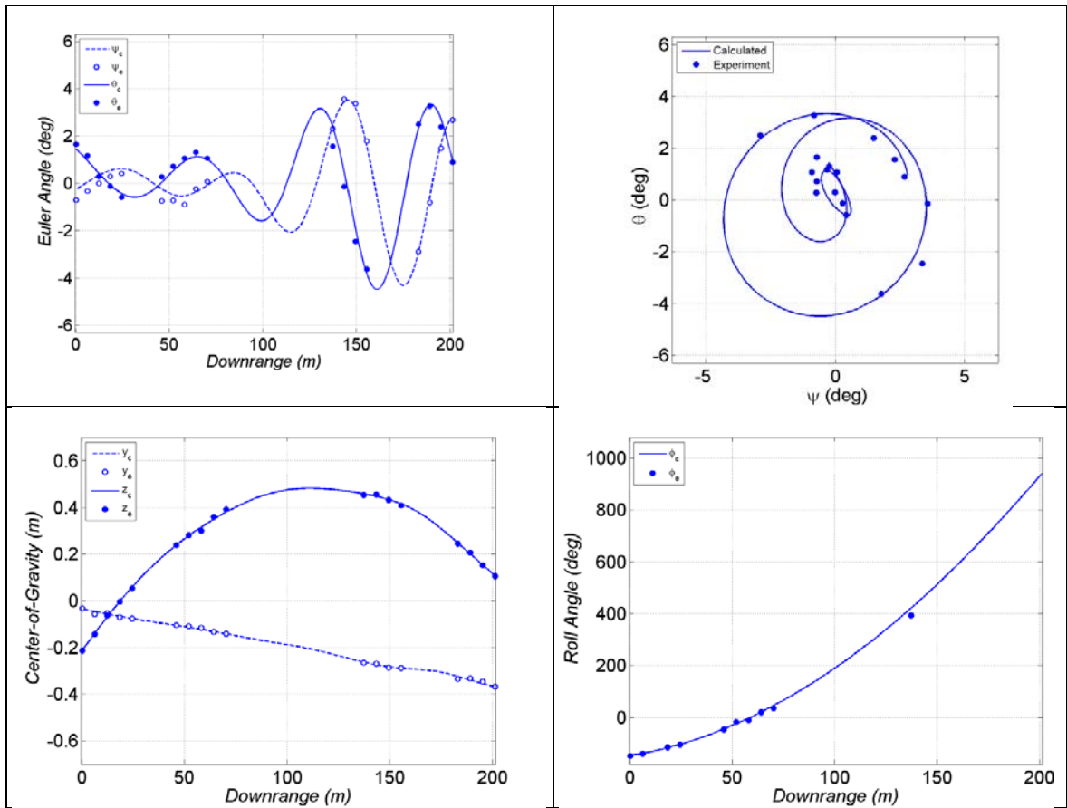
Fig. C-1 Measured and calculated motion for TRN39043
