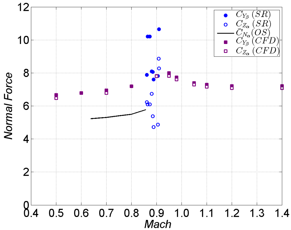
Fig. 19 Normal force coefficient
