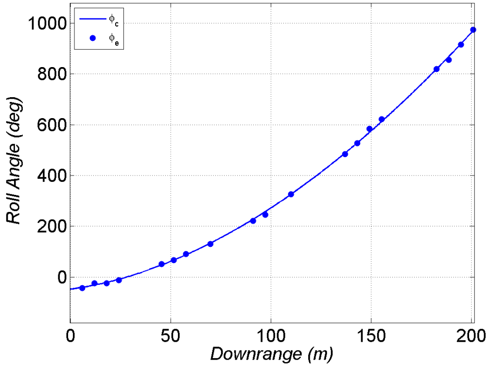
Fig. 12 Roll motion for TRN39363
