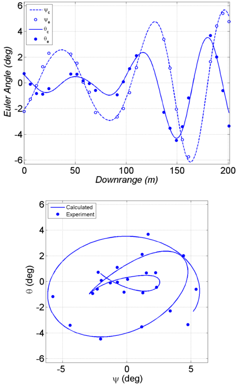
Fig. 7 Angular motion for TRN39362
