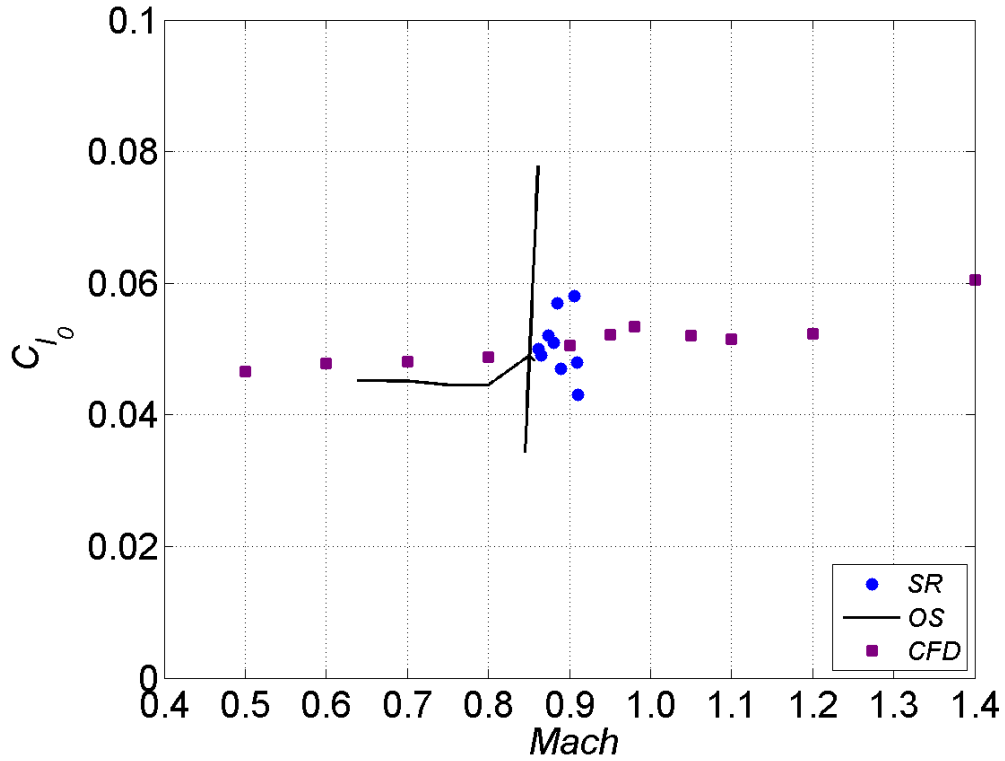
Fig. 21 Static roll moment coefficient
