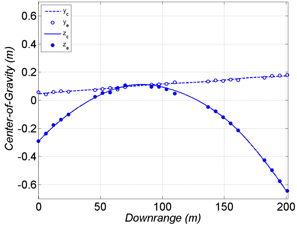
Fig. 11 Center-of-gravity motion for TRN39363
