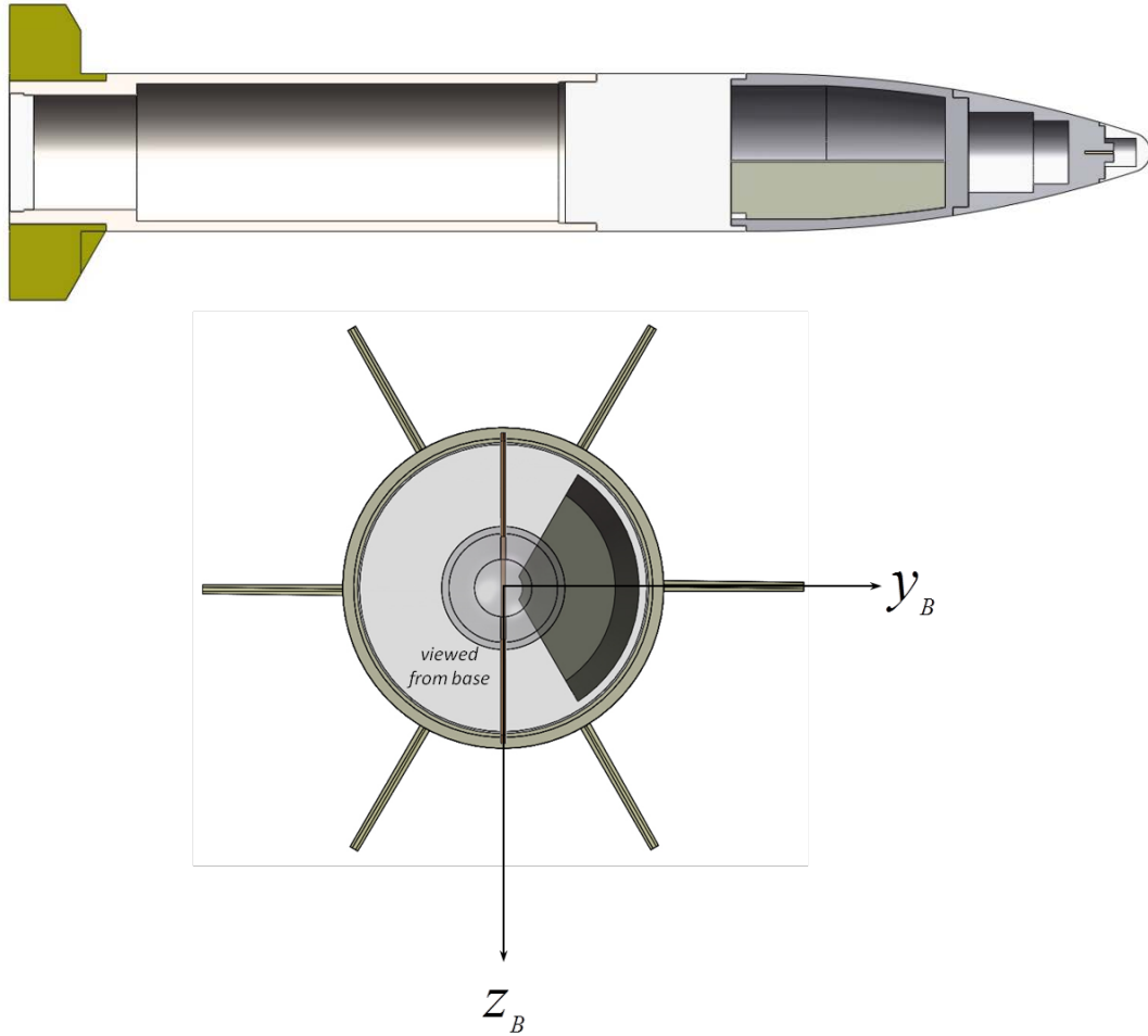
Fig. 2 Cutaway of projectile with internal asymmetry: longitudinal (top) and axial (bottom)
