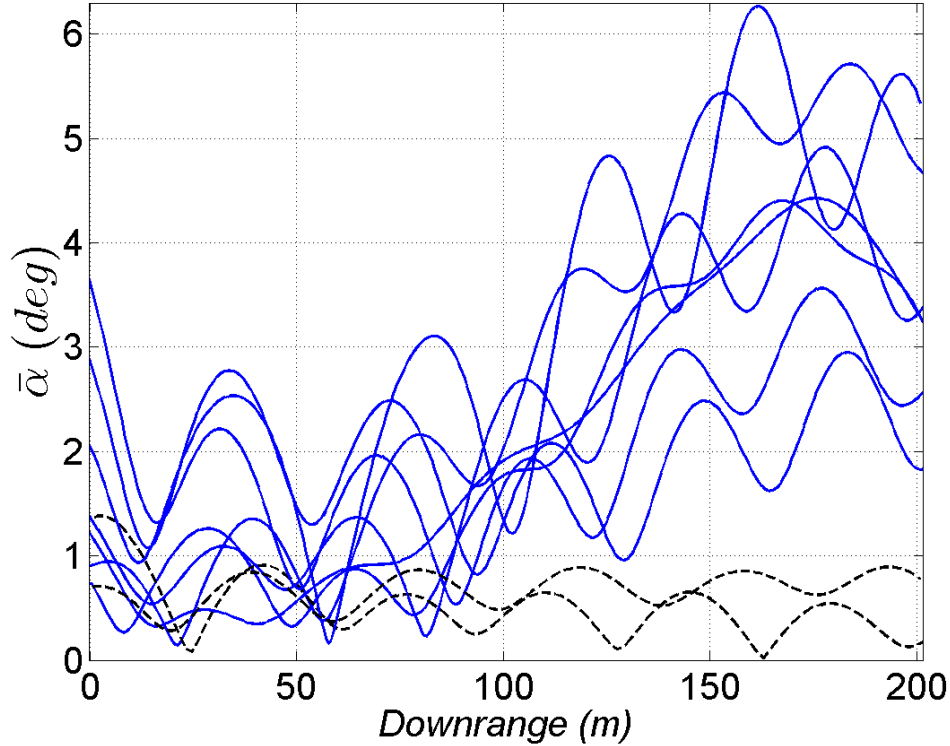
Fig. 13 Total angle-of-attack history for all flights
