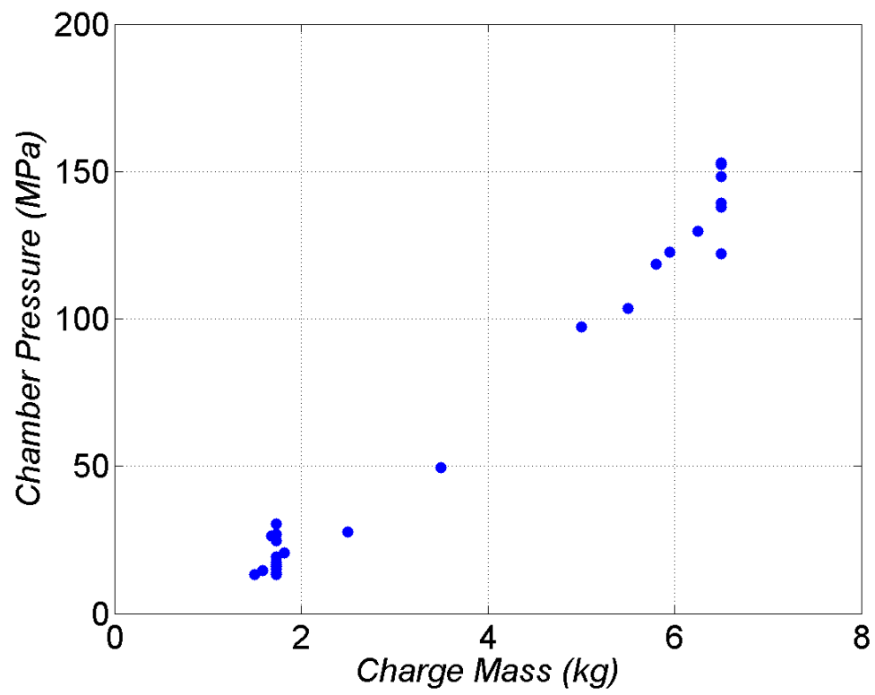
Fig. A-4 Relationship between charge mass and chamber pressure
