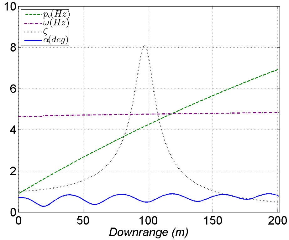
Fig. 15 Resonance for TRN39363
