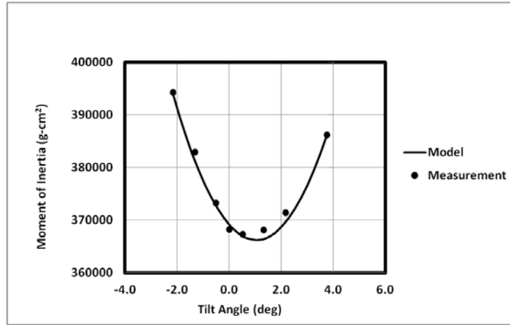
Fig. B-2 Axial moment of inertia about principal axis and tilt angle of principal axis
