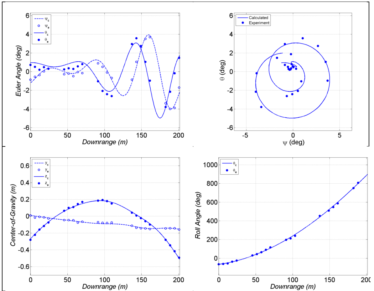
Fig. C-4 Measured and calculated motion for TRN39319
