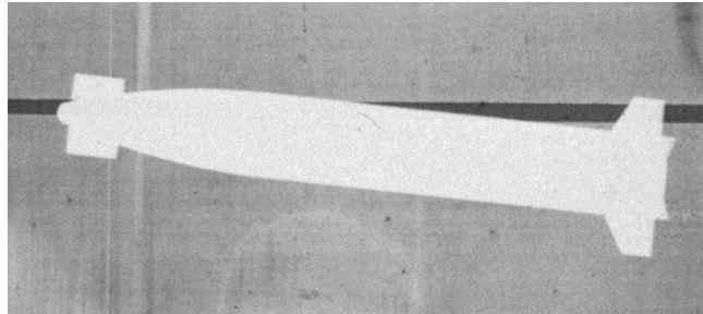
Fig. 6 Shadowgraph of model during free-flight experiment
