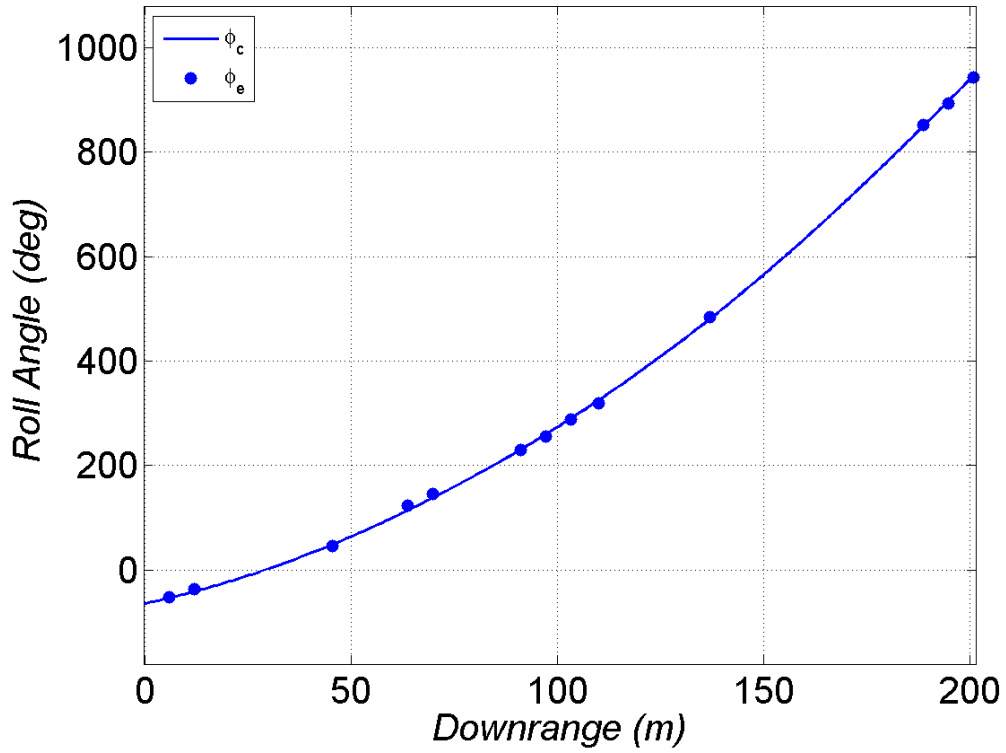
Fig. 9 Roll motion for TRN39362
