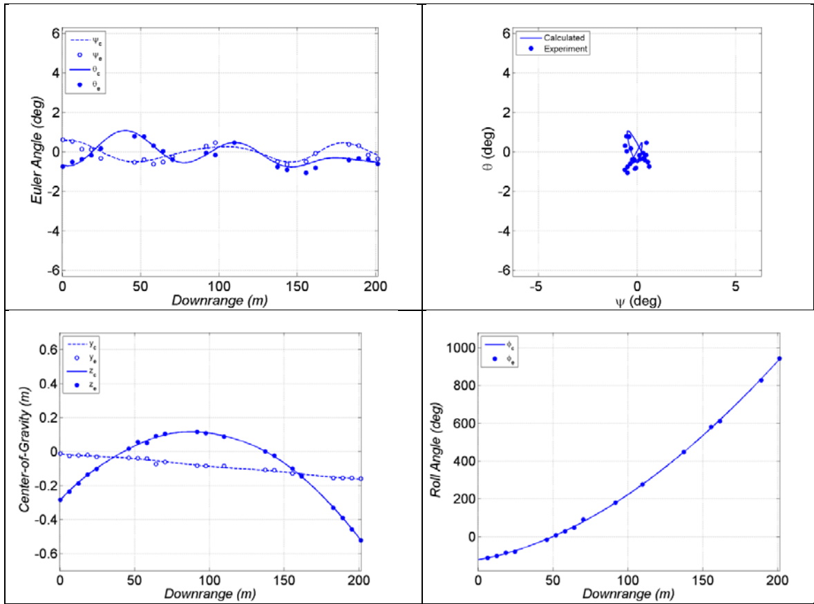
Fig. C-3 Measured and calculated motion for TRN39045
