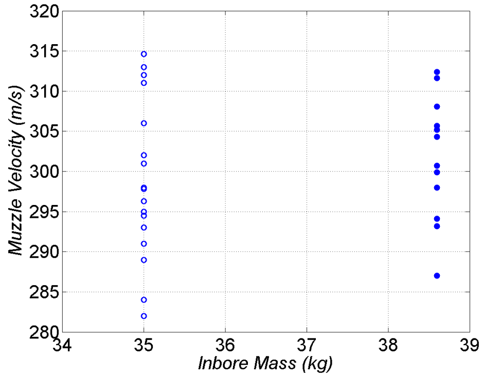
Fig. A-2 Relationship between in-bore mass and muzzle velocity for 1.73 kg of M2 propellant
