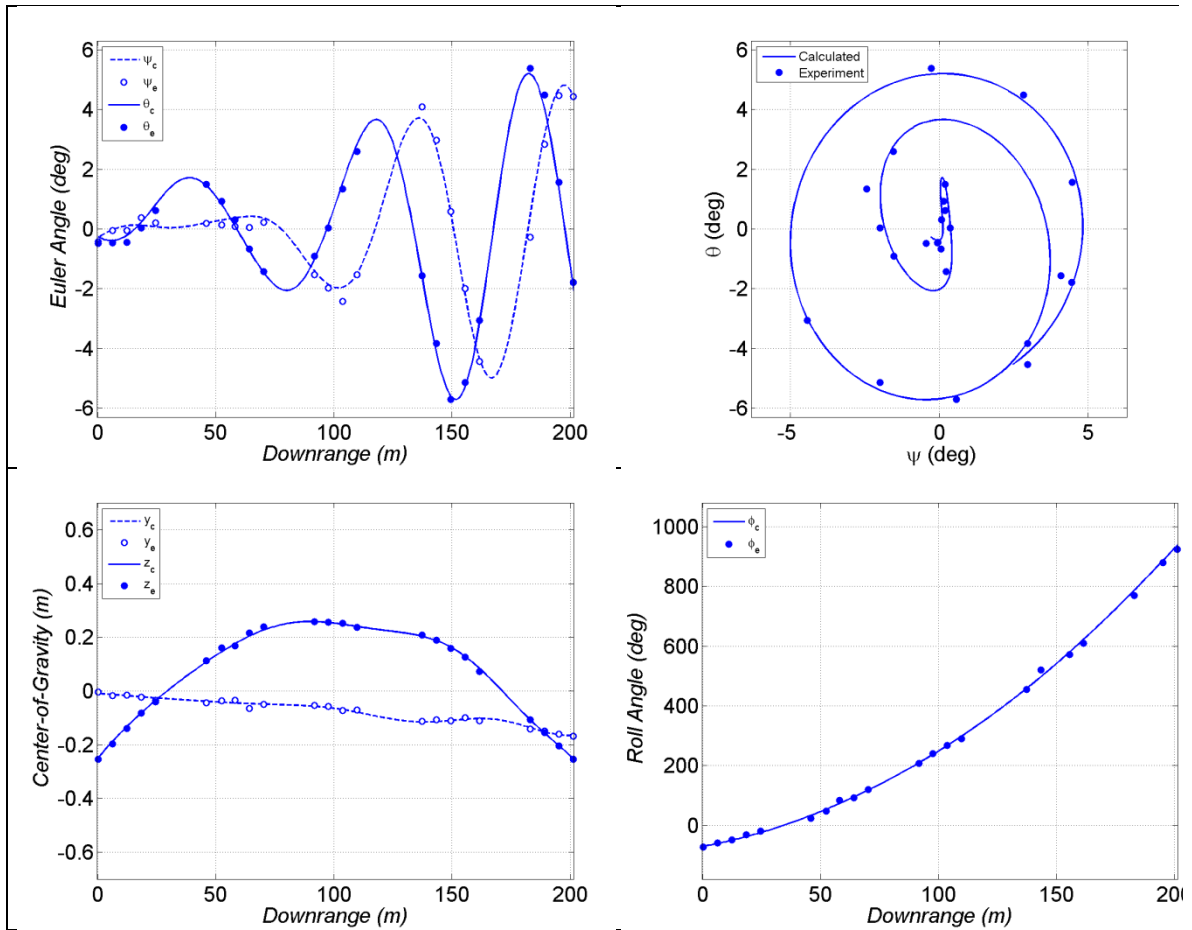
Fig. C-2 Measured and calculated motion for TRN39044
