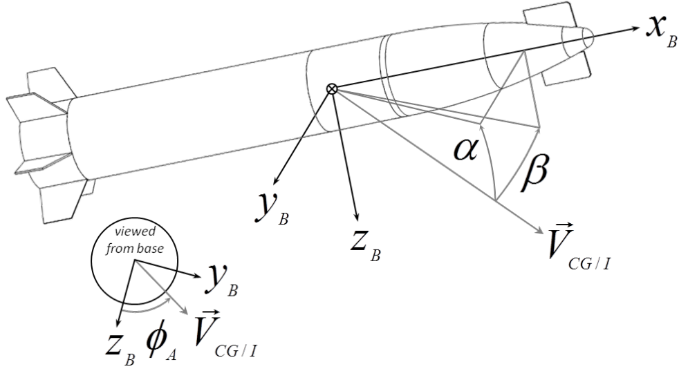
Fig. 4 Coordinate system definitions for aerodynamic angles
