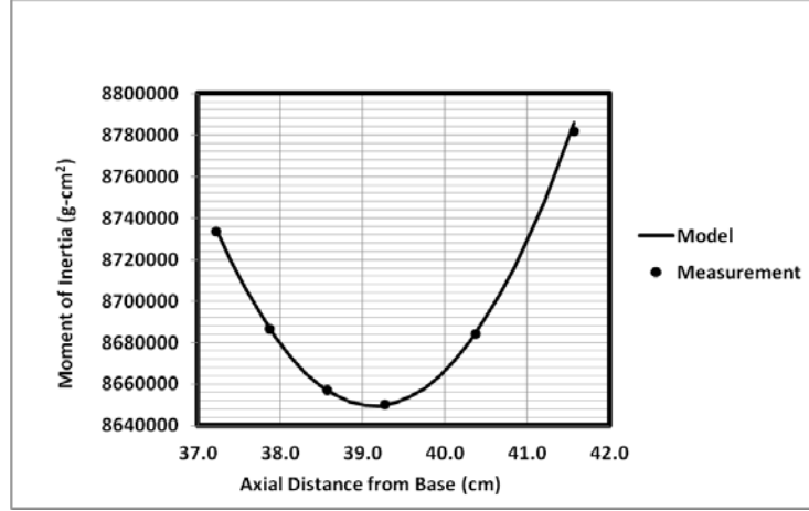
Fig. B-3 Transverse moment of inertia and longitudinal center of gravity
