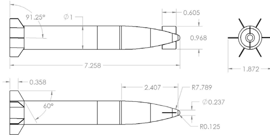
Fig. 1 Projectile dimensions (length dimensions measured in calibers)
