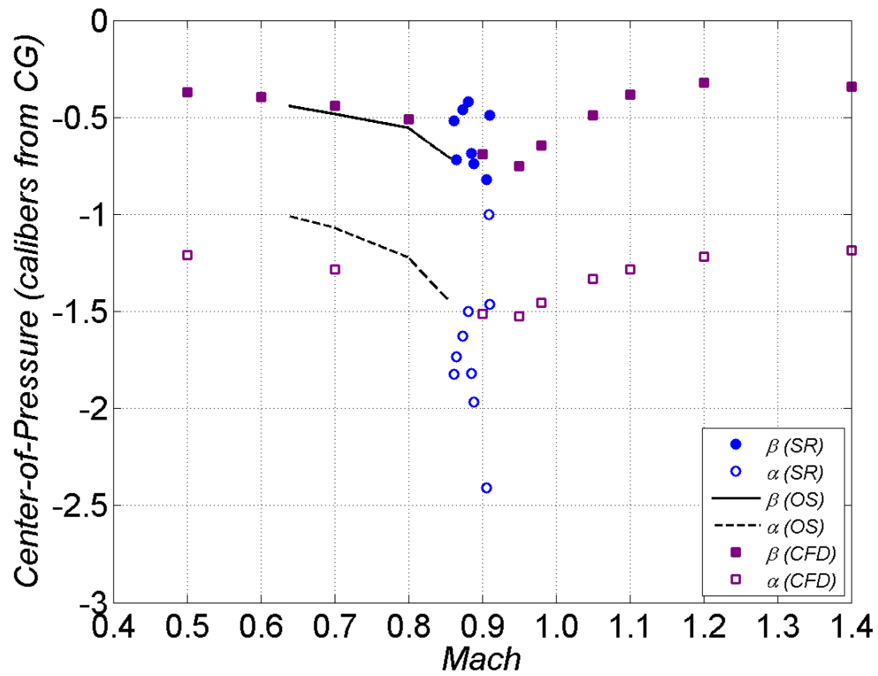
Fig. 20 Center of pressure
