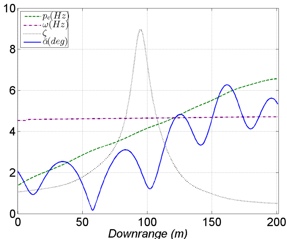
Fig. 14 Resonance for TRN39362
