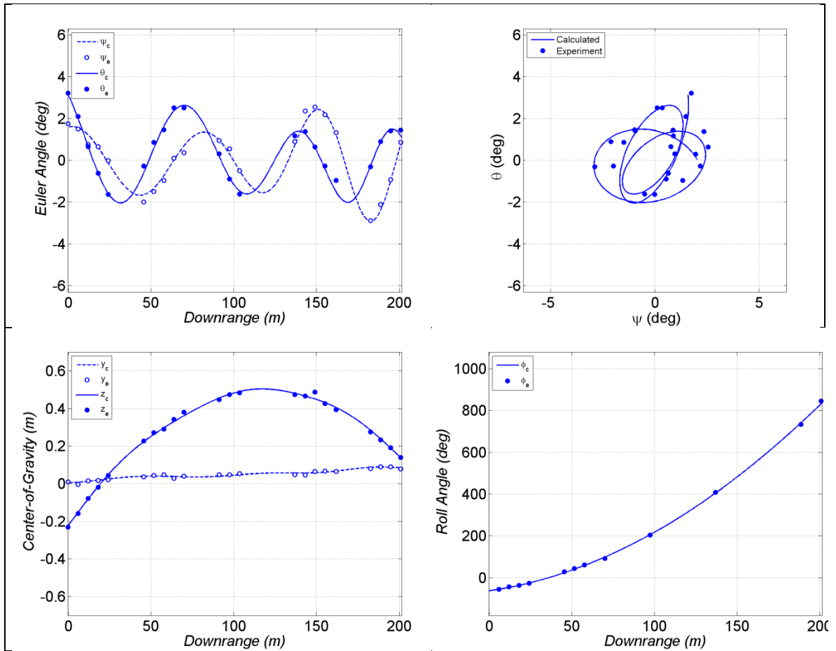
Fig. C-5 Measured and calculated motion for TRN39320
