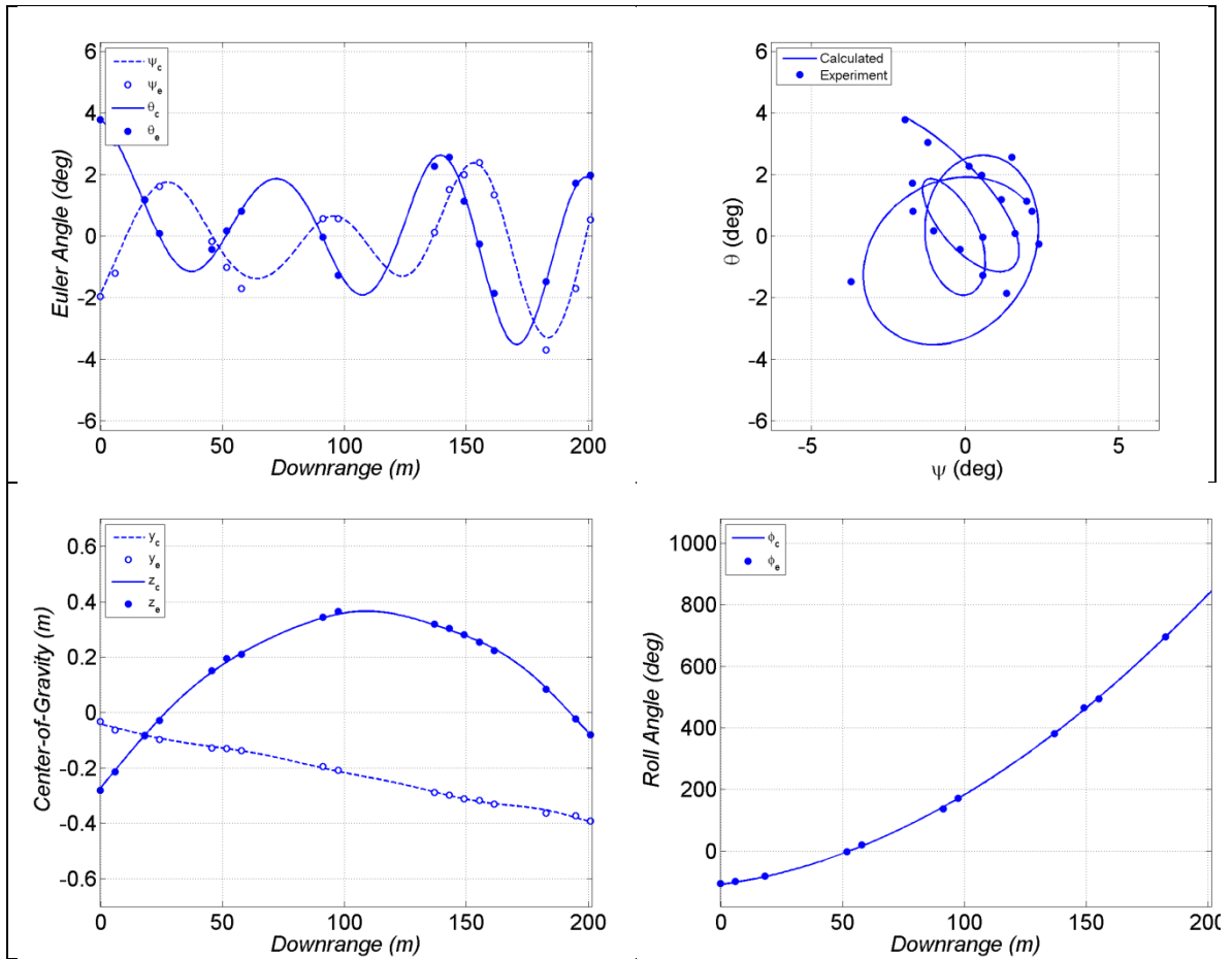
Fig. C-6 Measured and calculated motion for TRN39360
