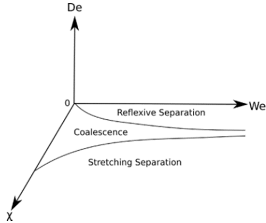
Figure 5-1: Representative viscoelastic collision outcome parameter space with the plane De=0 representing a Newtonian fluid.
