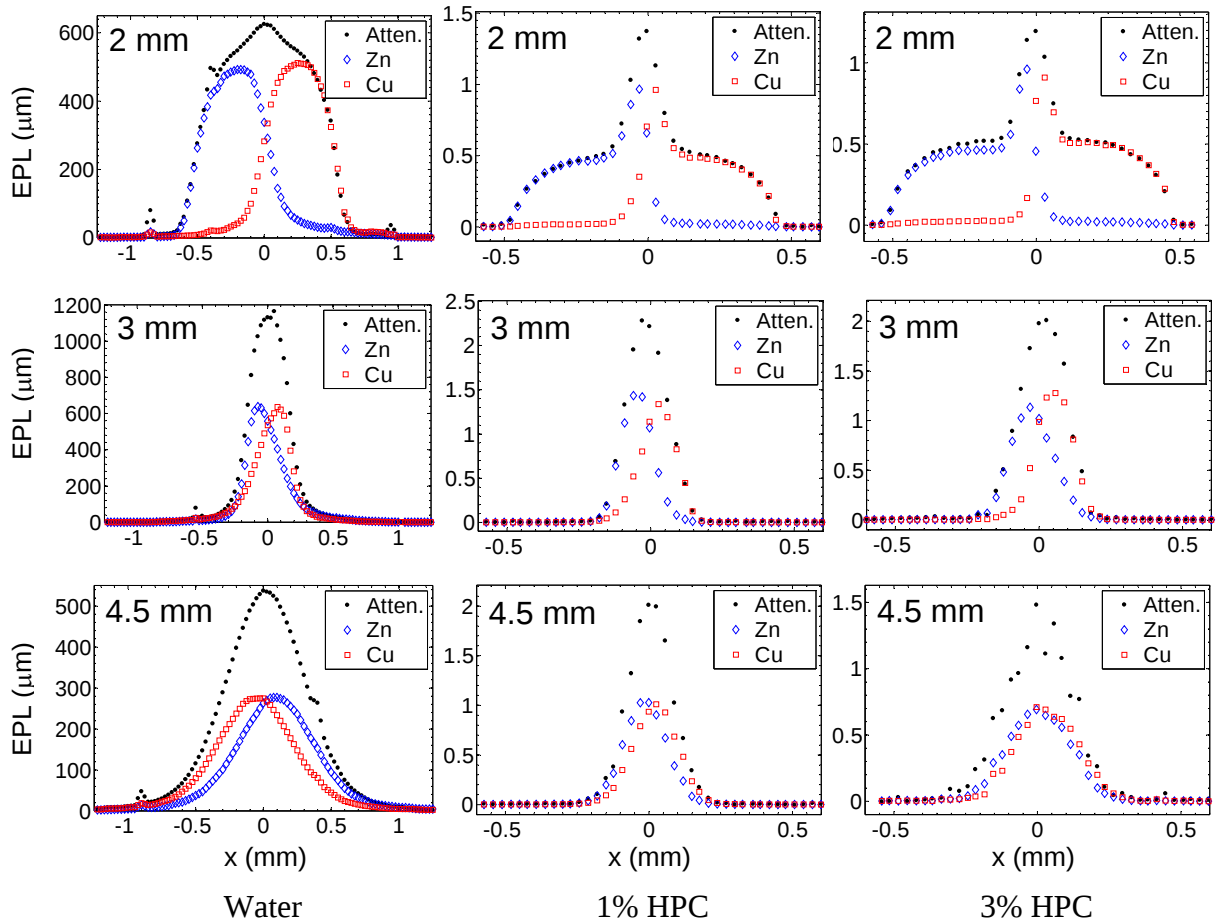
Figure 4-11: Comparison of mixing behavior for water and gels with two different concentrations of 1% and 3% HPC.
