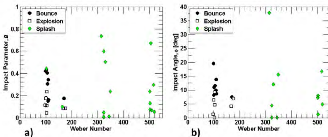
Figure 6-7. Impact types plotted against two measures of impact geometry, impact parameter a) and impact angle b) vs. Weber number. All data from MMH/WFNA tests.
