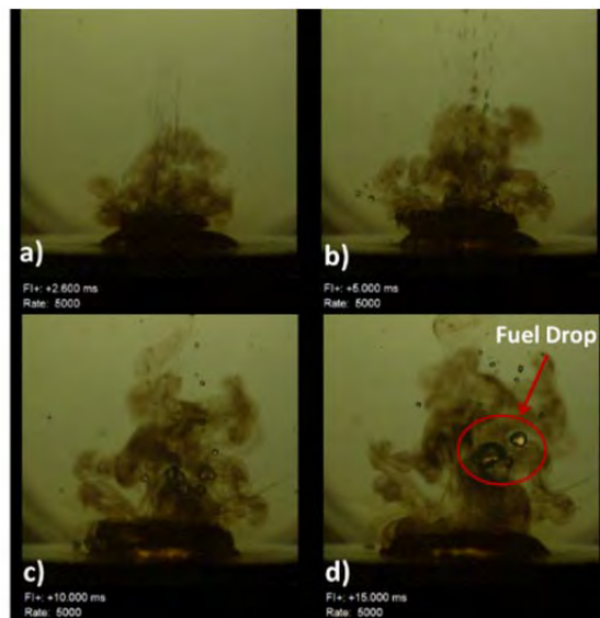
Figure 6-3. Drop of MMH bouncing out of a pool of RFNA. d = 2.3 \text{ mm} , v = 1.3 \text{ m/s} , We = 99 , pool volume = 60 \mu\text{L} . All times are referenced to contact.
