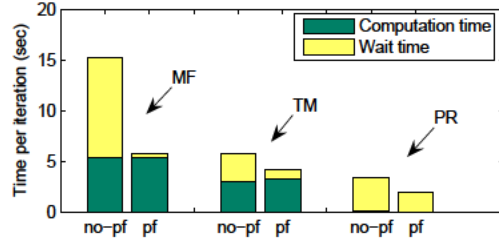
Figure 4.14: Effect of prefetching on computation time and wait time.
