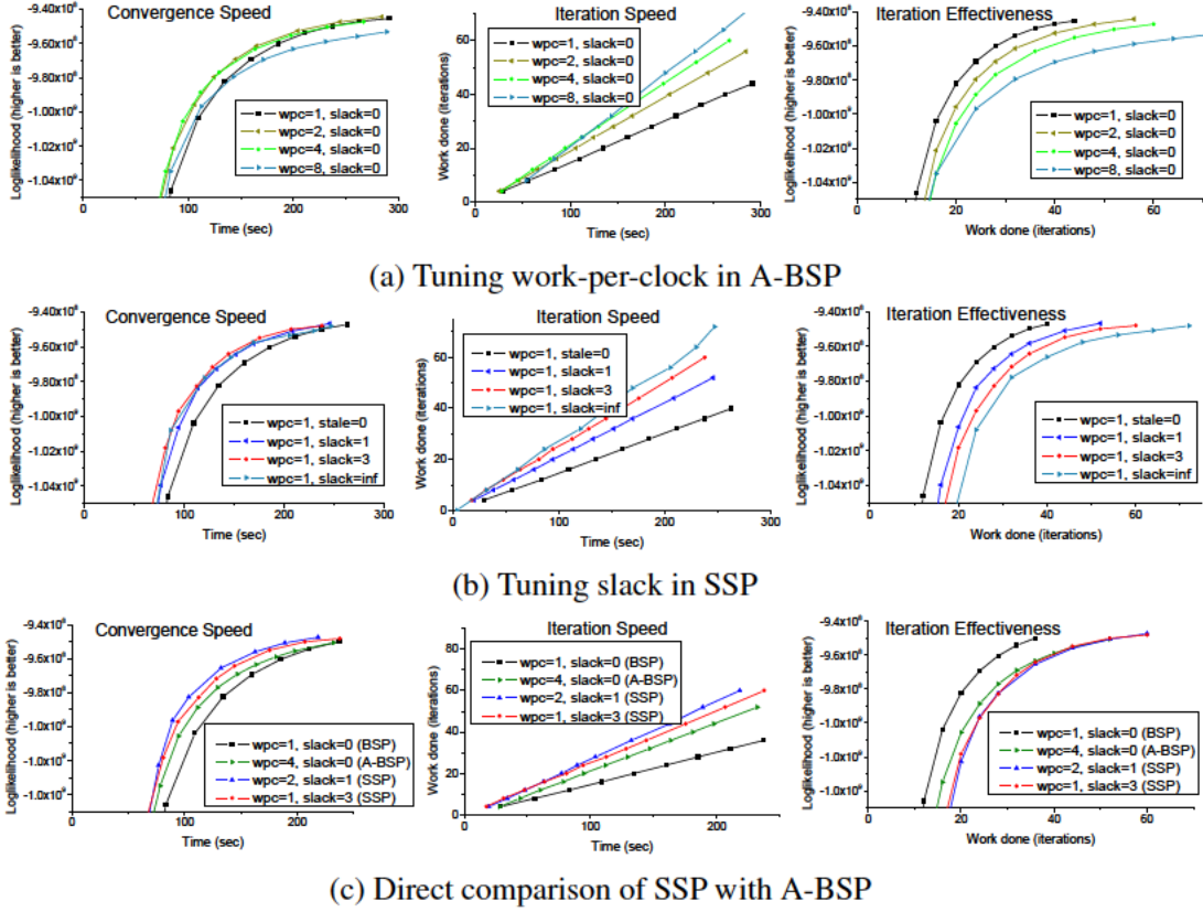
Figure 4.7: Different ways of exploiting data staleness in Topic Modeling. A-BSP adjusts the amount of work done in each clock period, while SSP adjust the "slack", i.e. how many clocks a thread can get ahead of others before it will be blocked.
