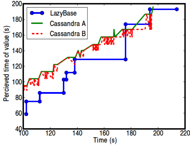
Figure 3.9: The effective timestamp of the returned rows at query time. Differences between Cassandra row A and Cassandra row B indicate inconsistencies between the rows at query time. Dips in the timestamps of a single row indicate violations in monotonic read consistency.
