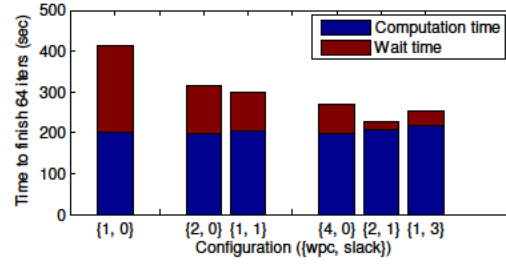
Figure 4.11: Computation time vs wait time for the Topic modeling application. Each bar represents a different staleness setting. The notation \{X,Y\} indicates WPC=X , slack=Y . Each group of bars has the same effective staleness.
