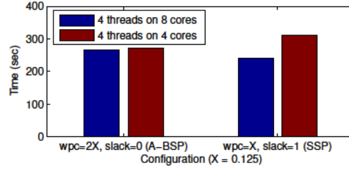
Figure 4.13: CPU overhead of communication: the blue bar represents a configuration where all threads, including communication threads, run on their own core. The red bar represents a CPU-constrained configuration, where communication threads share cores with computation threads. The relative increase between blue and red indicates the overhead of communication. This overhead is negligible for A-BSP, but significant for SSP.
