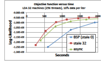
Topic Modeling 32 VMs, 10% minibatches
