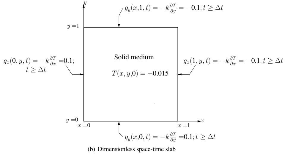
Figure 71: 2D solid-liquid phase transition: space-time slab, boundary conditions, and initial condition
