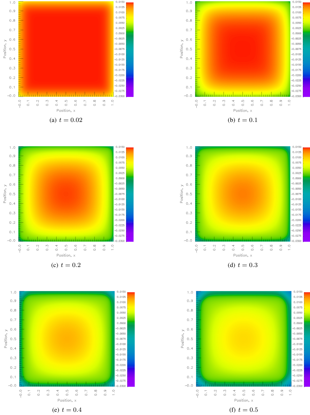
Figure 67: Model Problem 4: Evolution of temperature for liquid-solid phase change in \mathbb{R}^2 , C^{00}(\bar{\Omega}_{\mathbf{a}t}^e) , p = 3 , \Delta t = 0.0025 for 0 \leq t \leq 0.02 and \Delta t = 0.01 for t \geq 0.02
