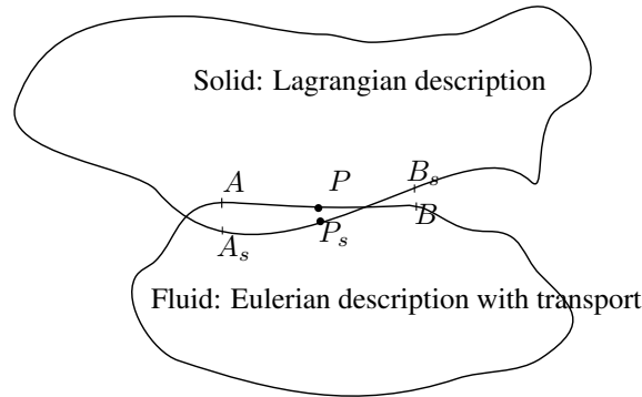
(b) Fluid-solid interaction with boundary AB at time t , current configuration
