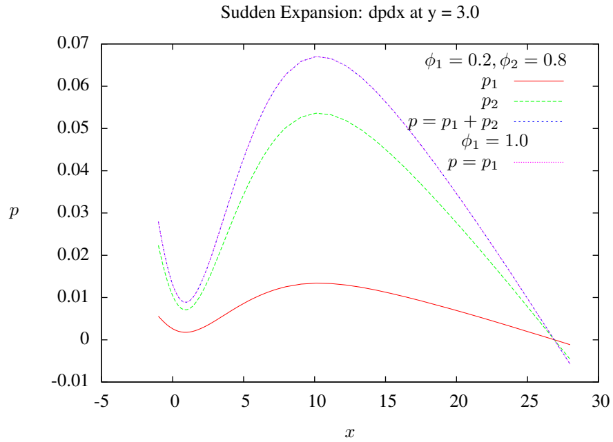
Figure 107: Pressure at top boundary ( y = 3, -1 \leq x \leq 28 ): fluid 2 same as fluid 1, \phi_1 = 0.2, \phi_2 = 0.8
