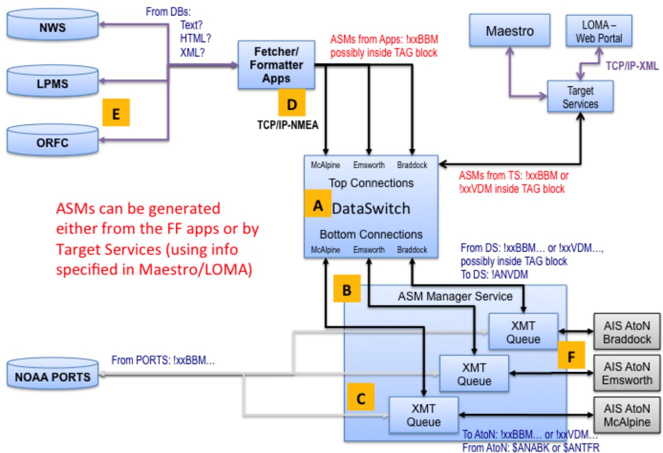
Figure 8. USACE AIS transmit test data flow.
