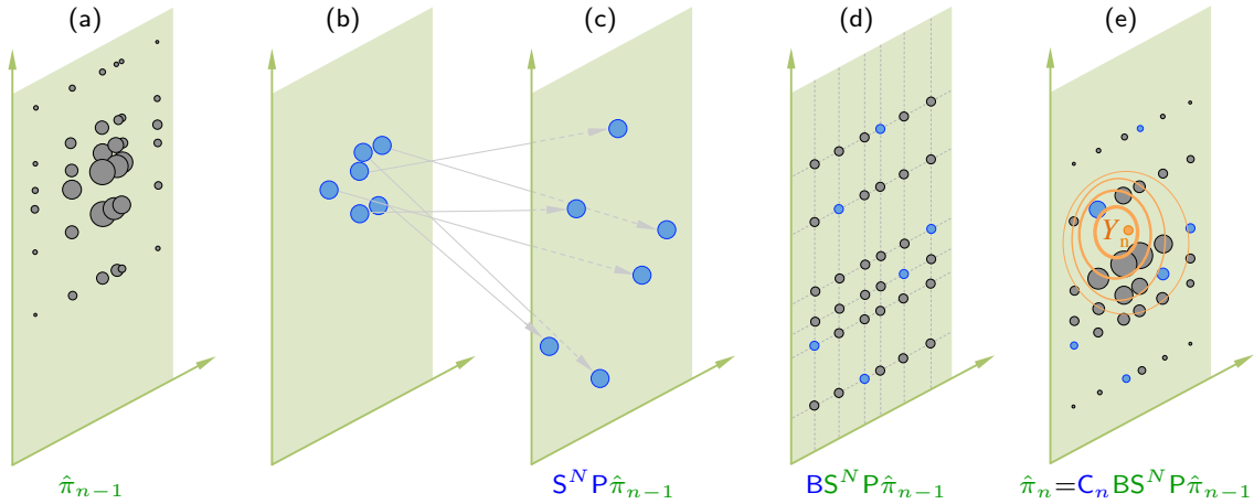
Figure 4.3: Representation of a single iteration of the block particle filter, with \mathbb{X} = \mathbb{Y} = \mathbb{R}_+^2 and N = 6 . Each particle is represented by a ball, whose size is proportional to the weight of the particle. (a) Representation of \hat{\pi}_{n-1} . (b) Resampling step: N particles are sampled independently with replacement and weights are reset to 1/N . (c) Particles are propagated forward using the underlying dynamics. (d) Blocking step: grey balls represent the “ghost” particles that are generated by shuffling the coordinates of the existing N particles (blue balls). (e) Particles are reweighed according to the likelihood of the new observation at time n (whose level sets are drawn in orange) yielding \hat{\pi}_n .
