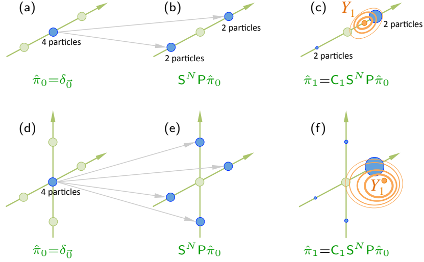
Figure 3.7: Representation of the first iteration of the SIR particle filter applied to the hidden Markov model described in Example 3.9, with N = 4 particles and x = \vec{0} . Pictures (a), (b) and (c) refer for the case d = 1 , while pictures (d), (e) and (f) refer for the case d = 2 . Each particle is represented by a blue ball, whose size is proportional to the weight of the particle, and orange curves represents the level sets of the likelihood function. As symbolically represented, after the first iteration of the algorithm only an average of N/2^d particles have meaningful weights, which is a manifestation of the curse of dimensionality.
