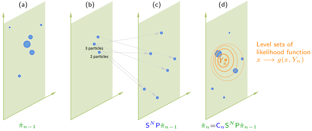
Figure 3.5: Representation of a single iteration of the SIR particle filter with \mathbb{X} = \mathbb{Y} = \mathbb{R}_+^2 and N = 6 . Each particle is represented by a blue ball, whose size is proportional to the weight of the particle. (a) Representation of \hat{\pi}_{n-1} . (b) Resampling step: N particles are sampled independently with replacement and weights are reset to 1/N . If a number m is attached to a particle, then there are m particles sharing the same location. (c) Particles are propagated forward using the underlying dynamics. (d) Particles are reweighed according to the likelihood of the new observation at time n (whose level sets are drawn in orange) yielding \hat{\pi}_n , following the weight recursion (3.4).
