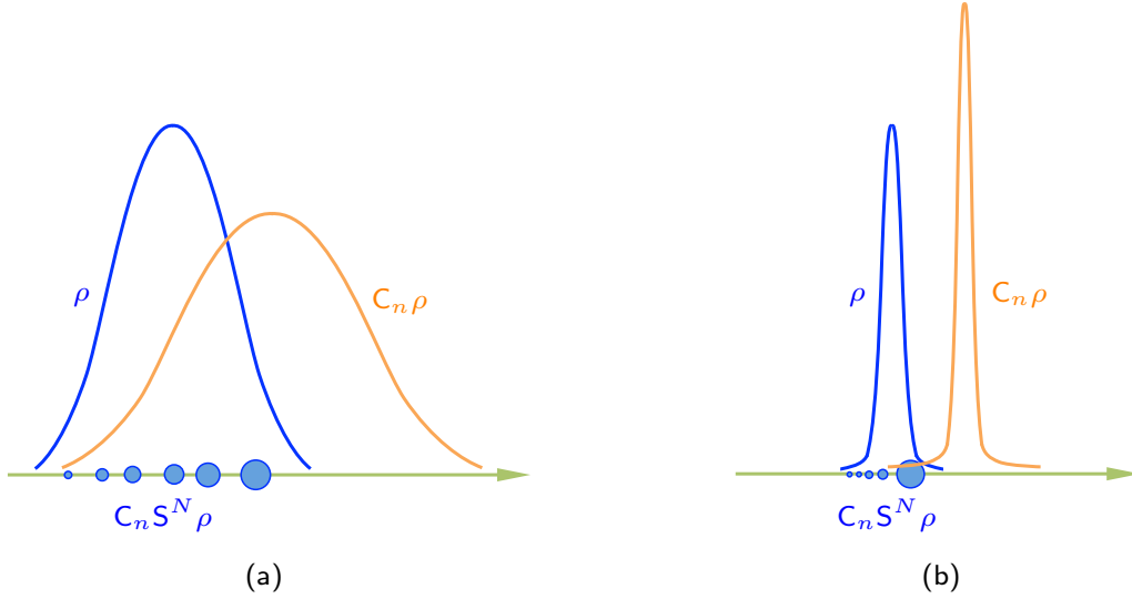
Figure 3.8: Illustration of weights degeneracy with model dimension in a typical iteration of the SIR particle filter. (a) Probability measures in low dimension. (b) Probability measures in high dimension (low-dimensional representation). In high dimension \rho and C_n \rho tend to put mass on different portions of the space. This is the reason why already after a single iteration of the SIR particle filter only a small fraction of samples (in fact, a fraction that is exponentially small in the dimension) is relevant in the algorithm. Each sample X from \rho is represented by a blue ball whose size is proportional to the likelihood g(X, Y_n) , as prescribed by the weights definition (3.4).
