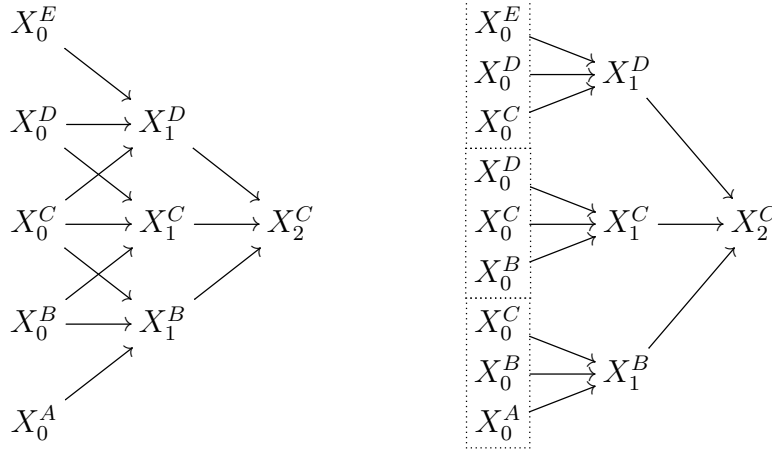
Figure 4.4: For a linear spatial graph G partitioned into blocks A – E (with r = 1 ), the dependencies between the blocks at subsequent times are illustrated here. The left dependency graph represents \mathbf{B}^C \mathbf{P}^2 \mu , the right graph represents \mathbf{B}^C \mathbf{PBP} \mu . The blocking operation unravels the original graph into a tree by introducing independent duplicates (dotted boxes) of blocks in the previous time step.
