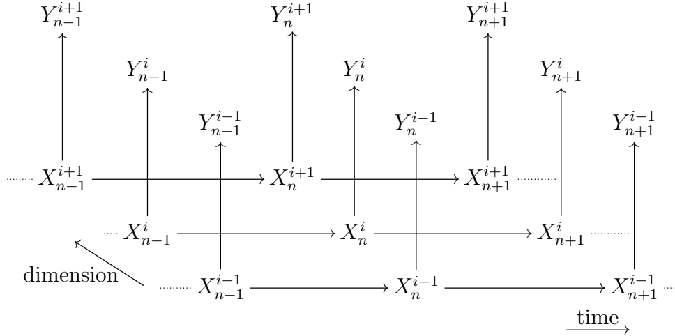
Figure 1.3: Dependency graph of a (trivial) high-dimensional filtering model.
