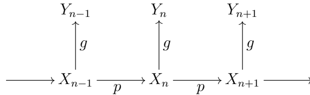
Figure 1.1: Dependency graph of a hidden Markov model.
