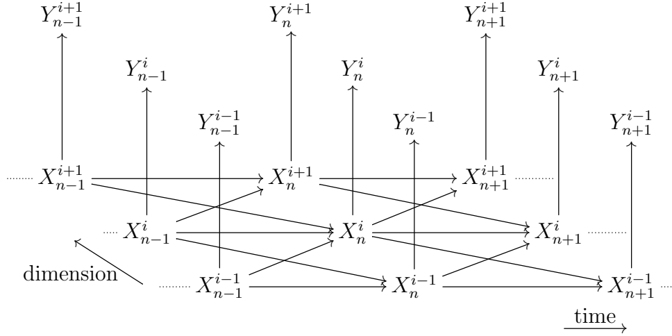
Figure 4.1: Dependency graph of a high-dimensional filtering model of the type considered in this chapter.
