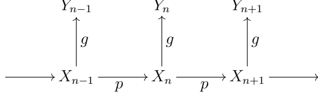
Figure 3.1: Dependency graph of a hidden Markov model.
