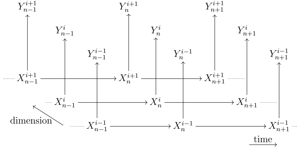
Figure 3.6: Dependency graph of a (trivial) high-dimensional filtering model.
