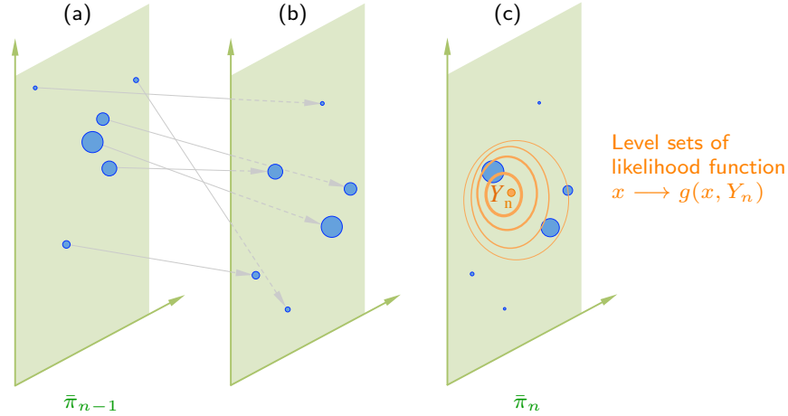
Figure 3.3: Representation of a single iteration of the SIS particle filter in the case when the state and observation spaces are \mathbb{X} = \mathbb{Y} = \mathbb{R}_+^2 , and when there are N = 6 particles considered by the algorithm. Each particle is represented by a blue ball, whose size is proportional to the weight of the particle. (a) Representation of \bar{\pi}_{n-1} . (b) Particles are propagated forward using the underlying dynamics. (c) Particles are reweighted according to the likelihood of the new observation at time n (whose level sets are drawn in orange) yielding \bar{\pi}_n , following the multiplicative weight recursion (3.2).
