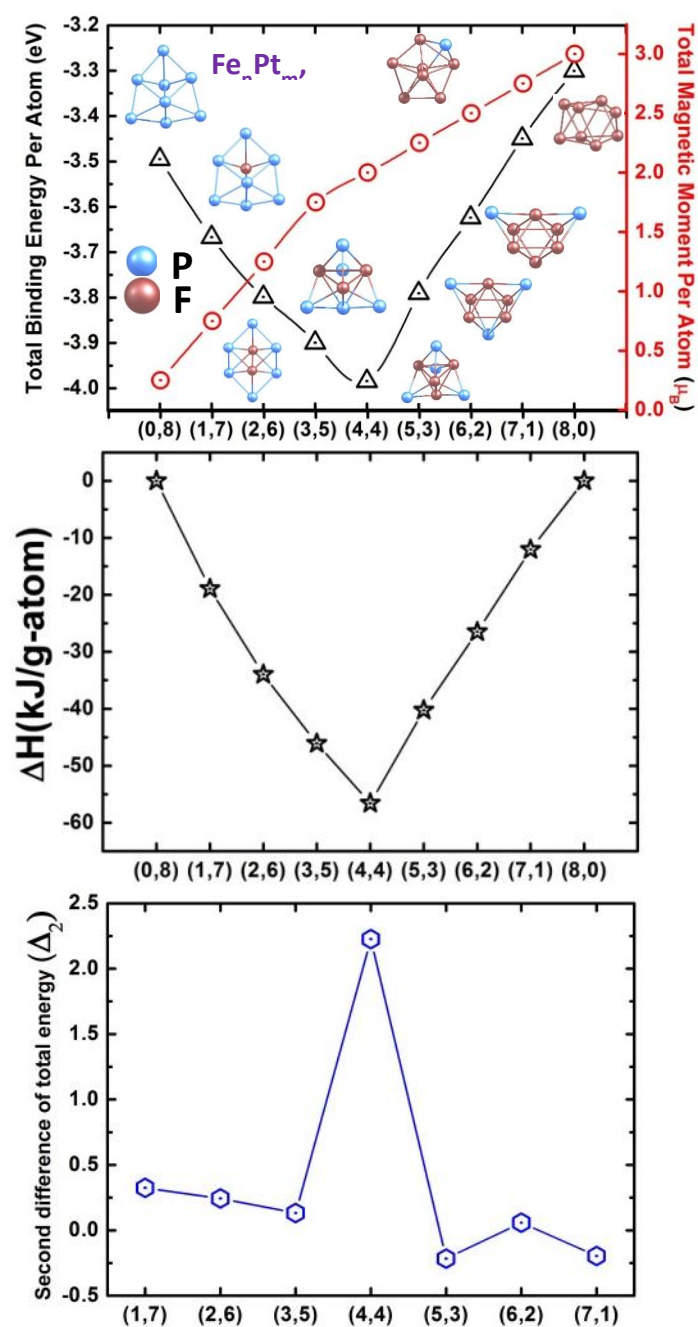
Fig. 2. The total binding energy (eV/atom) along with the total magnetic moment ( \mu_B ) per atom, heat of formation ( \Delta H ), and the second order difference of total energy ( \Delta_2 ) for (\text{Fe}_n\text{Pt}_m) cluster for n + m = 8 .
