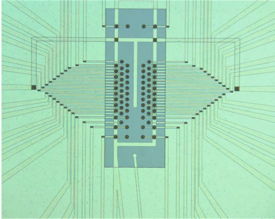
Figure 33: Optical photograph of the interposer wafer after 3rd metal patterning.
