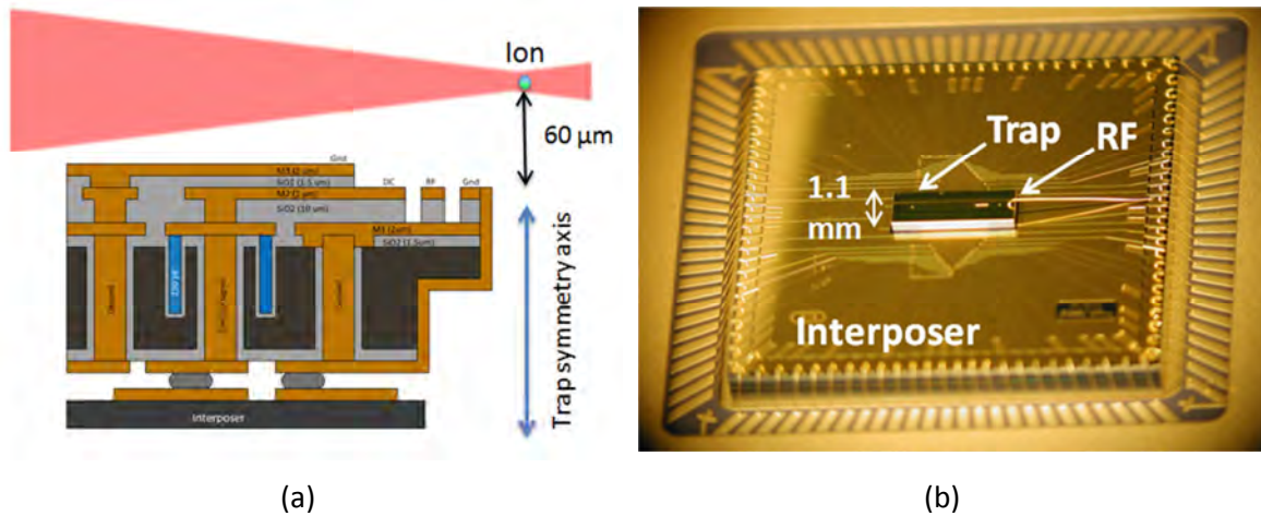
Figure 62: Pictures of SMIT BGA trap – (a) cross-section schematic showing unobstructed beam path to ion, and (b) picture of actual BGA trap.
