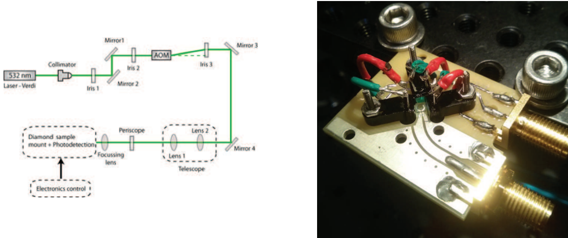
Fig. 1: Left: Schematics of the optical setup. Right: the light collection board, showing three photodetectors (black boxes) surrounding the diamond and connected with red/green cables to the PCB board.
