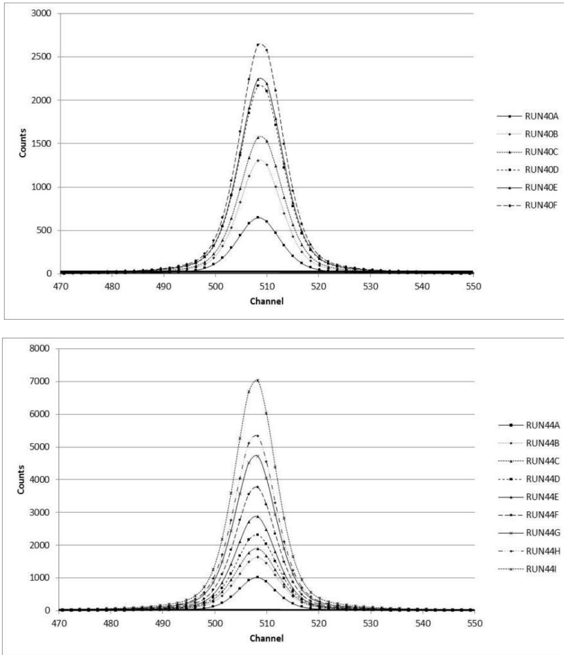
Figure 31: Peak Development for In-Experiment Runs. Peaks are the Voigt fit to the data. Top: Run40A-F. Bottom: Run44A-I.
