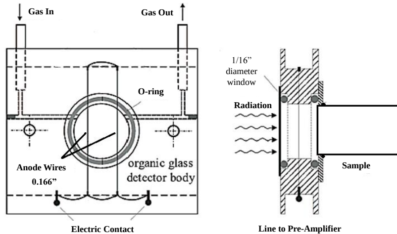
Figure 14: Simple diagram of the SD200: a gas-flow proportional detector for CEMS.
