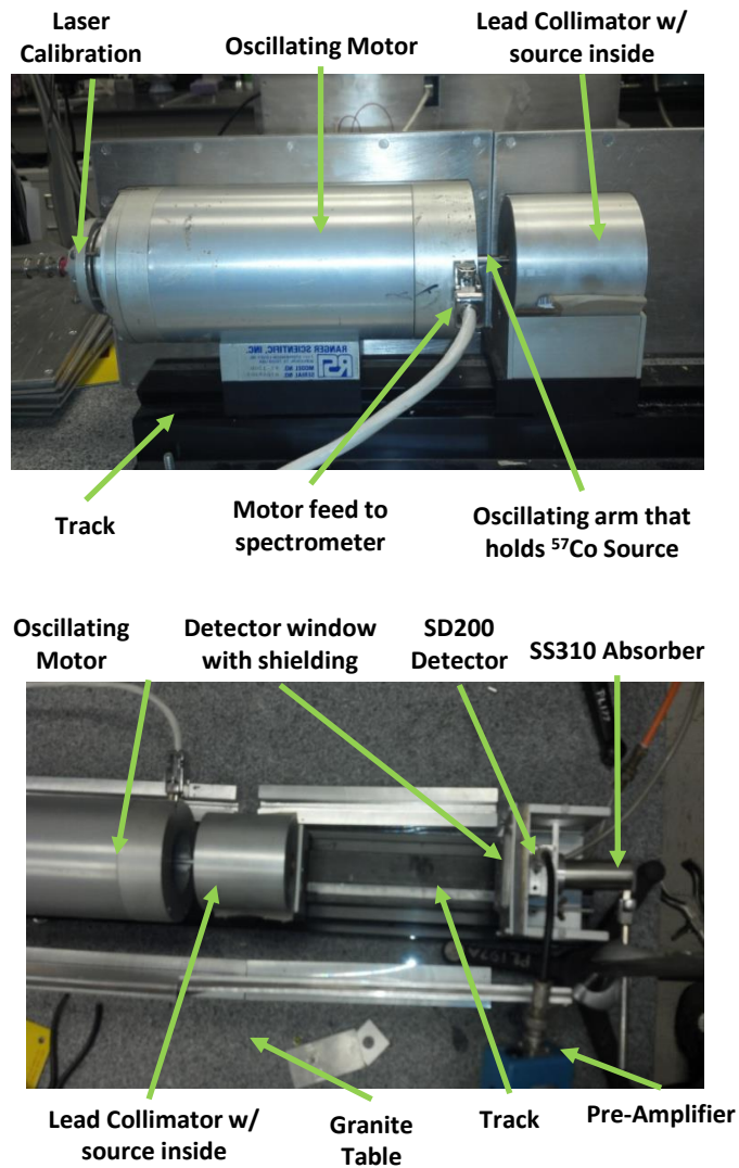
Figure 20: Top: Image of the oscillating motor, laser calibration, ^{57}\text{Co} source location and lead collimator. Bottom: Source orientation from detector window, SD200 detector and SS310 absorber rod.
