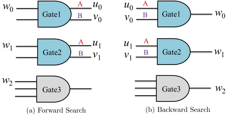
Figure 2.6: Structural Heuristics for Finding Target Words from Source Word \vec{w} . Gates of different function types are colored differently.
