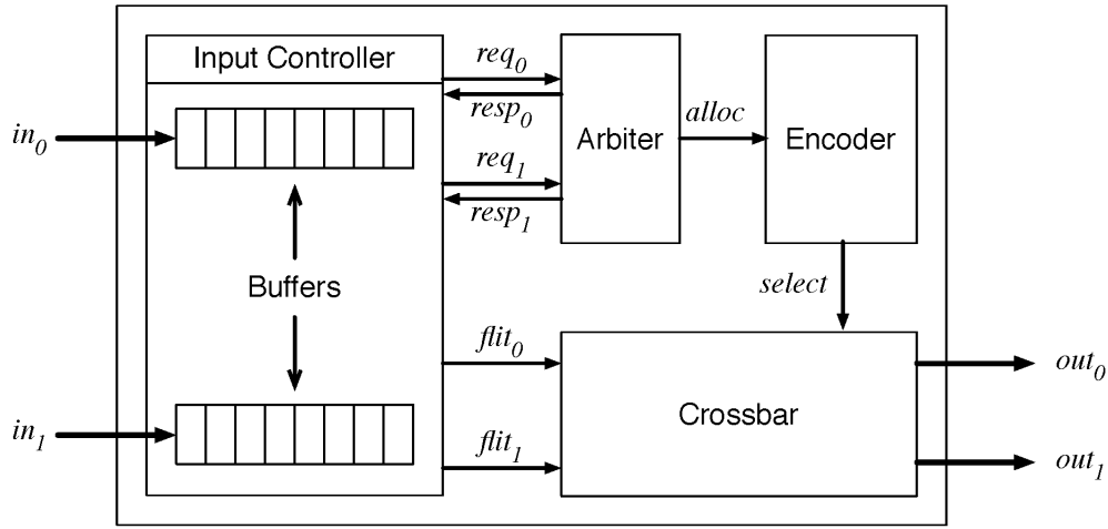
Figure 2.13: CMP Router Comprising Four High-Level Modules
