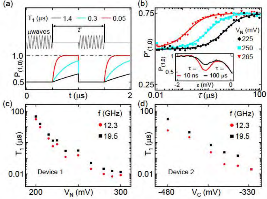
Figure 4.12: (a) Pulse sequence used to measure T_1 and simulated qubit response. P_{(1,0)} = 0.5 when resonant microwaves drive transitions between (0,1)_g and (1,0)_g , and approaches 1 on a timescale set by T_1 when the microwaves are turned off. (b) P_{(1,0)}^* as a function of \tau extracted for different V_N at f = 19.5 GHz. Fits to the data give T_1 = 1.4 \mu s, 0.3 \mu s and 0.05 \mu s for V_N = 225 mV, 250 mV and 265 mV. (Inset) Comparison of typical PAT peaks at different \tau , with fixed V_N = 225 mV and f = 25.9 GHz. (c) T_1 as a function of V_N in device 1. (d) T_1 as a function of V_C in device 2. In both devices, T_1 increases as the interdot barrier is made less transparent.
