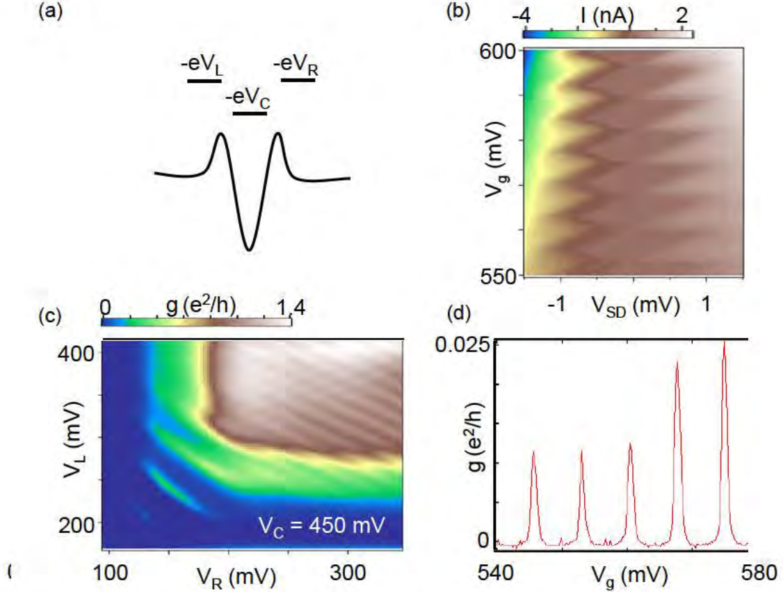
Figure 5.5: (a) Schematic diagram showing the confinement potential of the device. The dot is accumulated locally using a single gate V_C , where the lead-dot barriers are controlled by two plunger gate voltages V_L and V_R . (b) Coulomb diamond measured in current as a function of gate voltage V_g and source-drain bias voltage. (c) Measured conductance as a function of plunger gate voltages V_L and V_R , in a device with similar gate geometry as in Figure 5.4. (d) 1D conductance measurement as a function of V_g , demonstrating typical Coulomb blockade peaks.
