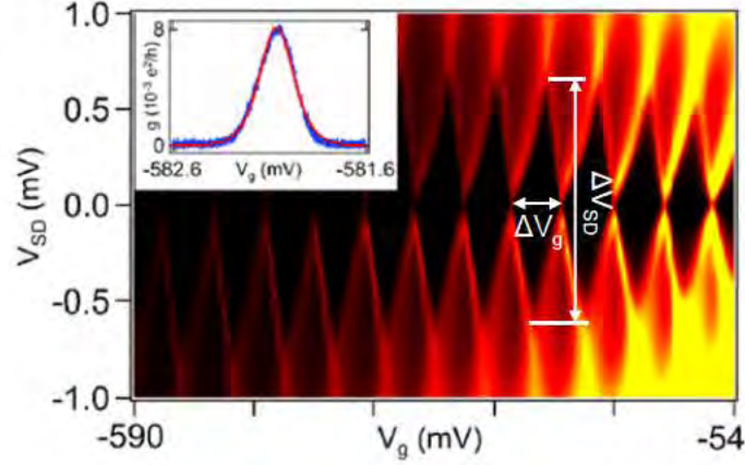
Figure 3.6: Colorscale plot of QD conductance, g , as a function of V_g and V_{SD} . Clear Coulomb diamonds are observed when the device is configured as a single dot. Inset: Conductance as a function of V_g for V_{SD} = 0 .
