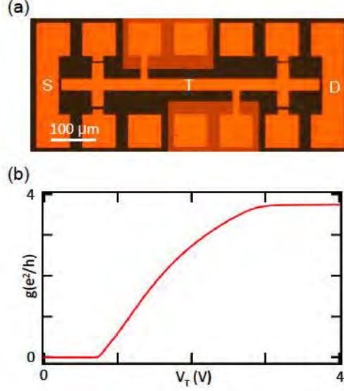
Figure 4.2: (a) Optical image of a typical accumulation-mode Hall bar device. Main contacts are labeled as S (source), D (drain) and T (top gate). (b) Conductance g as a function of top gate voltage V_T . The 2DEG turns on at V_T = 800 \text{ mV} and saturates at V_T = 3000 \text{ mV} .
