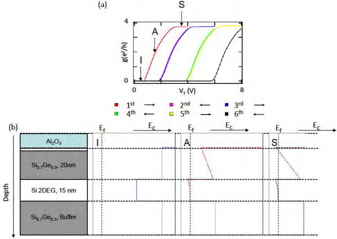
Figure 4.4: (a) Six consecutive measurements of the longitudinal conductance g as a function of top gate voltage V_T . The arrows denote different stages of the device operation, namely the isolation stage (I), the accumulation stage (A) and the saturation stage (S). (b) Simulated band diagrams of the heterostructure in each of the three conductance stages, showing the conduction band minimum as a function of depth.
