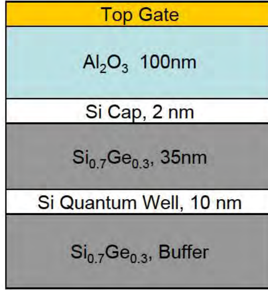
Figure 4.1: Profile of a typical undoped Si/SiGe heterostructure. Doping layer and dopants are absent in the heterostructure. Instead, the 2DEG is accumulated by applying positive voltages to the global top gate.
