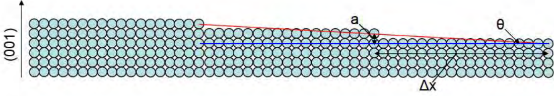
Figure 5.3: Schematic of lattice miscut in Si/SiGe heterostructure. The blue line corresponds to the lattice plane perpendicular to (001) direction, while the red line corresponds to the cut direction of Si substrate. The resulting atomic steps are separated by \Delta x = \frac{a}{\tan \theta} , in which a \approx 0.357 nm is the lattice constant of Si and \theta is the lattice miscut angle.
