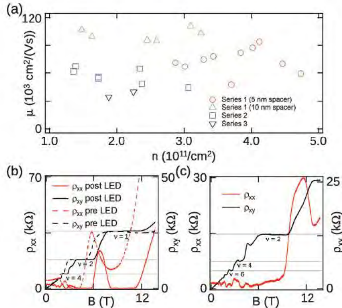
FIG. 2. (Color online) (a) Carrier mobility plotted as a function of charge density for each wafer series. (b) Hall data sets recorded before and after illumination with a LED for a series 2 wafer with a doping level of 3 \times 10^{18}/\text{cm}^3 , resulting in \mu = 36,000 \text{ cm}^2/\text{Vs} and n = 1.8 \times 10^{11}/\text{cm}^2 after illumination and \mu = 49,000 \text{ cm}^2/\text{Vs} and n = 2.4 \times 10^{11}/\text{cm}^2 after illumination. (c) A series 1 wafer (5 nm spacer) with a doping level of 6 \times 10^{17}/\text{cm}^3 does not show clear zeros in \rho_{xx} after illumination with a LED. \mu = 48,000 \text{ cm}^2/\text{Vs} and n = 3.7 \times 10^{11}/\text{cm}^2 after illumination.
