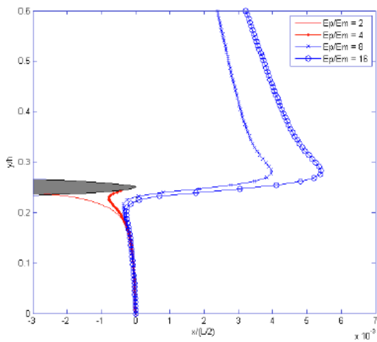
Figure 4. Crack extension near an auxetic particle, \nu_p/\nu_m = -1 .
