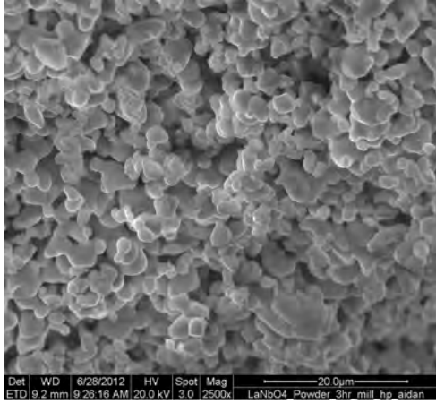
Figure 9. Scanning electron micrograph of \text{LaNbO}_4 powder made by mixing for 3 h and calcining at 1200\text{ }^\circ\text{C} for 14 h.
