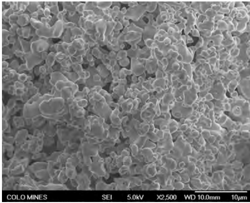
Figure 10. Scanning electron micrograph of \text{LaNbO}_4 powder made by mixing for 10 h and calcining at 1200\text{ }^\circ\text{C} for 14 h.
