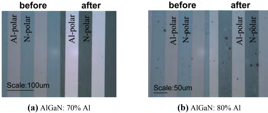
FIG. 40: Microscope images of AlGa 1-x N LPS before and after KOH etching determination of polarity. (a) Al x Ga 1-x N LPS grown with 0.7 Al content. (b) Al x Ga 1-x N LPS grown with 0.8 Al content.
