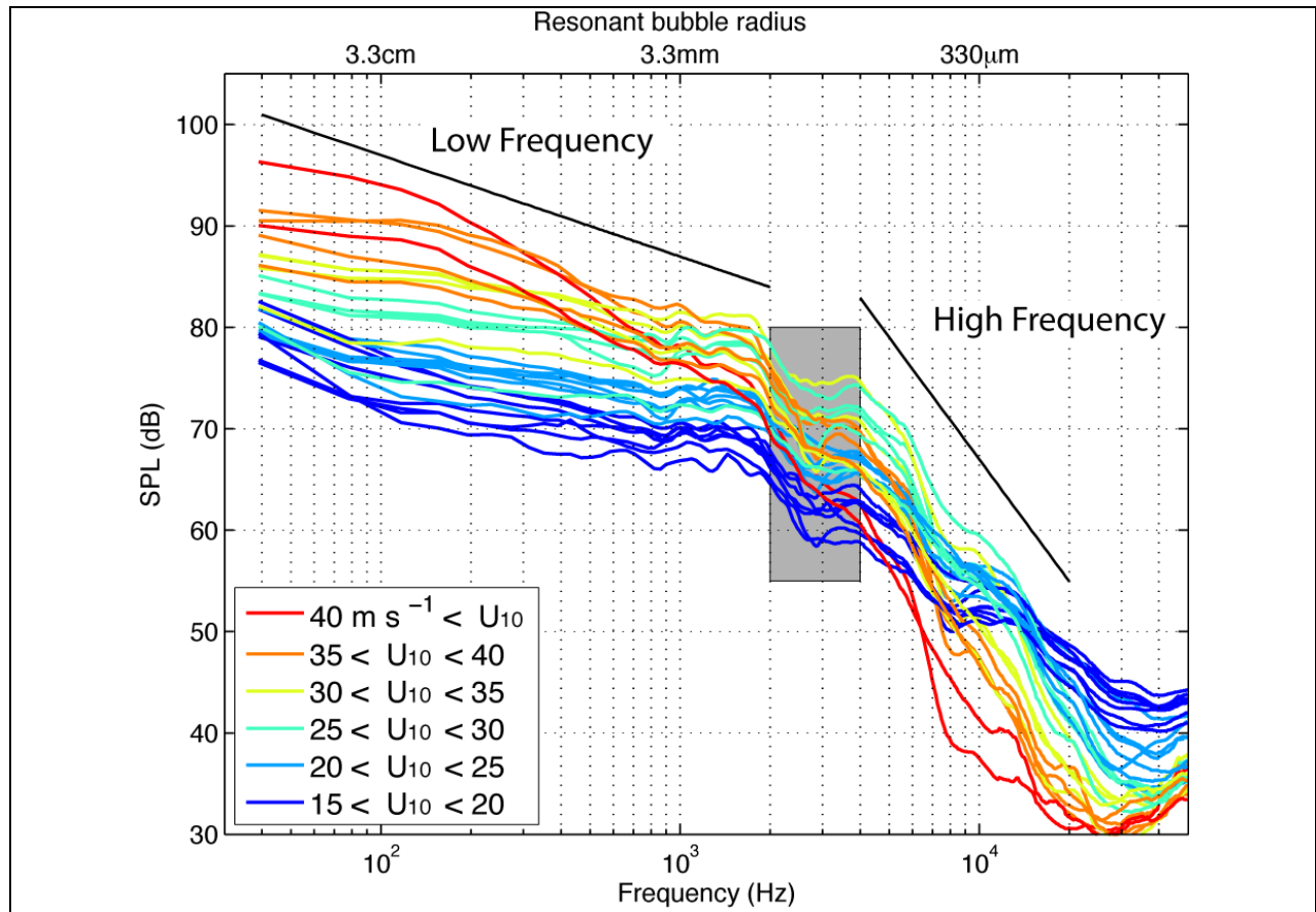
Figure 3. Sound spectra within selected wind speed categories. At all wind speeds, a clear break in spectral slope occurs near 3 kHz, corresponding to a bubble size of approximately 1mm.
