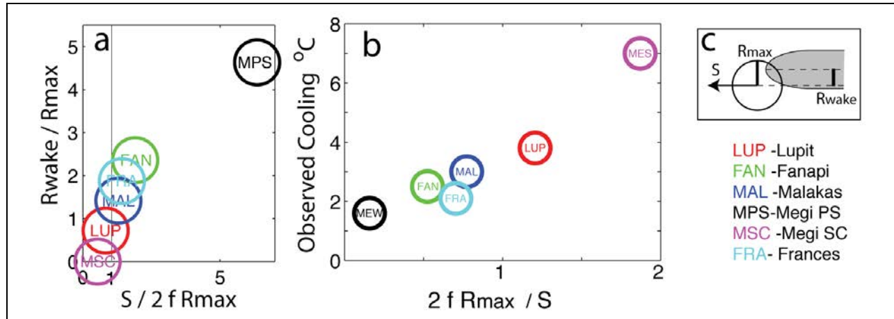
Figure 1. Variation of cold wake properties with the non-dimensional storm speed for 6 ITOP/CBLAST storms. a) The position of the cold wake moves away from the storm track with increasing storm speed. b) The amount of cooling decreases. Thus a slow storm has strong cooling along the track while a weak one has weak cooling to the right of the track. c) This sketch shows defines the wake and storm geometry.
