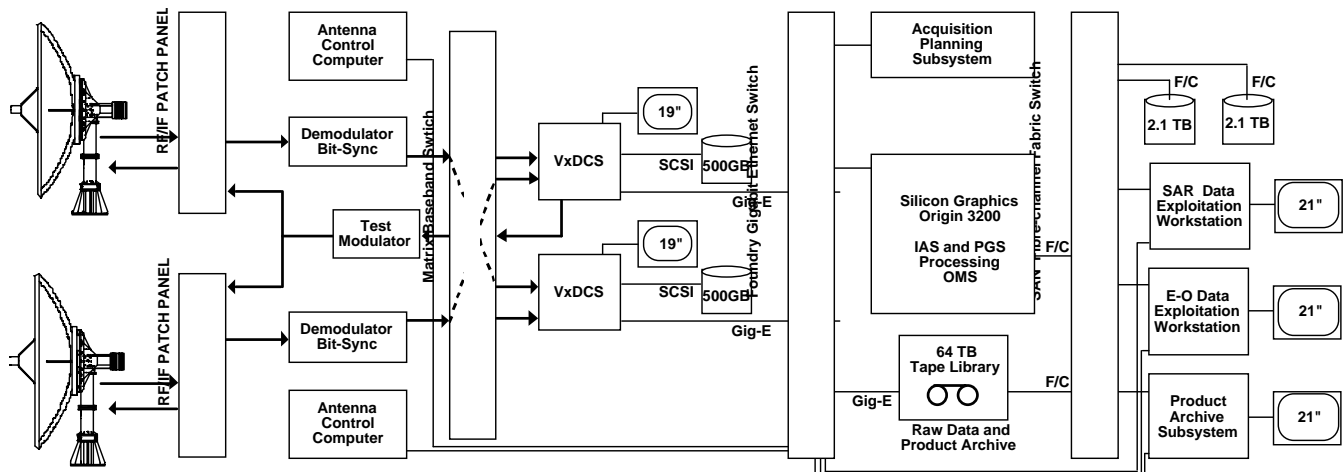
Figure 1: Block diagram of basic system for CSTARTS facility.
