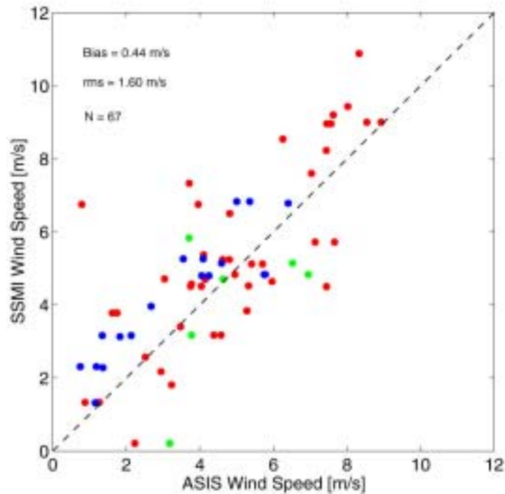
Figure 3: Scatterplot of ASIS and SSM/I wind speeds.
