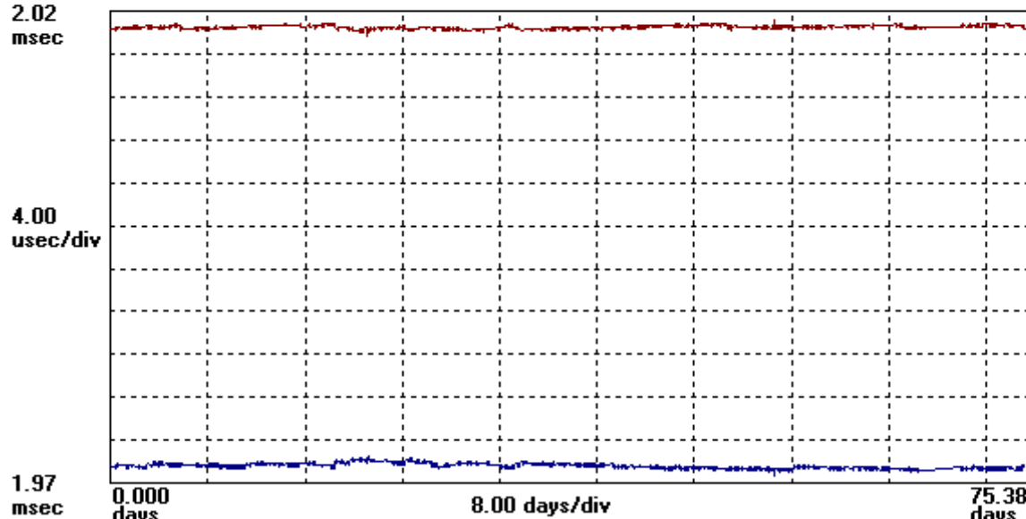
Figure 1: PTP over SONET results over 75 days, showing the forward delay in blue and the reverse in red. The total delay is about 2 ms with about a 40 \mu s asymmetry.
