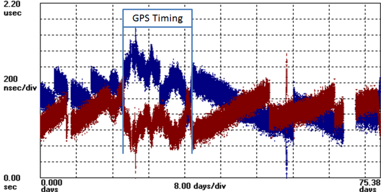
Figure 2: Data as in Figure 1 with the minimum offset of each plot set to 0.0 to show the deviations. For most of this period nodes were timed by Cs clocks, showing a slope of about 50 ns/d with occasional resets of about 300 ns. A period in the middle is marked where GPS timing was used. Here, the system accumulated wander with no apparent systematic behavior.
