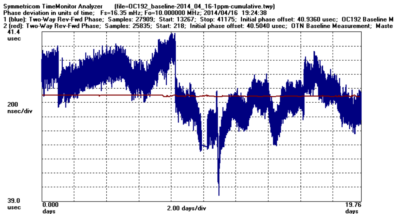
Figure 6: The asymmetry from the reverse minus forward directions for the SONET-based circuit (blue) and the OTN-based circuit (red) plotted on the same graph. The two systems have a very similar average asymmetry.
