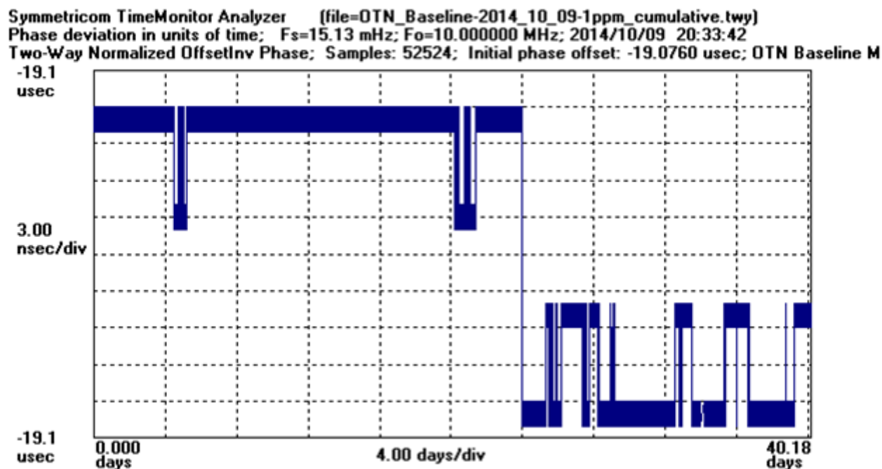
Figure 5: Time transfer capability using the OTN. The value of -19.1 \mu s is due to an asymmetry of 38.2 \mu s. The peak-to-peak deviation is 26 ns, with the short term no more than 4 ns.
