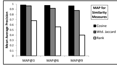
Figure 3: [Mean Average Precision (MAP).] Cosine similarity outperforms alternative approaches.
