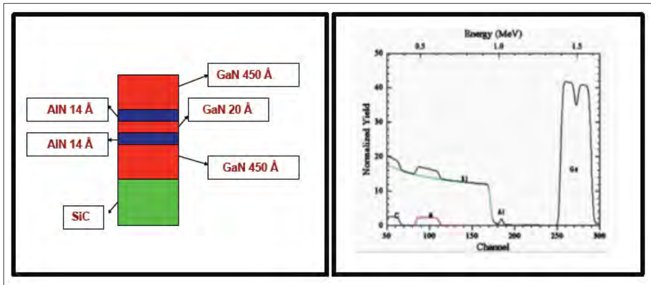
Figure 36: RBS simulation of the RTD structure shown on the left.
