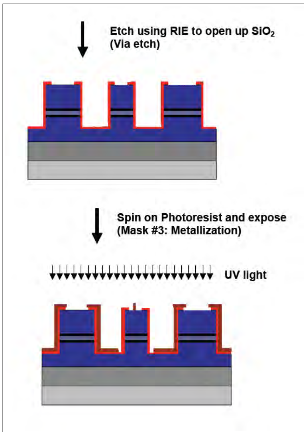
Figure 48: Top: RIE etch used to open the SiO 2 layer over the junction (CF 4 chemistry). Bottom: Lithography is used to define the metal contacts (Mask 3 – Lift off).
