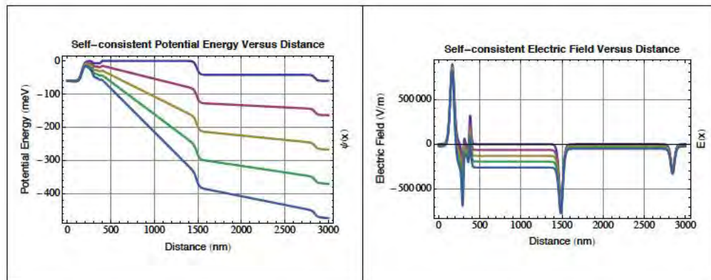
Figure 29: (a) Self-consistent potential energy variation as a function of distance, for different values of applied bias. (b) The self consistent electric field as obtained from the potential energy variation.
