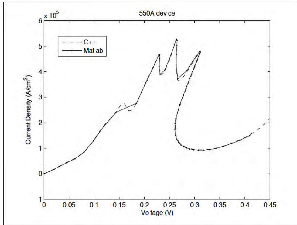
Figure 79: Comparison of IV curves from the Matlab code and the C++ code. The slight differences between the curves in each figure are attributable to more restrictive parameter settings in the C++ code.
