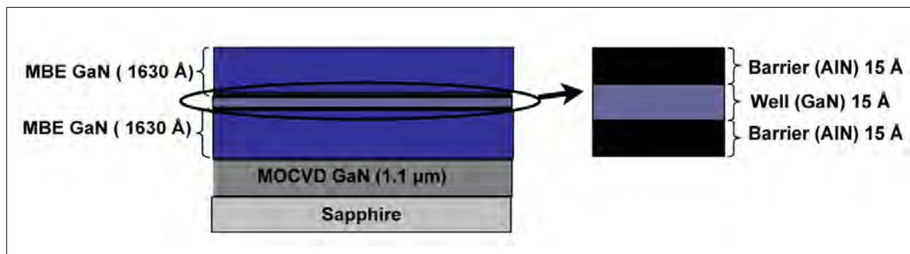
Figure 45: Color coded schematic of the structure prepared for processing.
