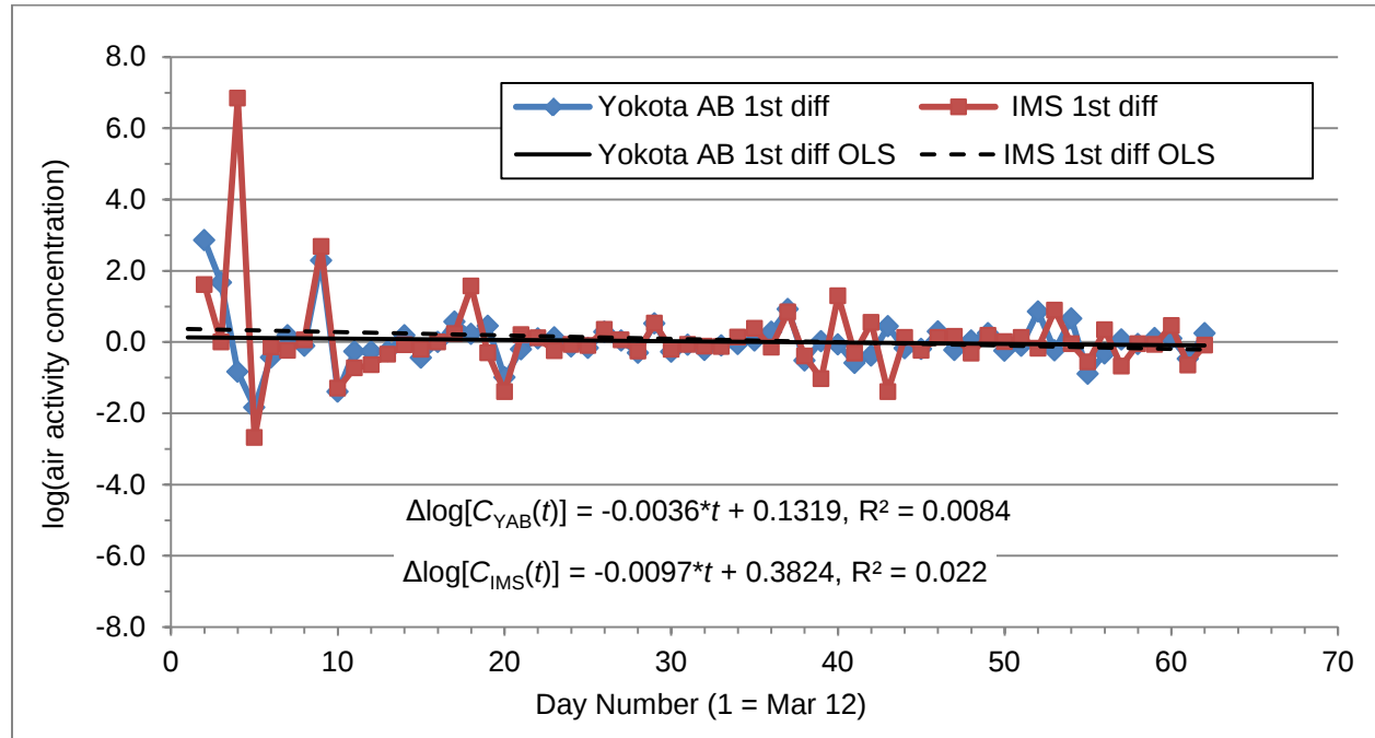
Figure 7. First differences in logarithmic values of air activity concentrations of Cs-134 for Yokota AB and IMS-Takasaki
