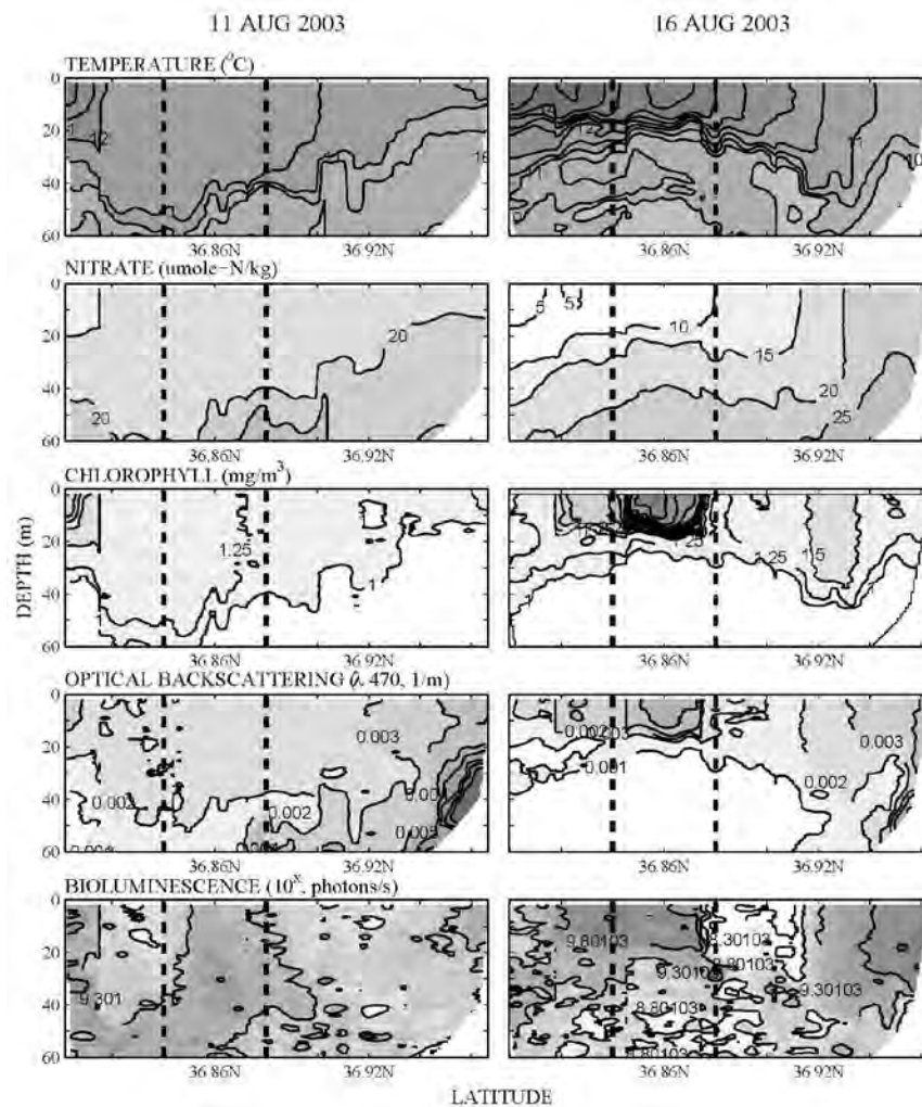
Figure 5. AUV DORADO surveys taken 11 and 16 August 2003. Vertical dashed lines indicate location of the high chlorophyll a filament: 11 August - where the filament appeared later on MODIS-Aqua image on 15 August; 16 August - where the filament observed in MODIS-Aqua image on 15 August.
