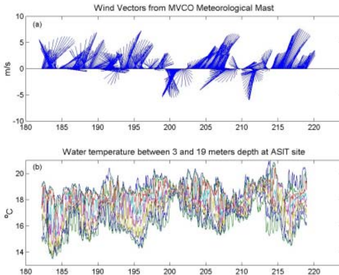
Figure 2. Timeseries of velocity vectors (a) and temperature profiles (b) from the 2001 Pilot Experiment. The velocity measurements are taken from the MVCO meteorological mast shown in Figure 1, while the temperature measurements were deployed beneath a guard buoy located at the proposed ASIT site.
