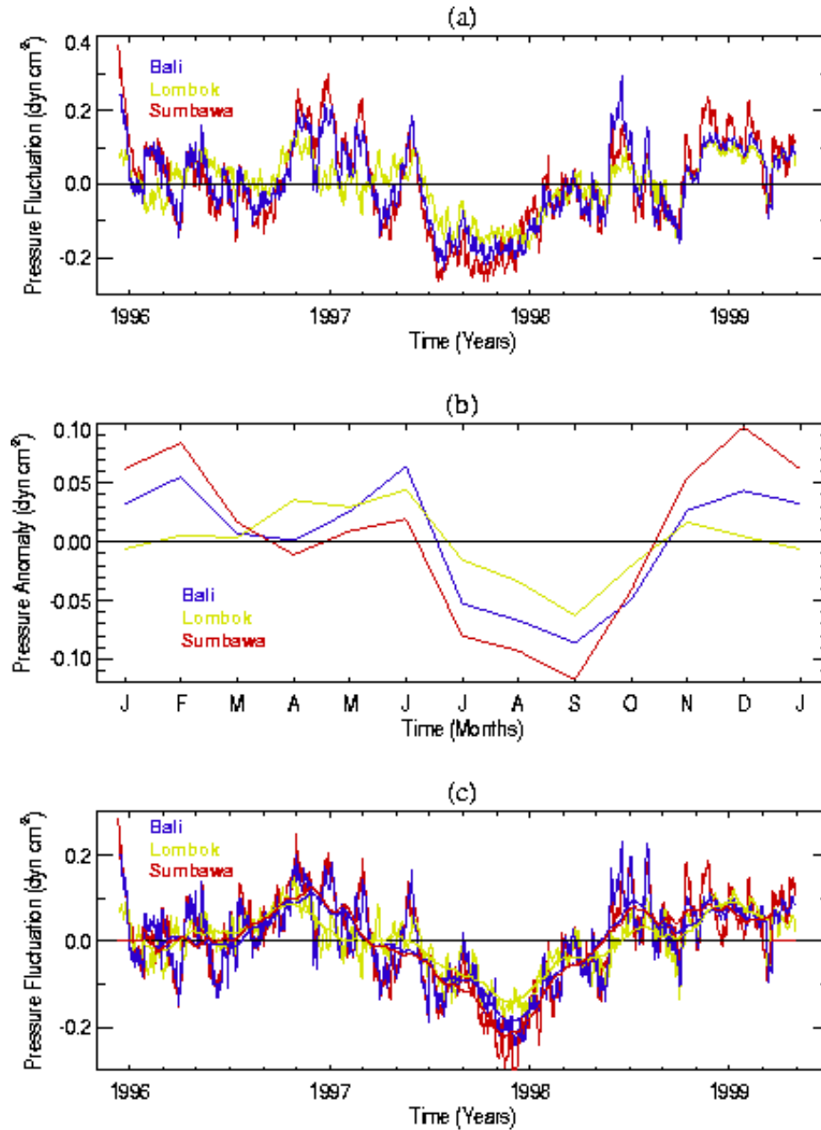
Fig. 1 The near-surface pressure fluctuations at the Bali, Lombok and Sumbawa pressure gauges. The signals at the Bali and Sumbawa gauges have similar amplitude and phase at all sub-inertial frequencies. This indicates that they lie on the same shelf in a dynamical sense – the Bali gauge was indeed located just to the south of the headland at Mt. Seraya – but importantly not necessarily the same wave amplitude. The Lombok gauge signal is quite different implying that it is dynamically isolated from these two gauges – it was ‘hidden’ behind the Gilli Islands. The daily averaged values are plotted in (a) with the mean and linear trend removed. The monthly averaged values for the 3.3 year time series are plotted in (b), and the resulting anomalies are plotted in (c) along with 90-day running means for each gauge.
