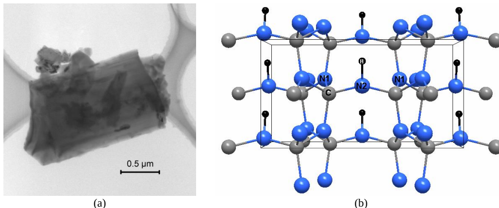
Fig. 2.14 a) Bright field TEM image of the C_2N_2(NH) crystal synthesized at P = 41 \text{ GPa} and T > 1700^\circ\text{C} and b) crystal structure of the defect wurtzite-type carbon nitride imide, dwur- C_2N_2(NH) 171
