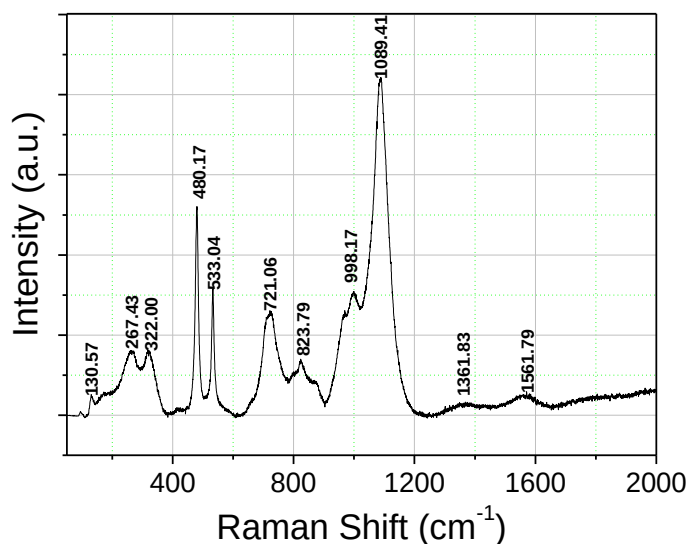
Fig. 1.4 Raman spectrum of 8' (at 2,000\text{ }^{\circ}\text{C} )
